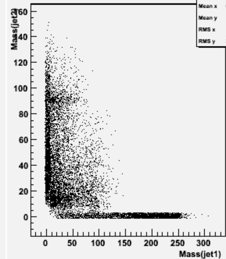
Jet mass for forced 2-jets : w102086 n3n3cce1e1_o
