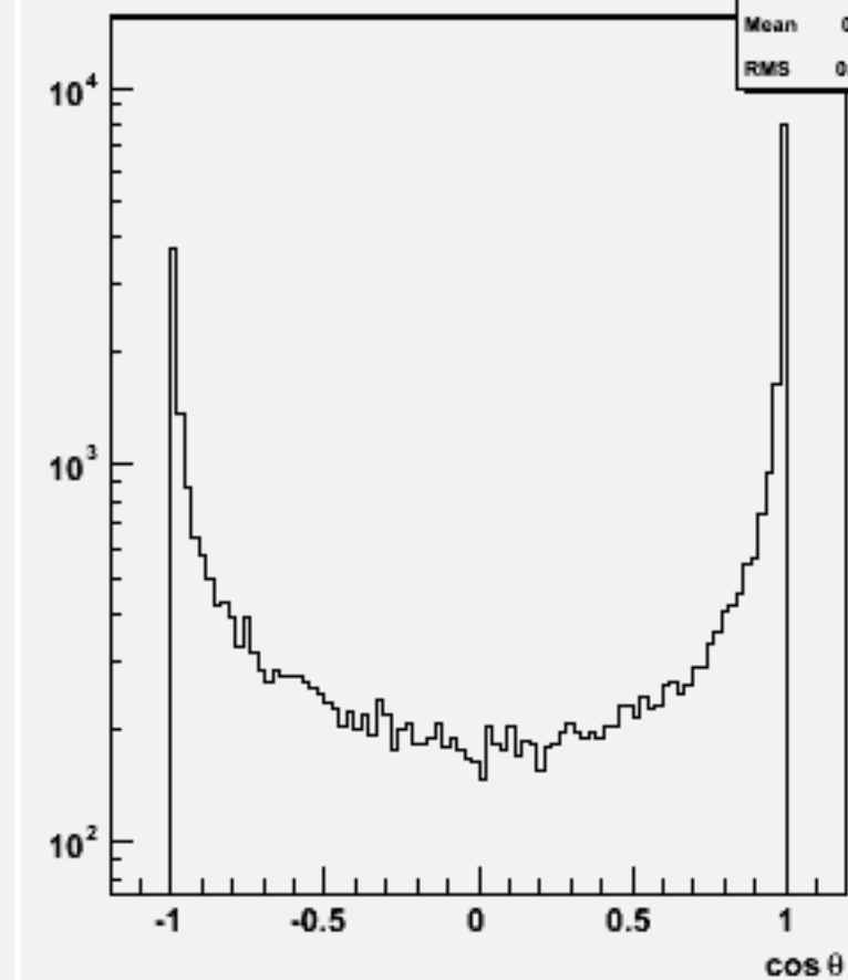
Jet cos \theta (All jets)w102086 n3n3cce1e1_o
