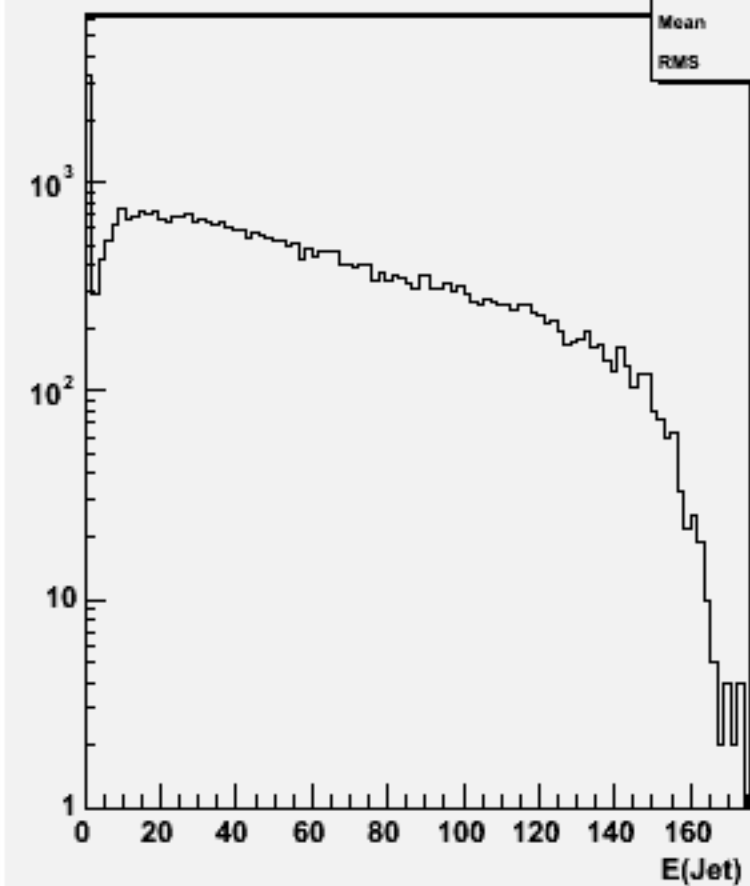
Jet energies(All jets)w102086 n3n3cce1e1_o
