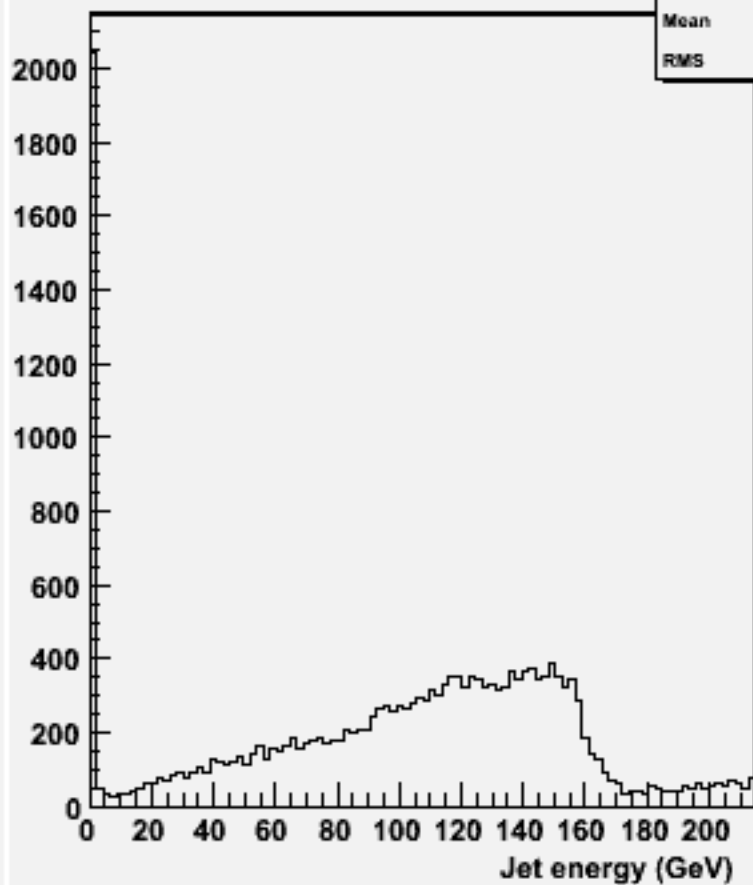
energy for 2-jets :w102086 n3n3cce1e1_o
