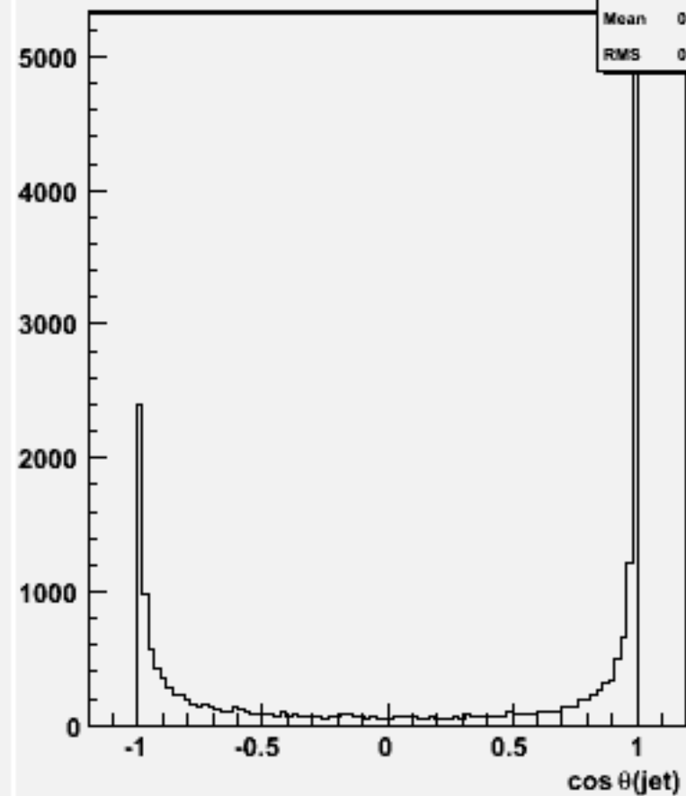
cos \theta for 2-jets :w102086 n3n3cce1e1_o
