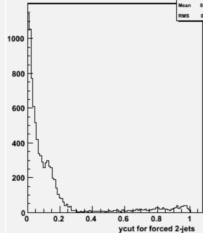
Ycut for 2-jets :w102086 n3n3cce1e1_o
