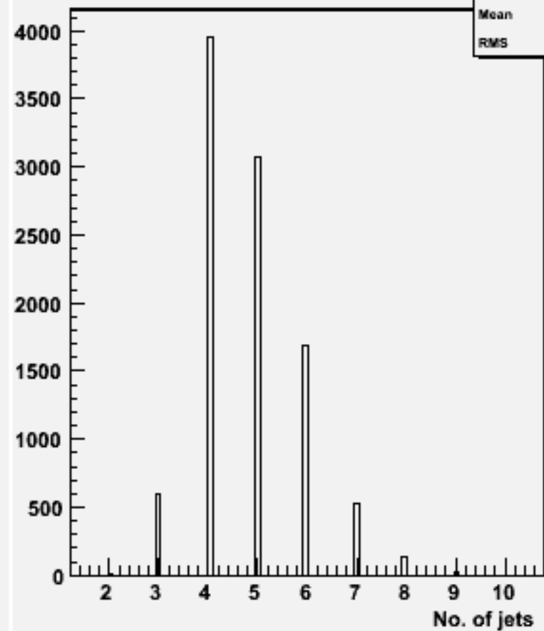
No. jets (ycut=0.001) : w102086 n3n3cce1e1_o
