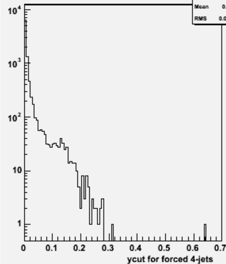
Ycut for 4-jets :w102086 n3n3cce1e1_o
