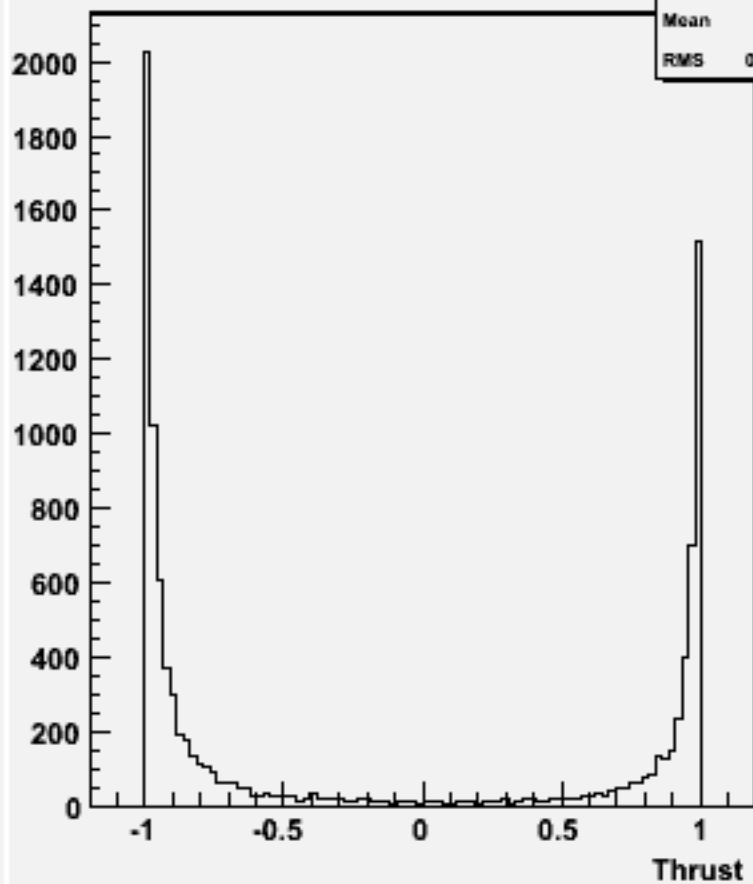
cos \Theta (thrust) w102086 n3n3cce1e1_o
