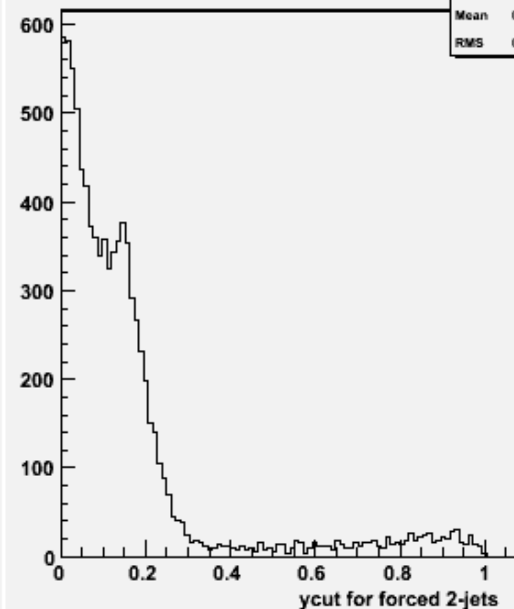
Ycut for 2-jets :w102084 n3n3cce1e1_o
