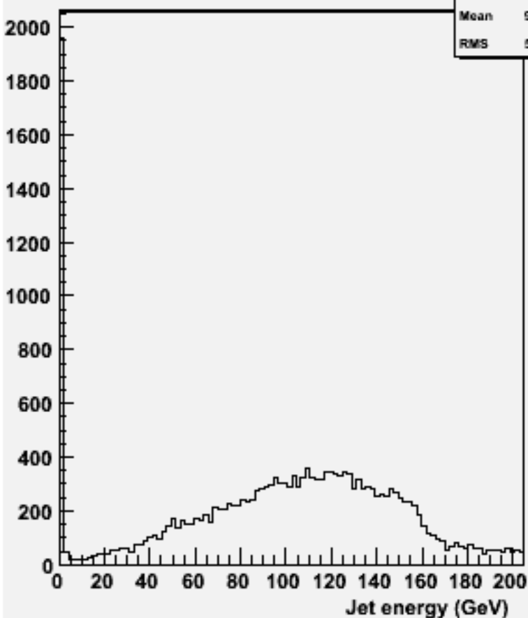
energy for 2-jets :w102084 n3n3cce1e1_o
