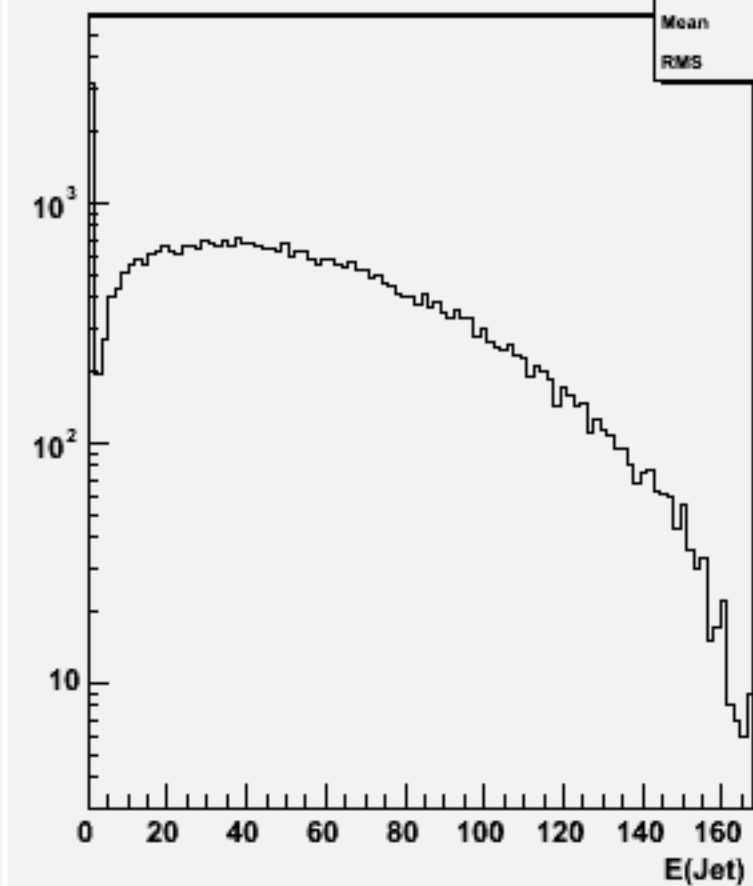
Jet energies(All jets)w102084 n3n3cce1e1_o
