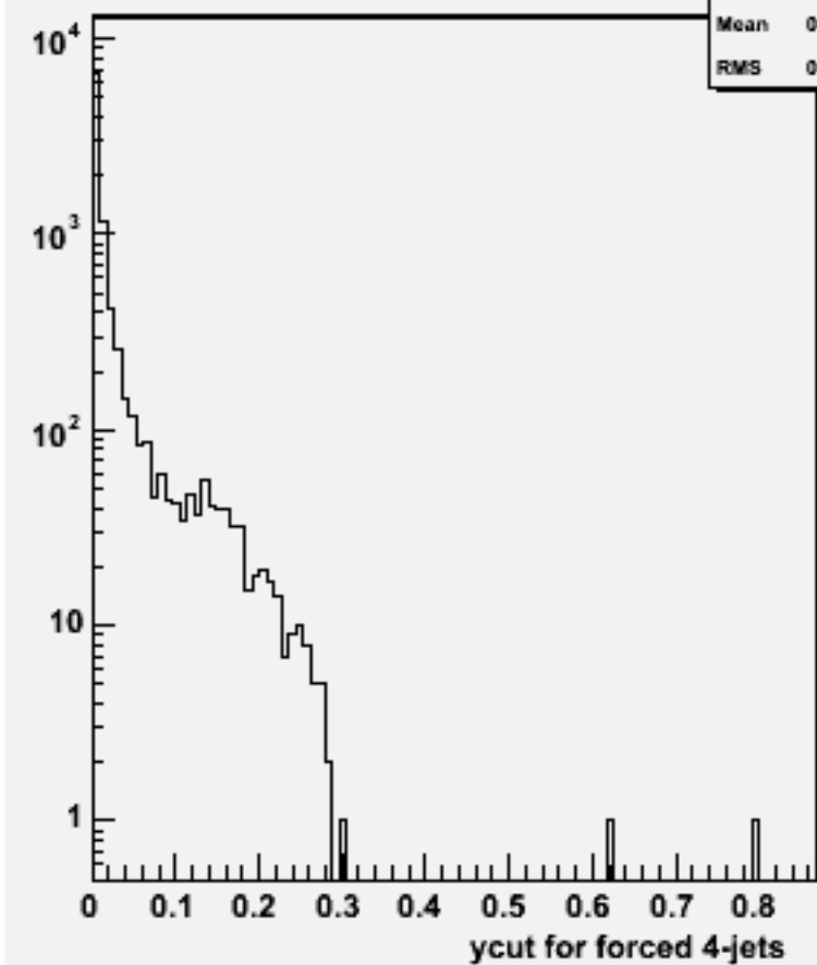
Ycut for 4-jets :w102084 n3n3cce1e1_o
