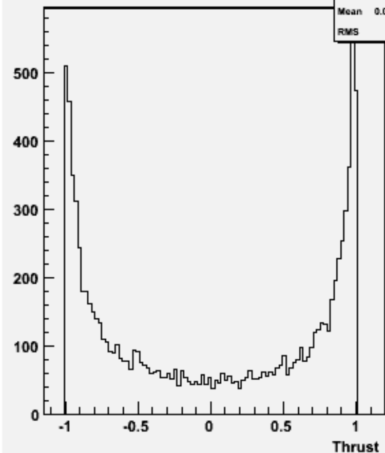
cos \Theta (thrust) w102084 n3n3cce1e1_o
