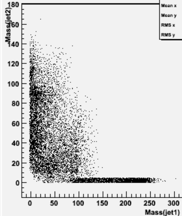
Jet mass for forced 2-jets : w102084 n3n3cce1e1_o
