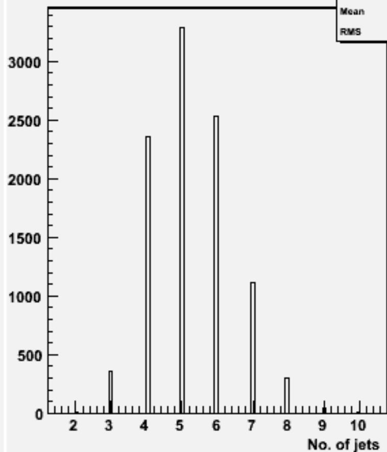
No. jets (ycut=0.001) : w102084 n3n3cce1e1_o
