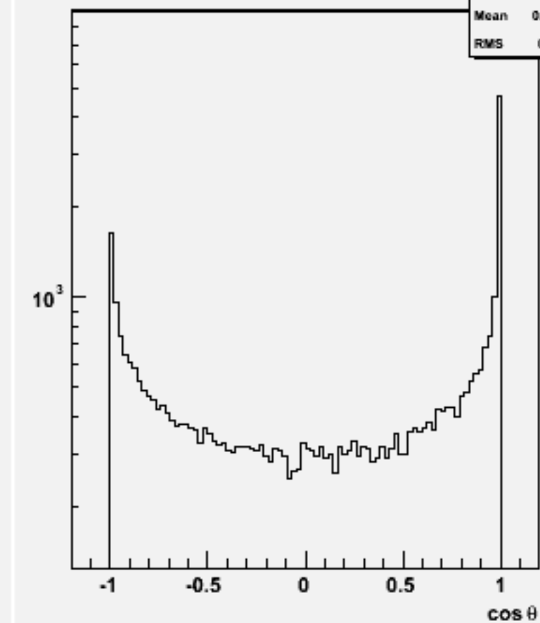
Jet cos \theta (All jets)w102084 n3n3cce1e1_o
