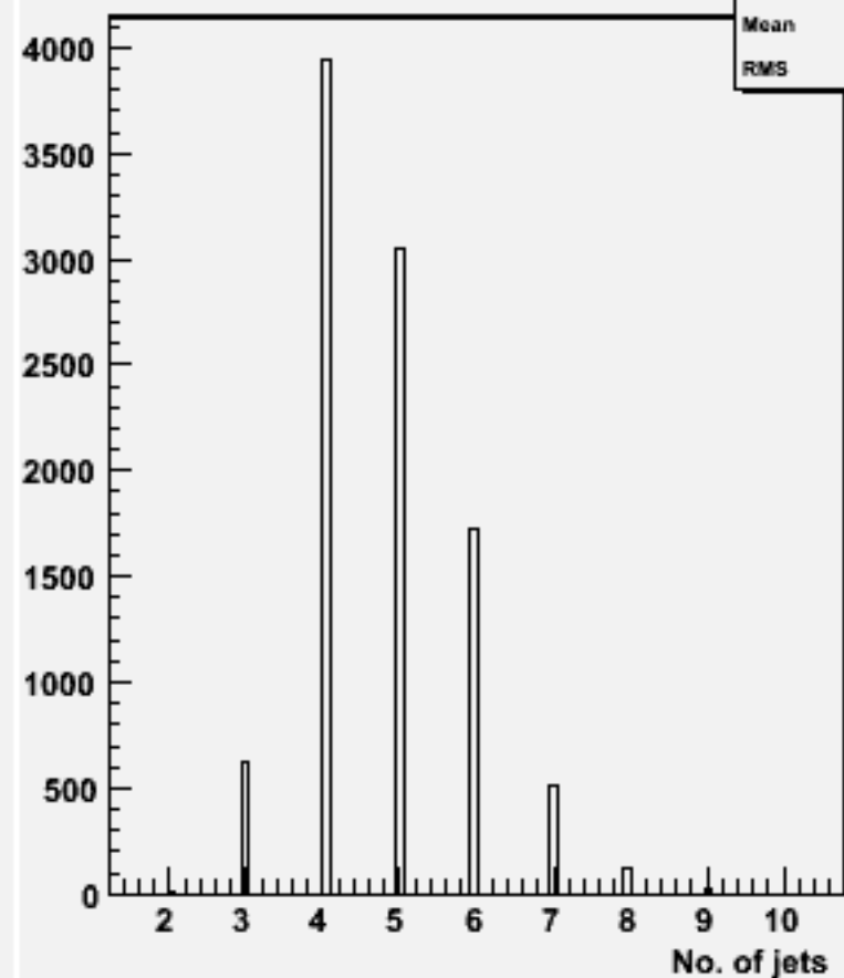
No. jets (ycut=0.001) : w102083 n3n3cce1e1_o
