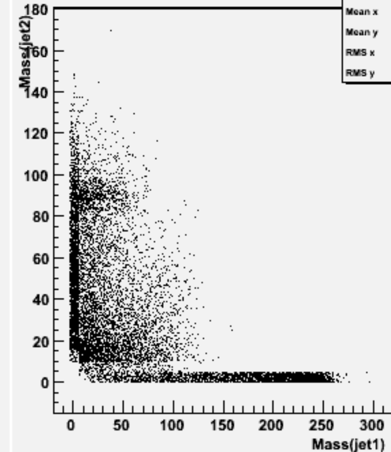
Jet mass for forced 2-jets : w102083 n3n3cce1e1_o
