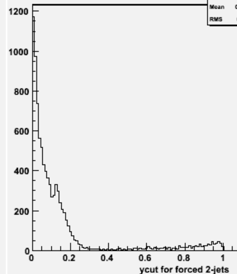
Ycut for 2-jets :w102083 n3n3cce1e1_o
