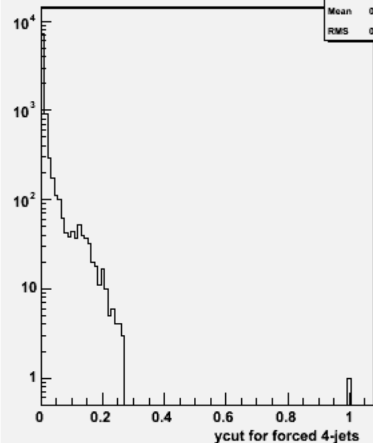
Ycut for 4-jets :w102083 n3n3cce1e1_o
