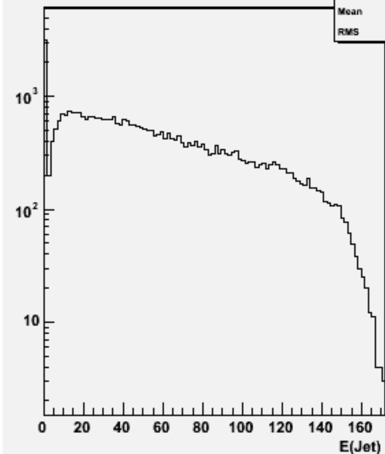
Jet energies(All jets)w102083 n3n3cce1e1_o
