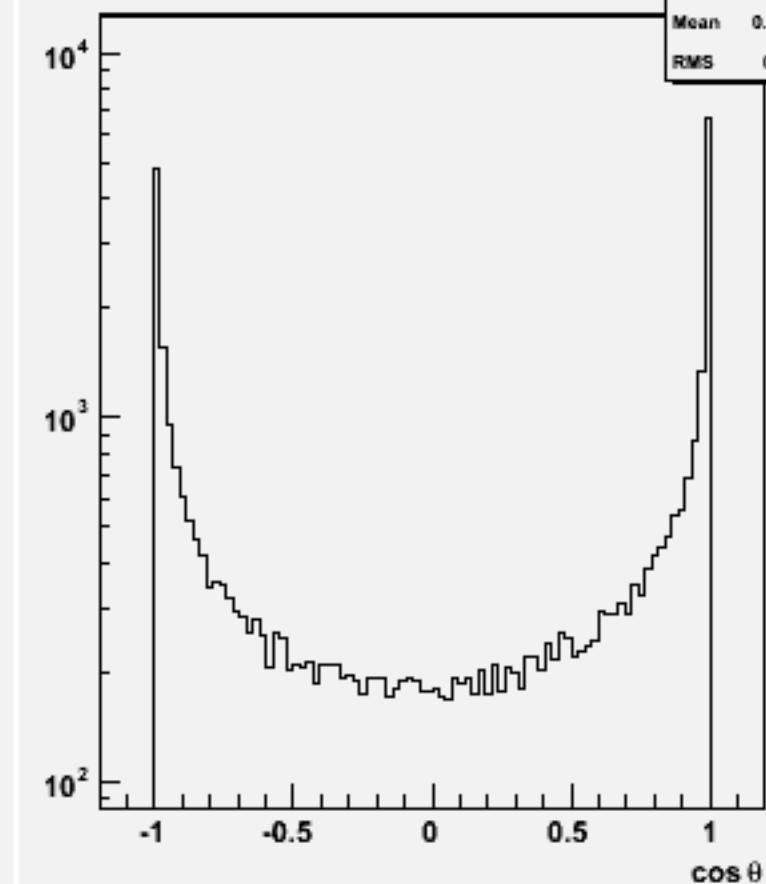
Jet cos \theta (All jets)w102083 n3n3cce1e1_o
