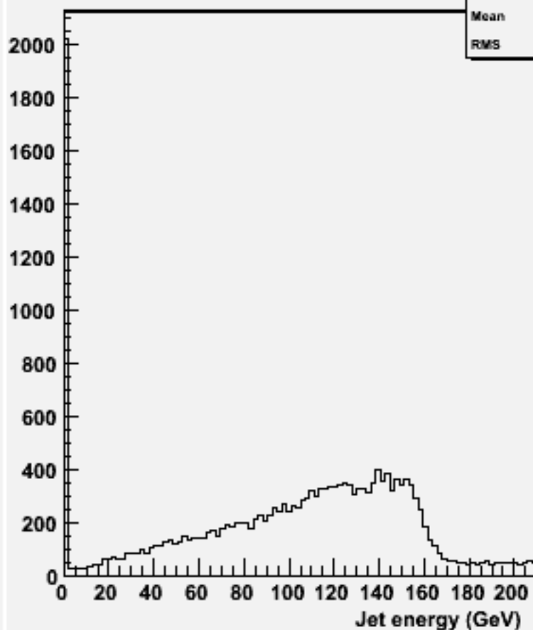
energy for 2-jets :w102083 n3n3cce1e1_o
