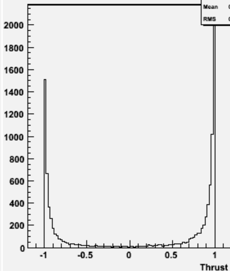
cos \Theta (thrust) w102083 n3n3cce1e1_o
