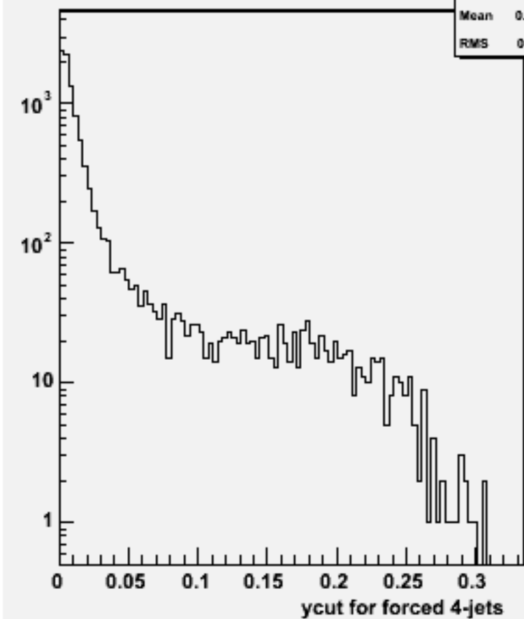
Ycut for 4-jets :w102076 n3n3uuss_o
