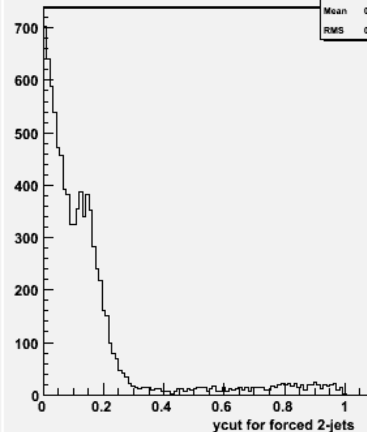
Ycut for 2-jets :w102073 n3n3uue2e2_o
