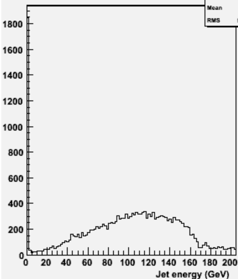
energy for 2-jets :w102073 n3n3uue2e2_o
