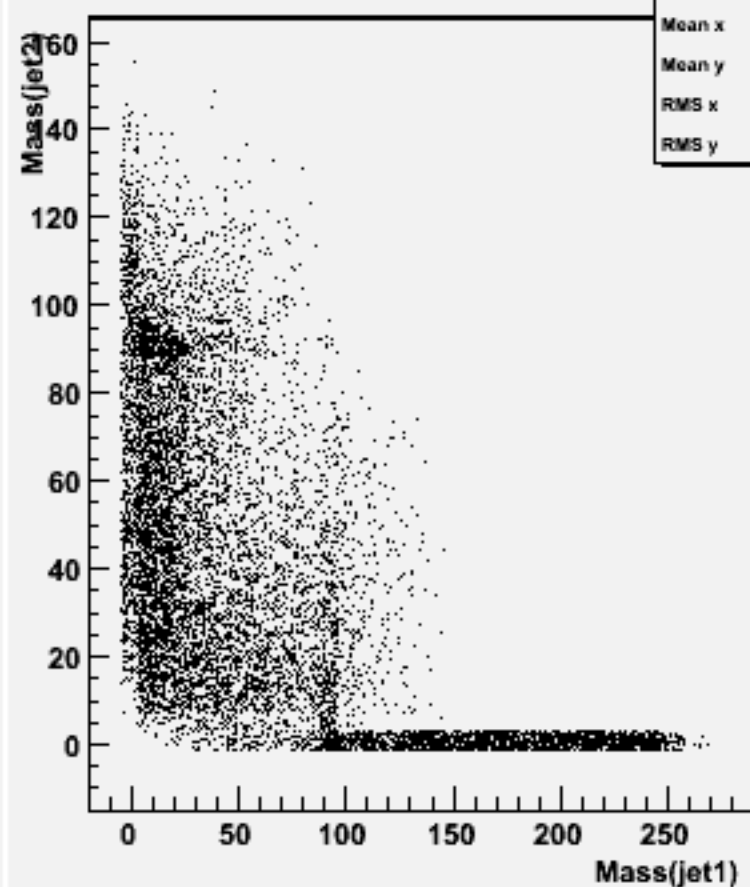
Jet mass for forced 2-jets : w102073 n3n3uue2e2_o
