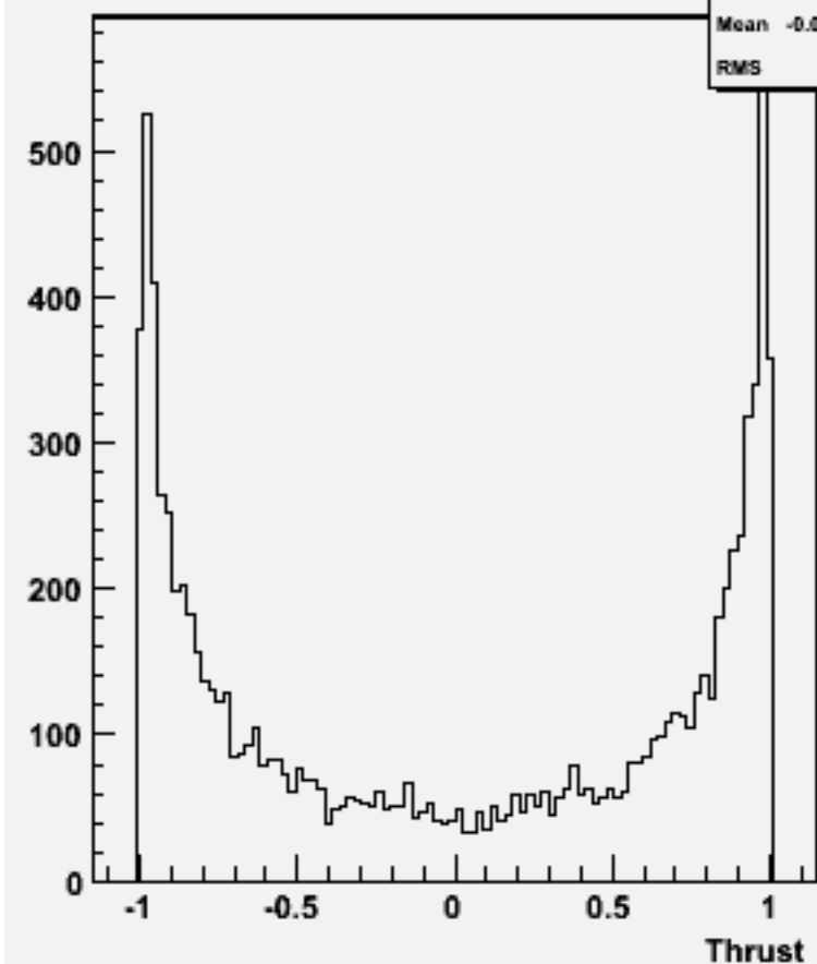
cos \Theta (thrust) w102073 n3n3uue2e2_o
