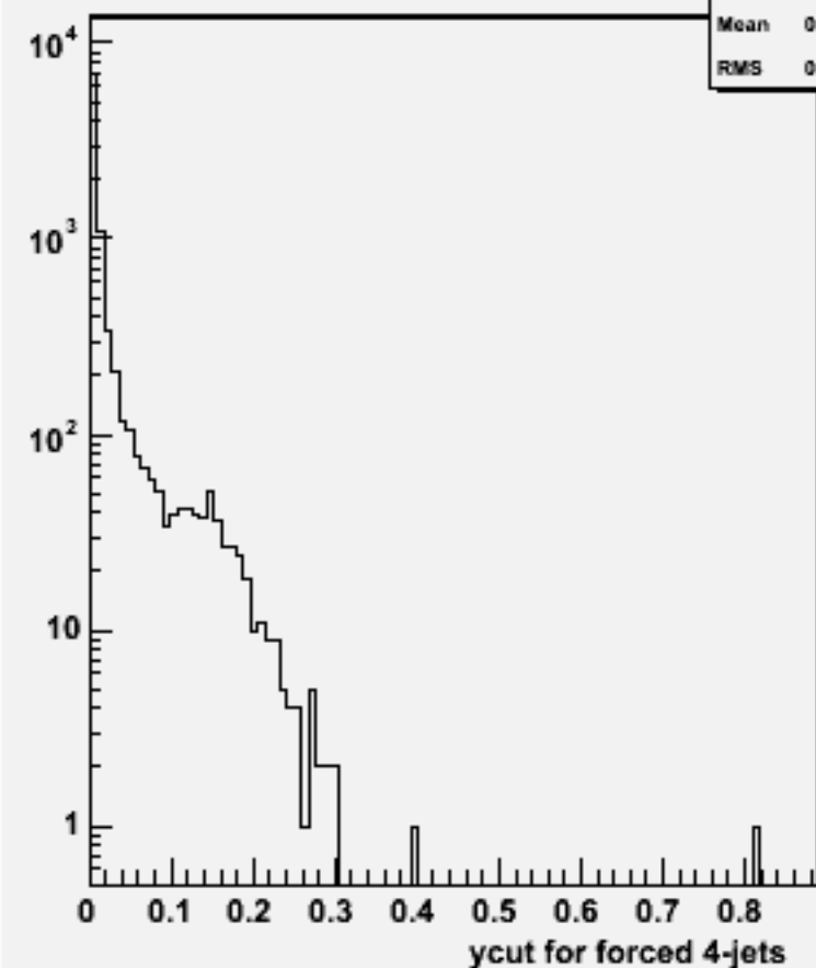
Ycut for 4-jets :w102073 n3n3uue2e2_o
