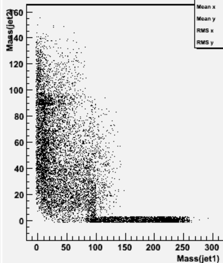
Jet mass for forced 2-jets : w102072 n3n3uue2e2_o
