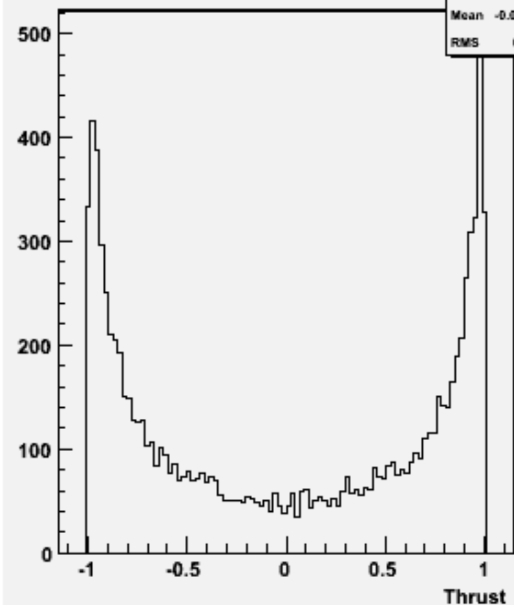
cos \Theta (thrust) w102072 n3n3uue2e2_o
