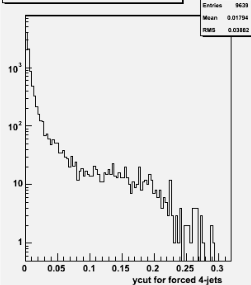
Ycut for 4-jets :w102068 n3n3uue1e1_o
