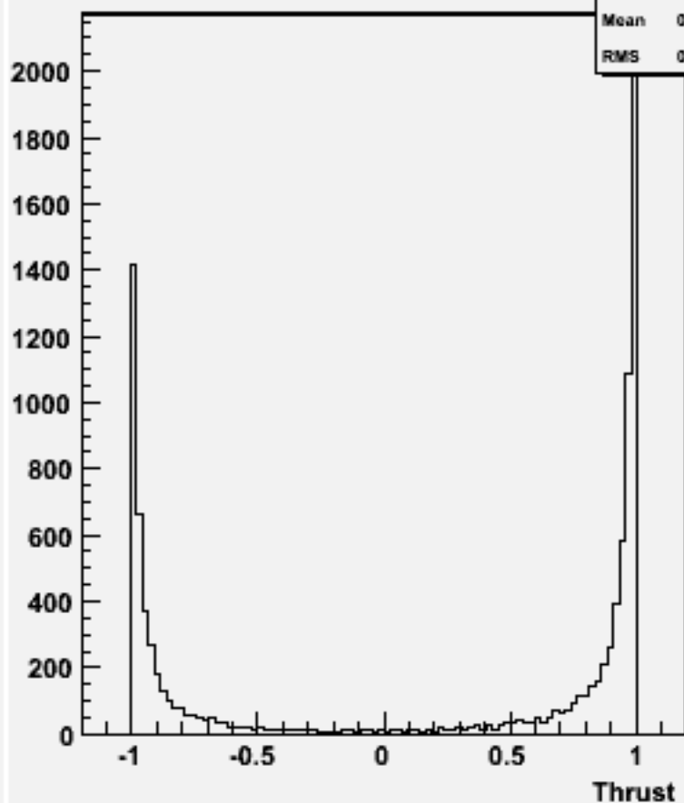
cos \Theta (thrust) w102067 n3n3uue1e1_o
