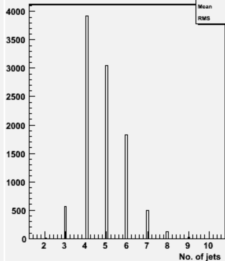
No. jets (ycut=0.001) : w102067 n3n3uue1e1_o
