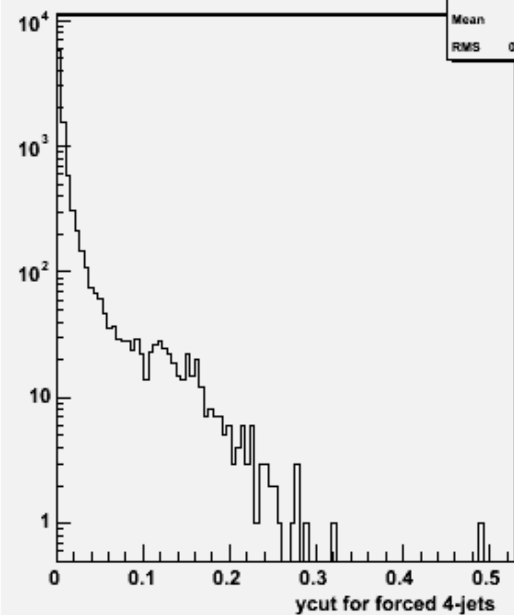
Ycut for 4-jets :w102067 n3n3uue1e1_o
