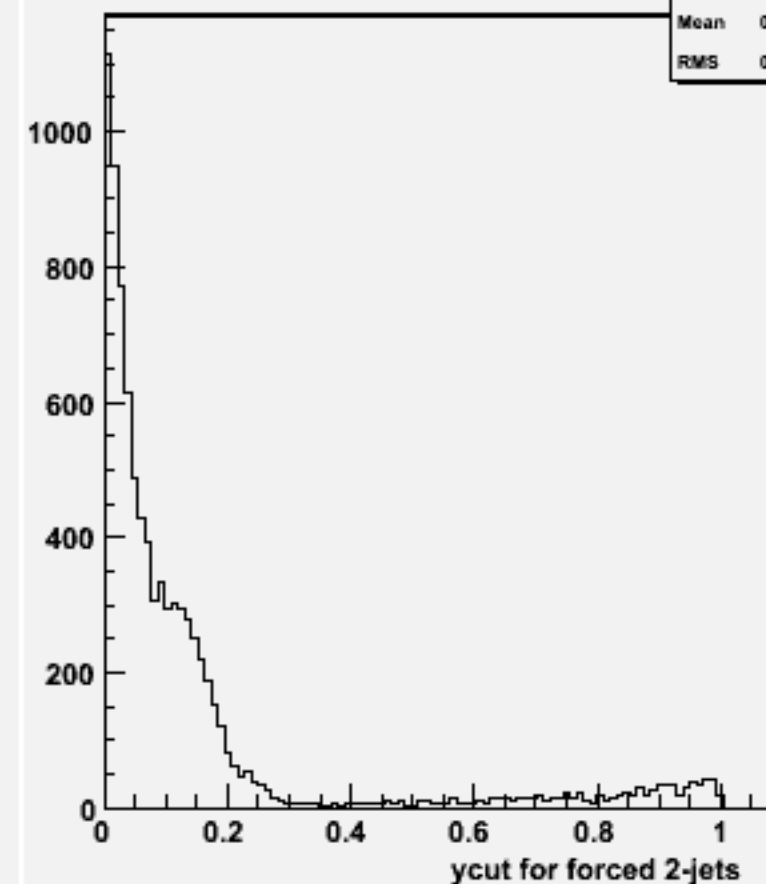
Ycut for 2-jets :w102067 n3n3uue1e1_o
