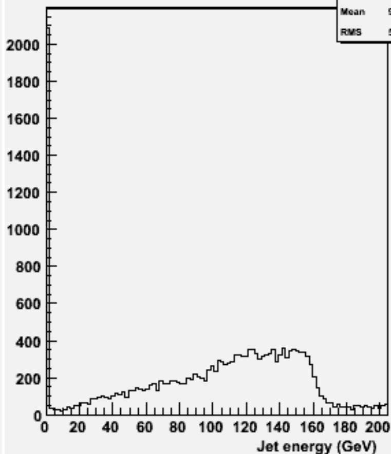
energy for 2-jets :w102067 n3n3uue1e1_o
