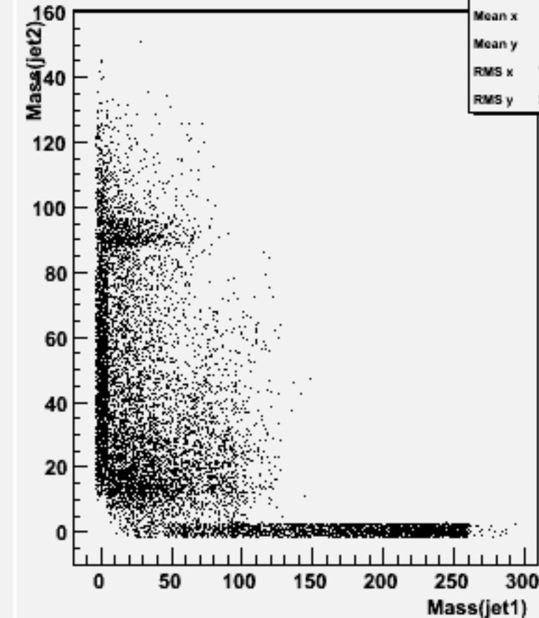
Jet mass for forced 2-jets : w102067 n3n3uue1e1_o
