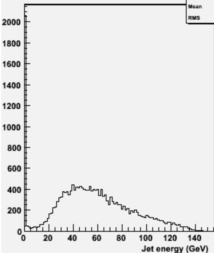
energy for 2-jets :w102064 n3n3n3n3bb_o
