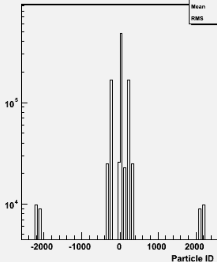
Particle ID : w102044 n2n2ccbb_o
