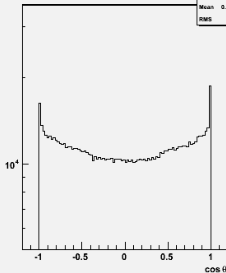
Particle cos \theta : w102044 n2n2ccbb_o
