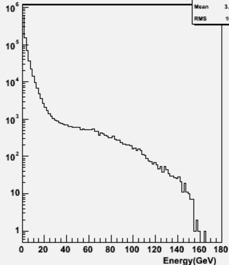
Particle Energy : w102044 n2n2ccbb_o
