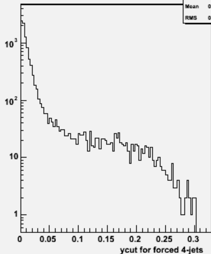
Ycut for 4-jets :w102044 n2n2ccbb_o
