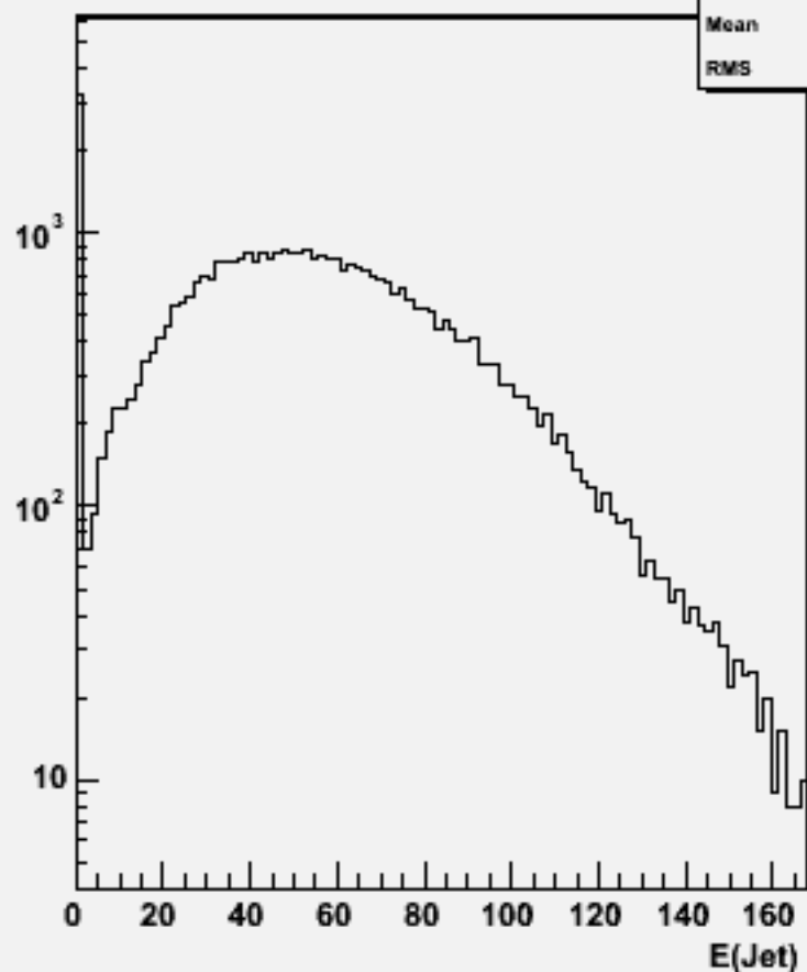
Jet energies(All jets)w102044 n2n2ccbb_o
