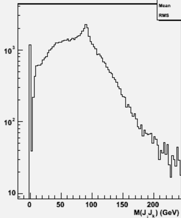
2jets mass(All comb)w102044 n2n2ccbb_o
