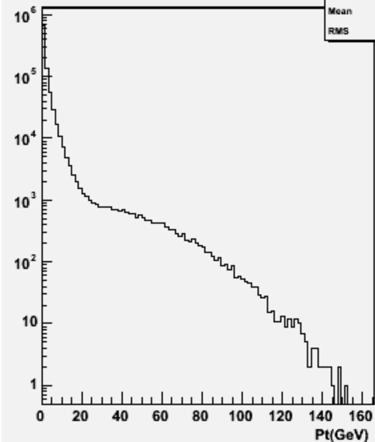
Particle Pt : w102044 n2n2ccbb_o
