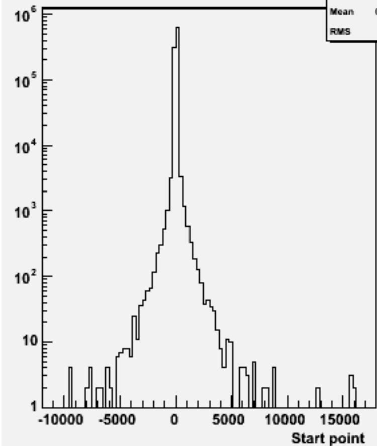
Start point Z : w102044 n2n2ccbb_o
