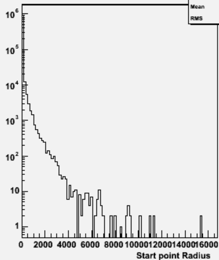
Start point R : w102044 n2n2ccbb_o
