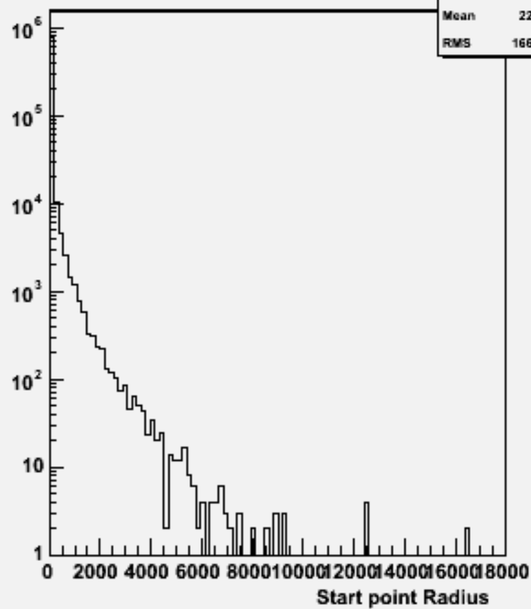
Start point R : w102041 n2n2ccdd_o
