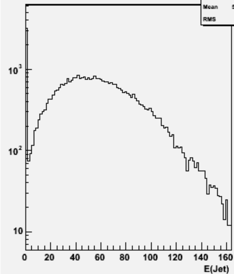
Jet energies(All jets)w102041 n2n2ccdd_o
