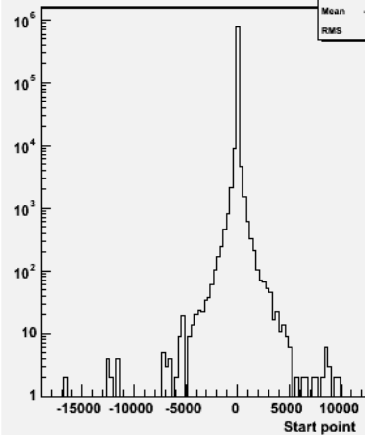
Start point Z : w102041 n2n2ccdd_o
