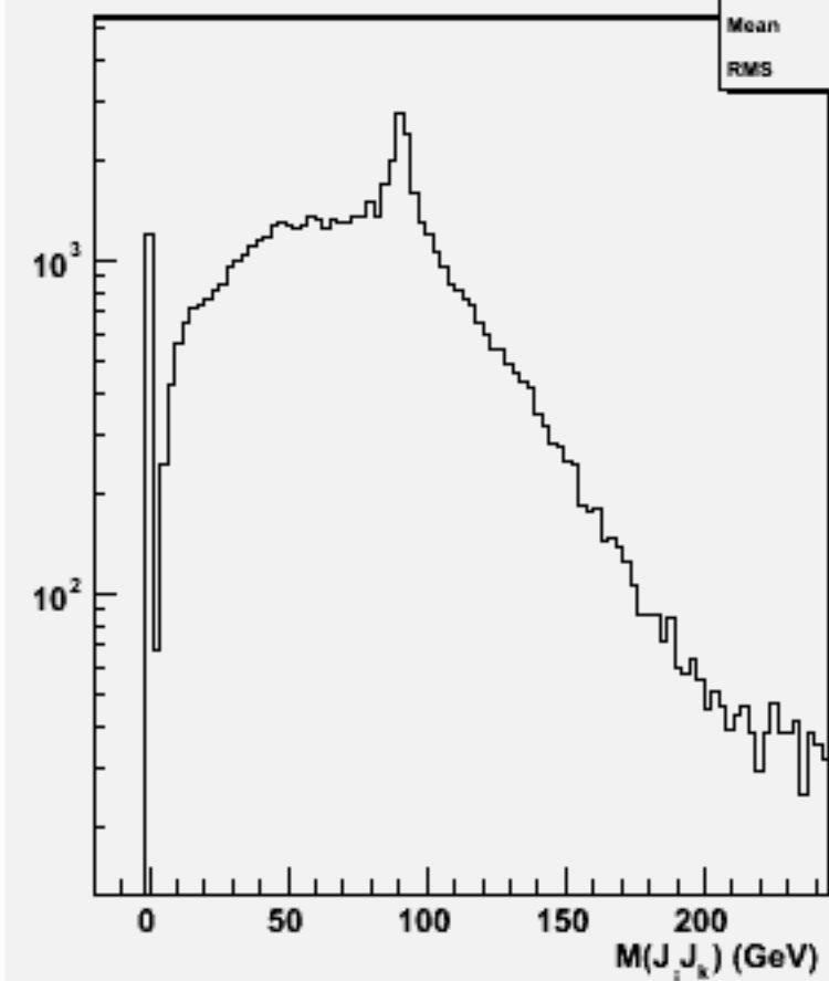
2jets mass(All comb)w102041 n2n2ccdd_o
