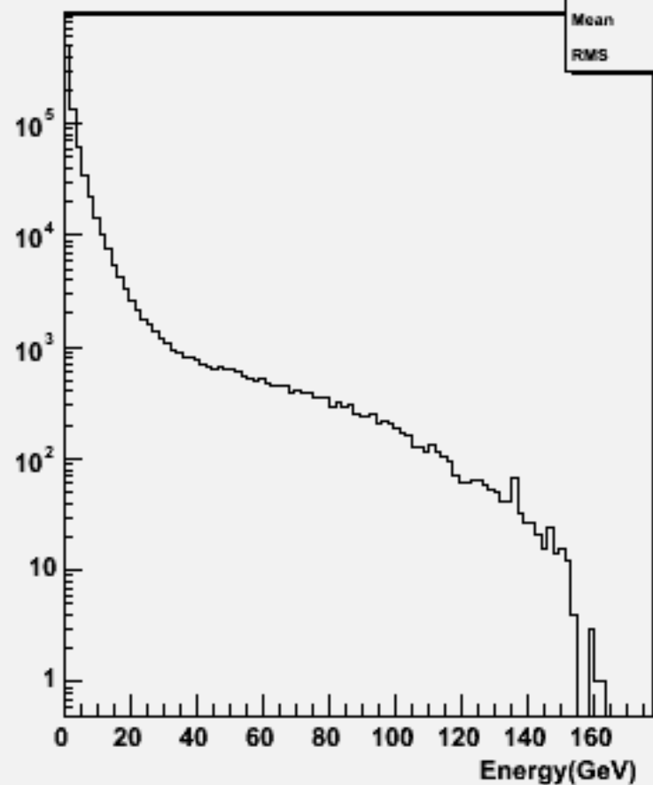
Particle Energy : w102041 n2n2ccdd_o
