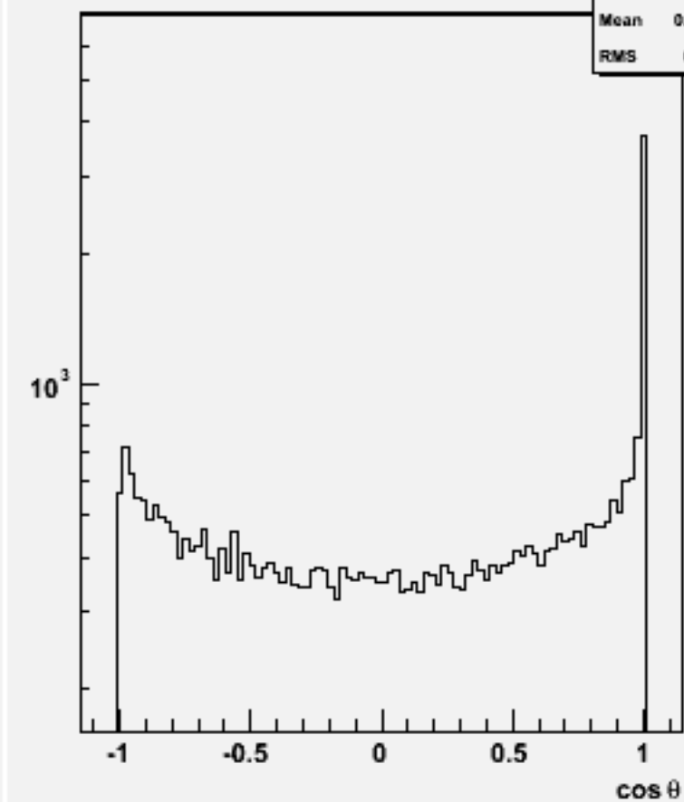
Jet cos \theta (All jets)w102041 n2n2ccdd_o
