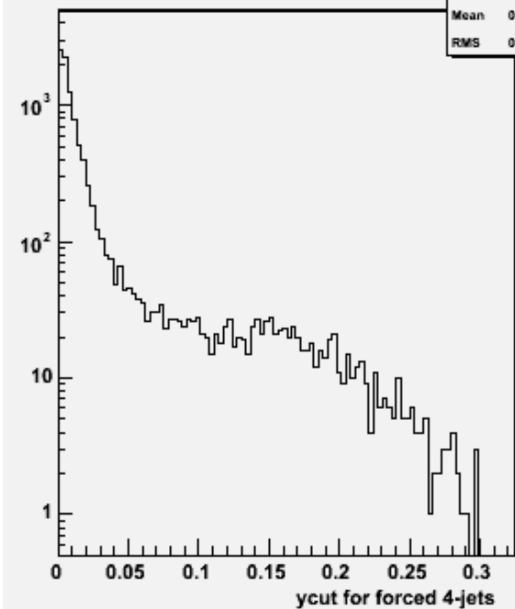
Ycut for 4-jets :w102041 n2n2ccdd_o
