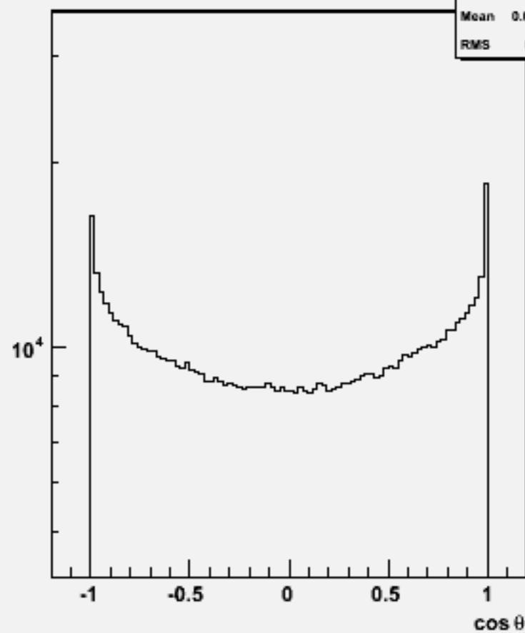
Particle cos \theta : w102041 n2n2ccdd_o
