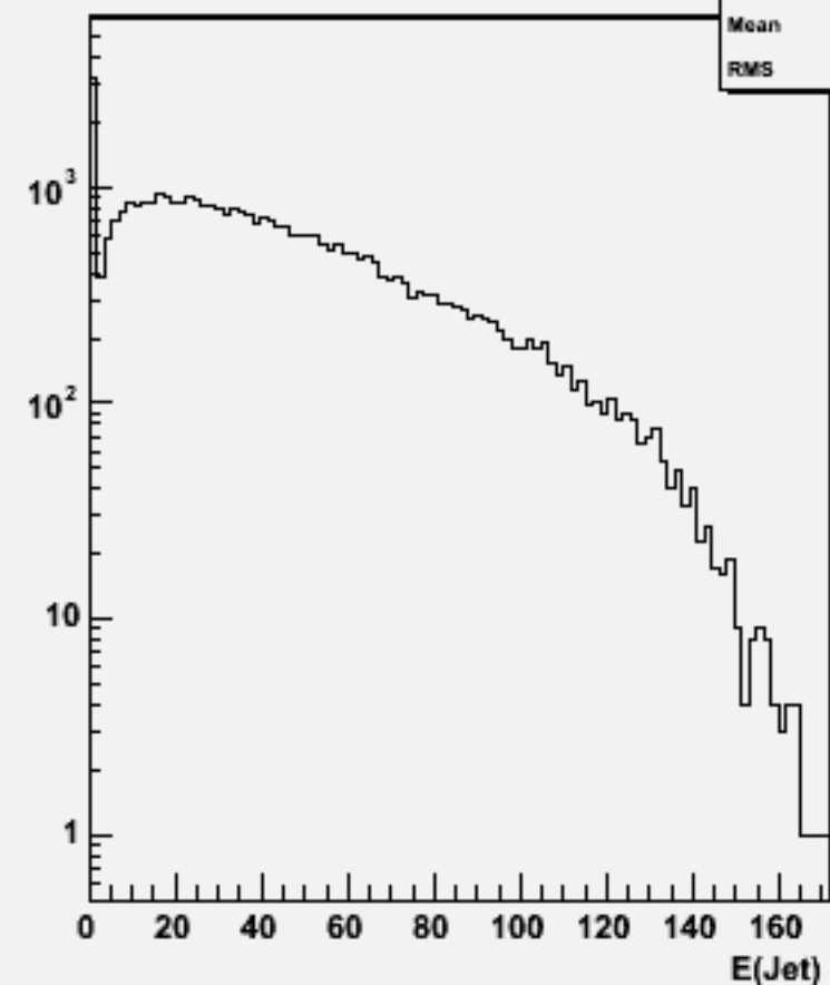
Jet energies(All jets)w102037 n2n2cce3e3_o
