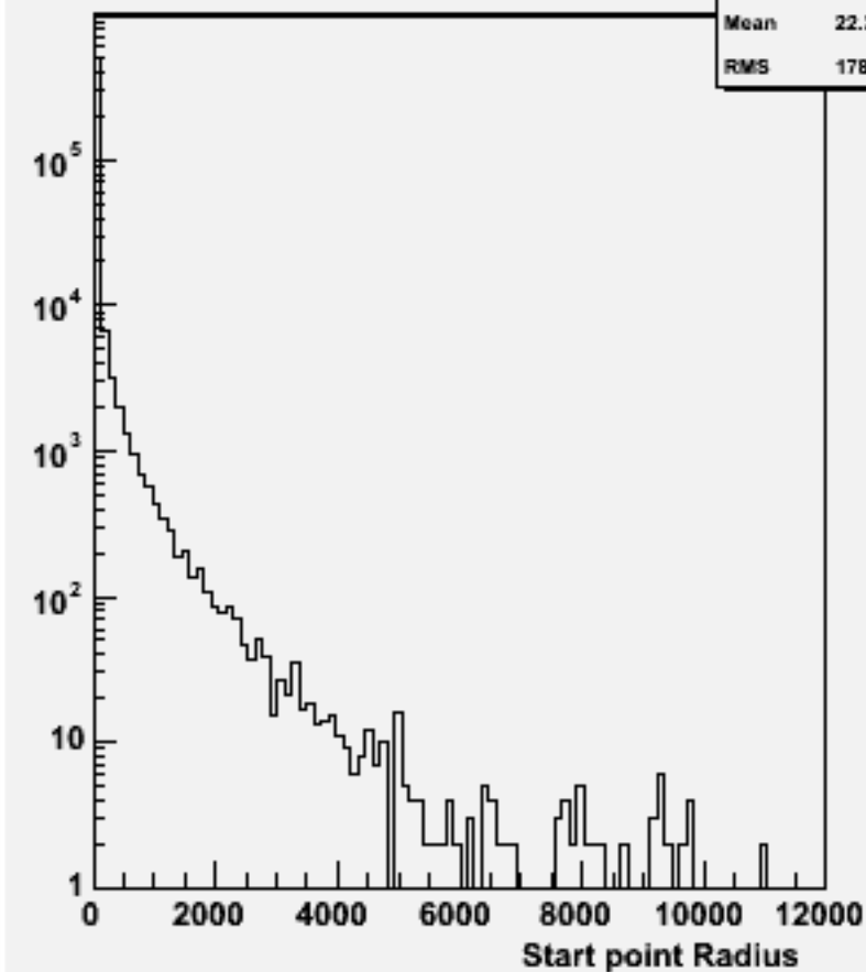
Start point R : w102037 n2n2cce3e3_o
