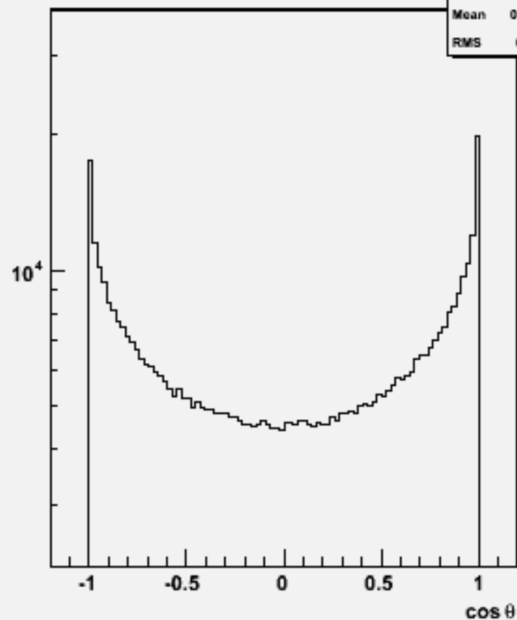
Particle cosθ : w102037 n2n2cce3e3_o
