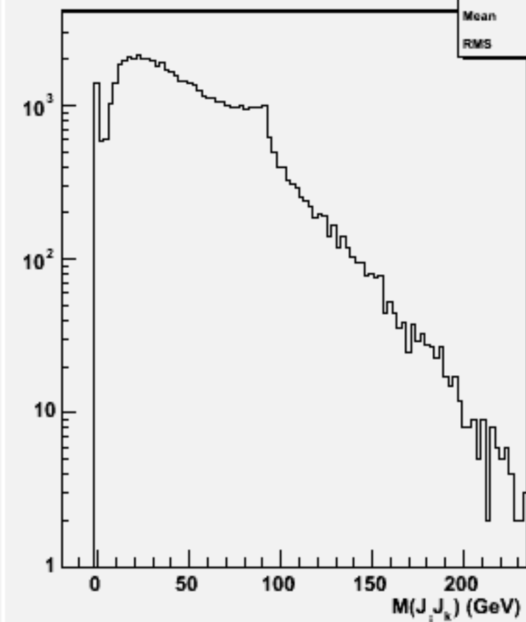
2jets mass(All comb)w102037 n2n2cce3e3_o
