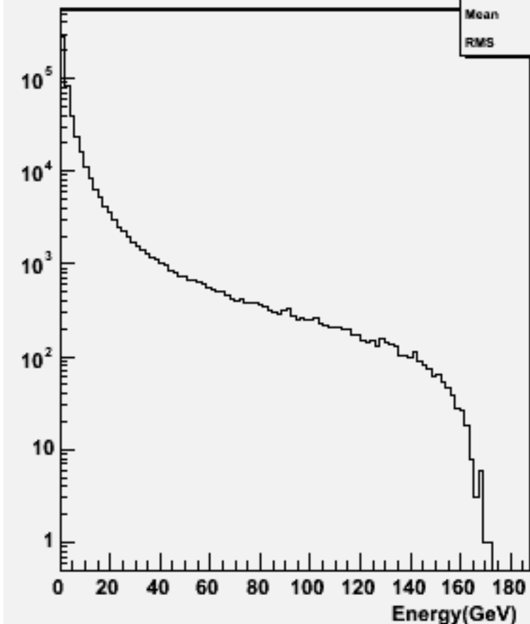
Start point R : w102037 n2n2cce3e3_o
