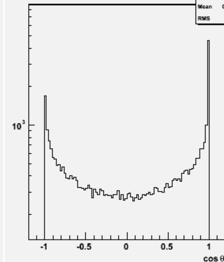
Jet cos \theta (All jets)w102037 n2n2cce3e3_o
