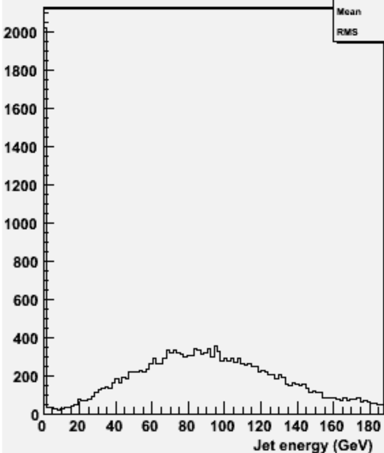
energy for 2-jets :w102036 n2n2cce3e3_o
