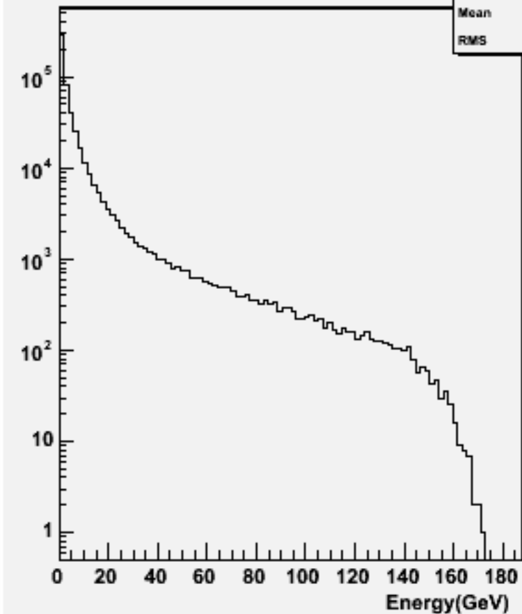
Start point R : w102036 n2n2cce3e3_o
