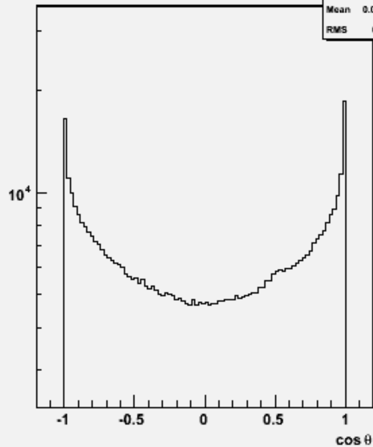
Particle cos \theta : w102036 n2n2cce3e3_o
