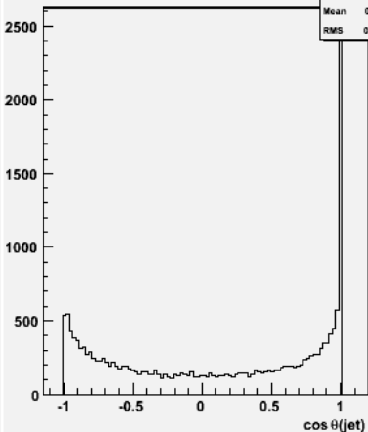
cos \theta for 2-jets :w102036 n2n2cce3e3_o
