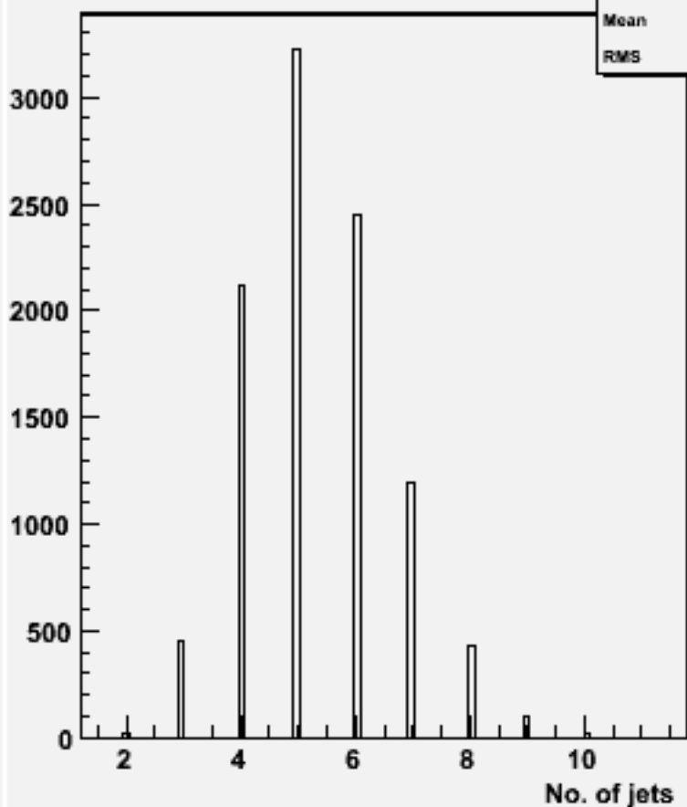
No. jets (ycut=0.001) : w102036 n2n2cce3e3_o
