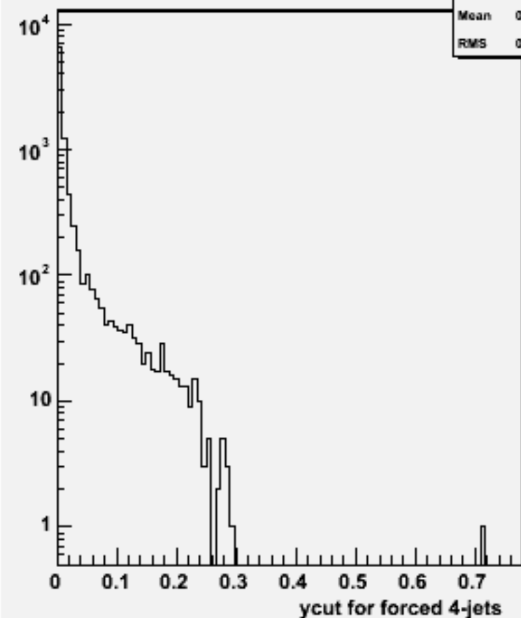
Ycut for 4-jets :w102036 n2n2cce3e3_o
