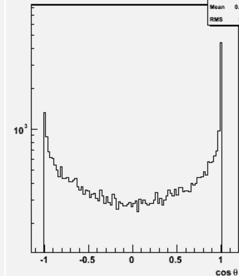
Jet cos \theta (All jets)w102036 n2n2cce3e3_o
