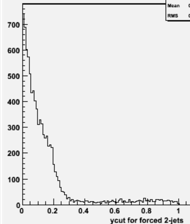
Ycut for 2-jets :w102036 n2n2cce3e3_o
