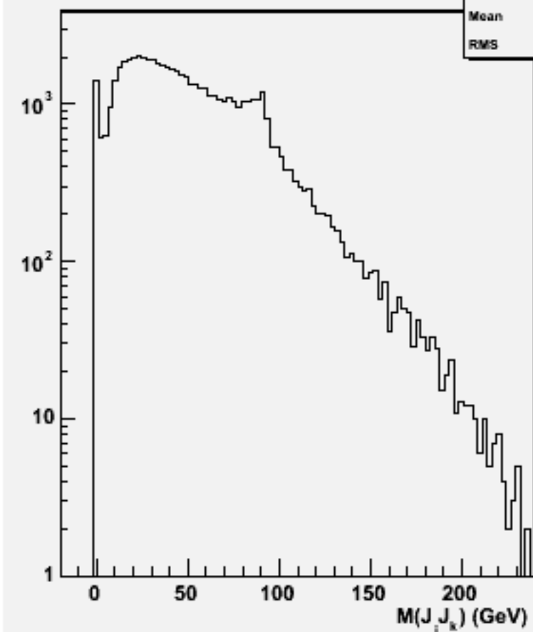
2jets mass(All comb)w102036 n2n2cce3e3_o
