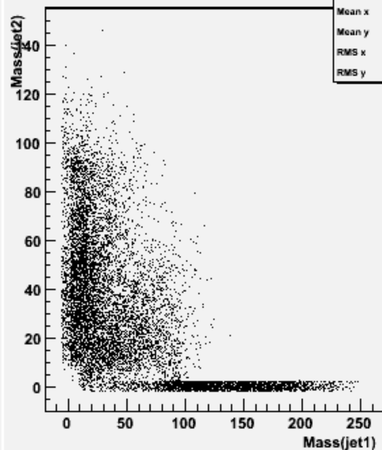
Jet mass for forced 2-jets : w102036 n2n2cce3e3_o
