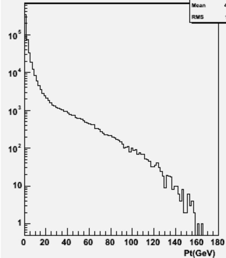
Start point Z : w102036 n2n2cce3e3_o
