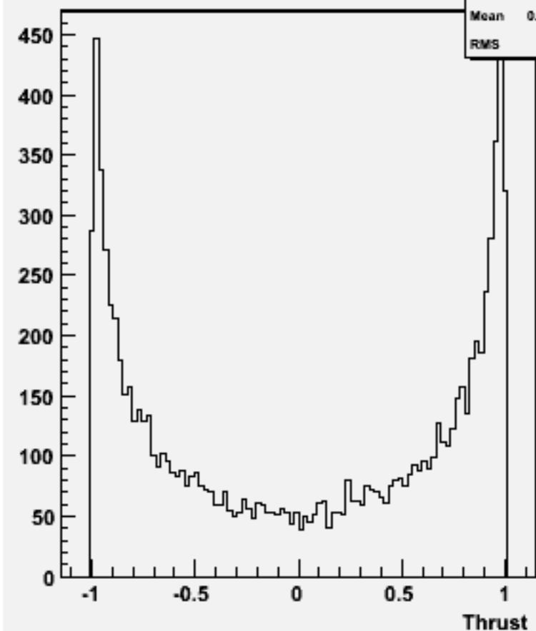
cos \Theta (thrust) w102036 n2n2cce3e3_o
