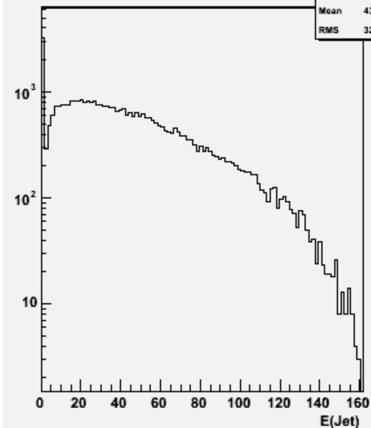
Jet energies(All jets)w102036 n2n2cce3e3_o
