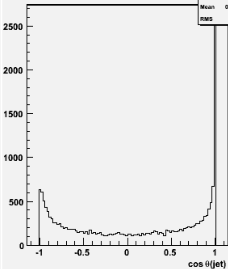
cos \theta for 2-jets :w102032 n2n2cce1e1_o
