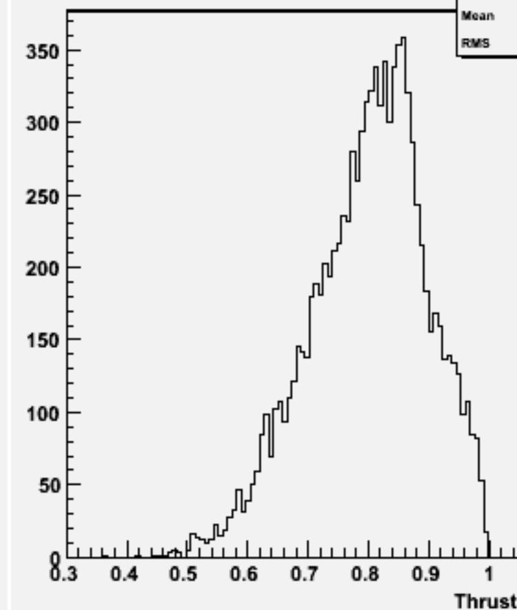
Thrust w102032 n2n2cce1e1_o
