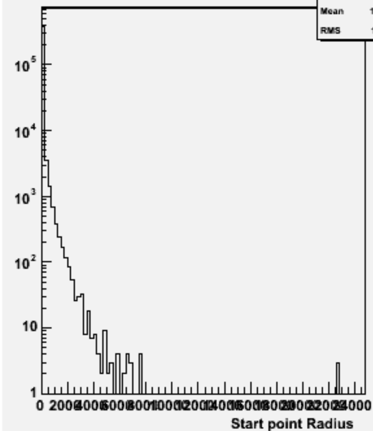
Start point R : w102031 n2n2cce1e1_o
