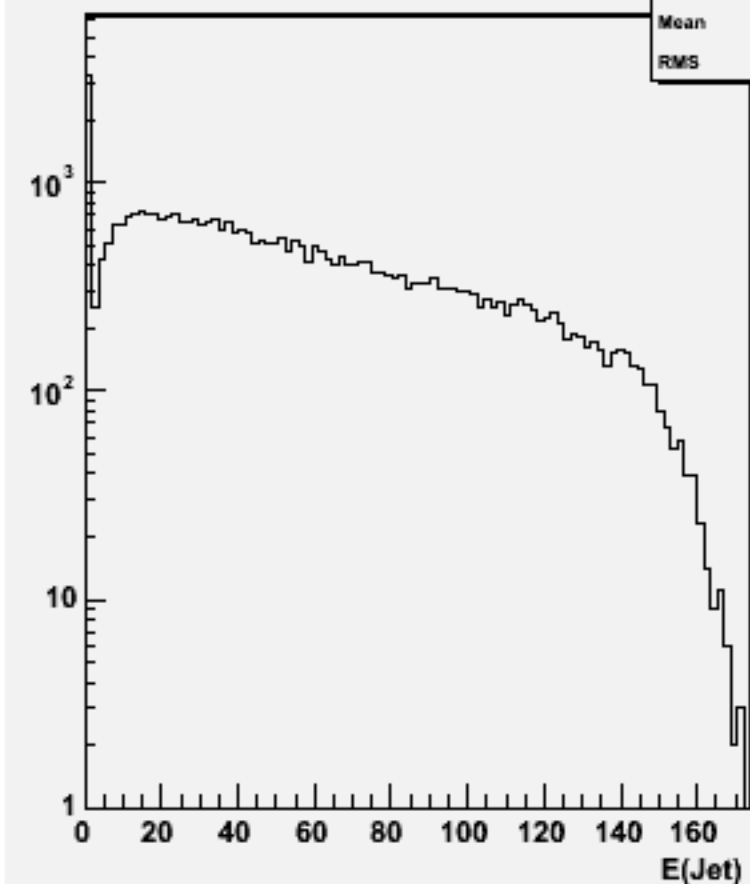
Jet energies(All jets)w102031 n2n2cce1e1_o
