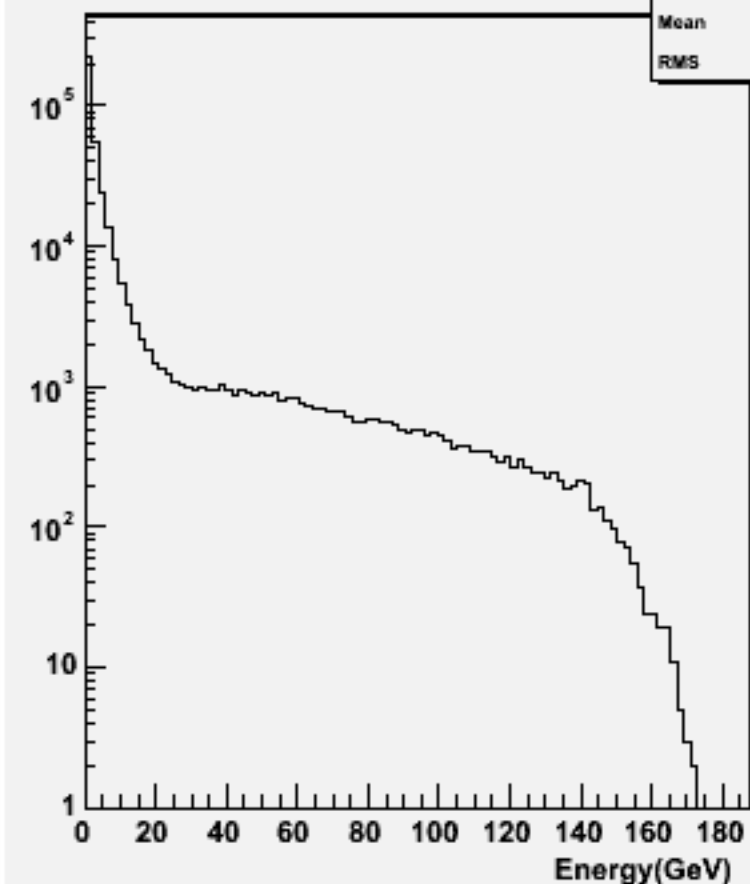
Particle Energy : w102031 n2n2cce1e1_o
