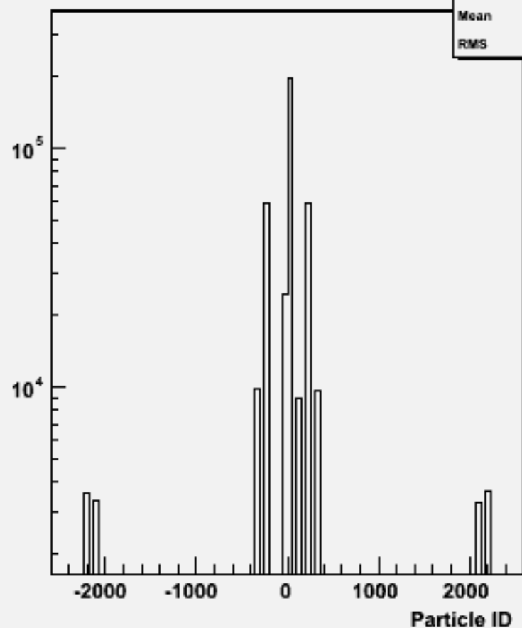
Particle ID : w102031 n2n2cce1e1_o
