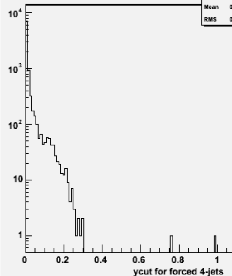
Ycut for 4-jets :w102031 n2n2cce1e1_o
