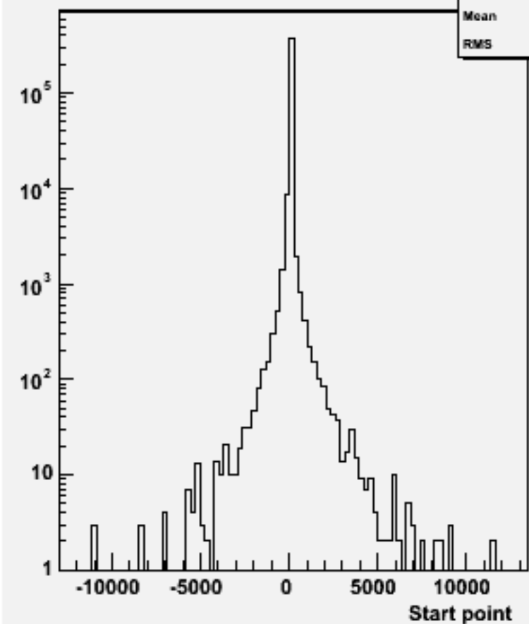
Start point Z : w102031 n2n2cce1e1_o
