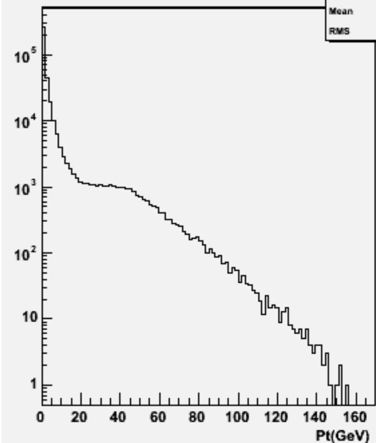
Particle Pt : w102031 n2n2cce1e1_o
