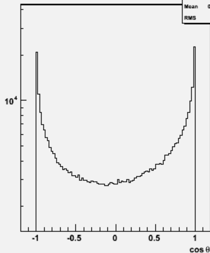
Particle cosθ : w102031 n2n2cce1e1_o
