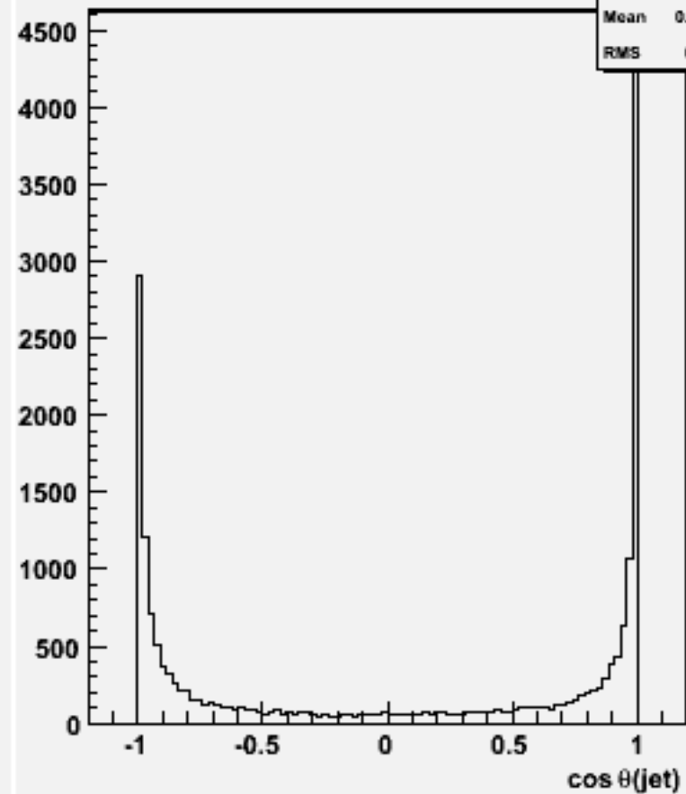
cos \theta for 2-jets :w102031 n2n2cce1e1_o
