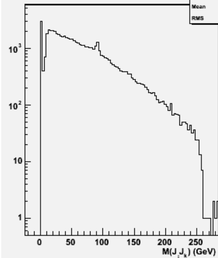
2jets mass(All comb)w102031 n2n2cce1e1_o
