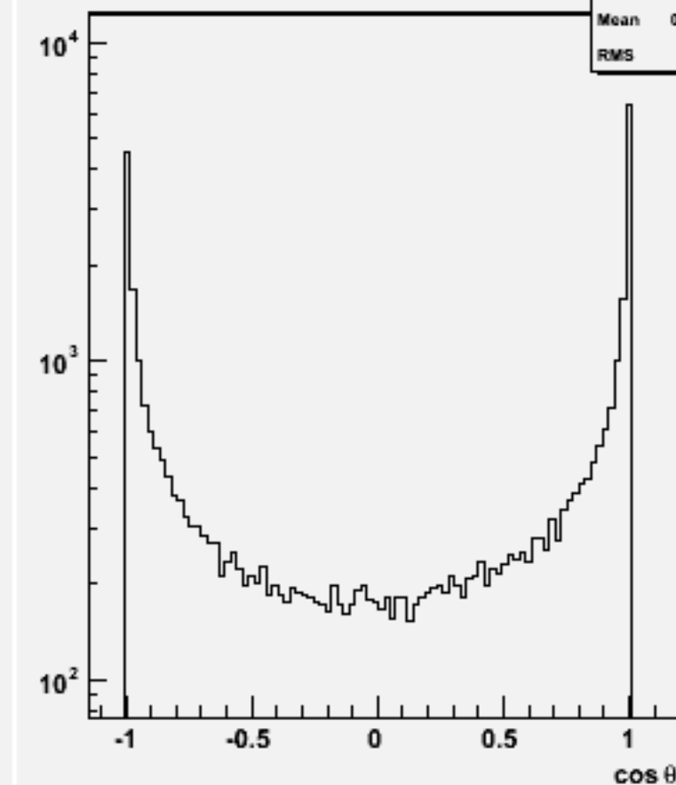
Jet cos \theta (All jets)w102031 n2n2cce1e1_o
