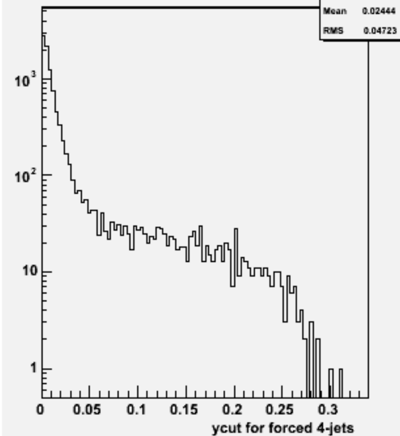
Ycut for 4-jets :w102029 n2n2uubb_o
