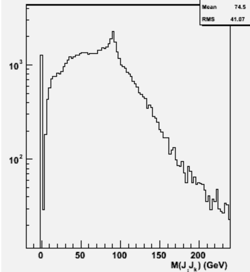
2jets mass(All comb)w102029 n2n2uubb_o
