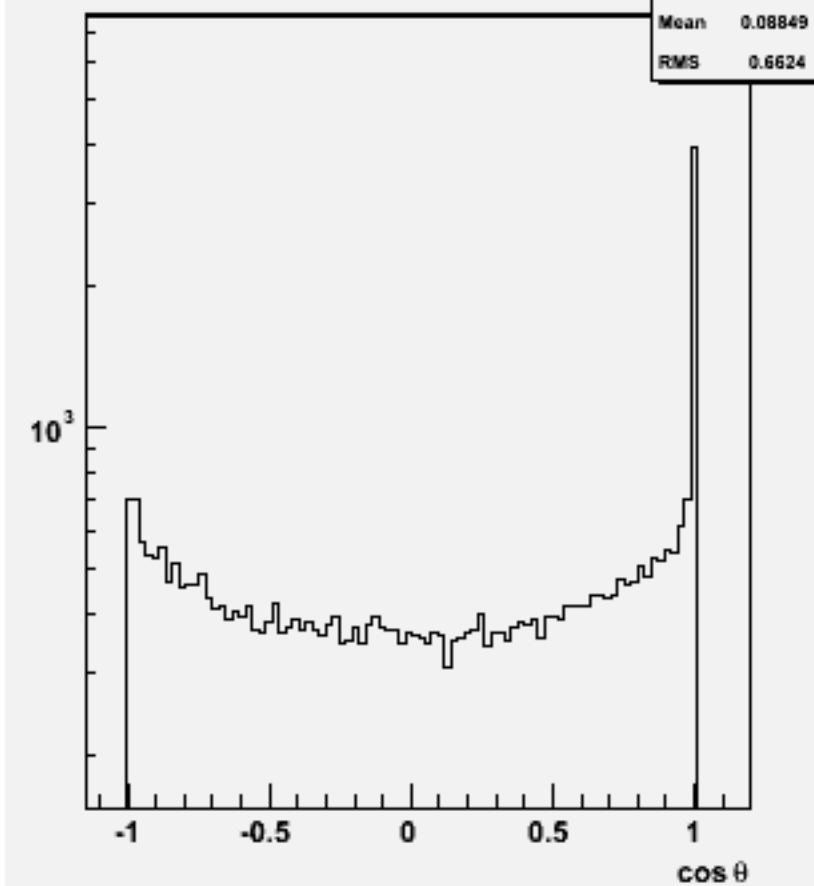
Jet cos \theta (All jets)w102029 n2n2uubb_o
