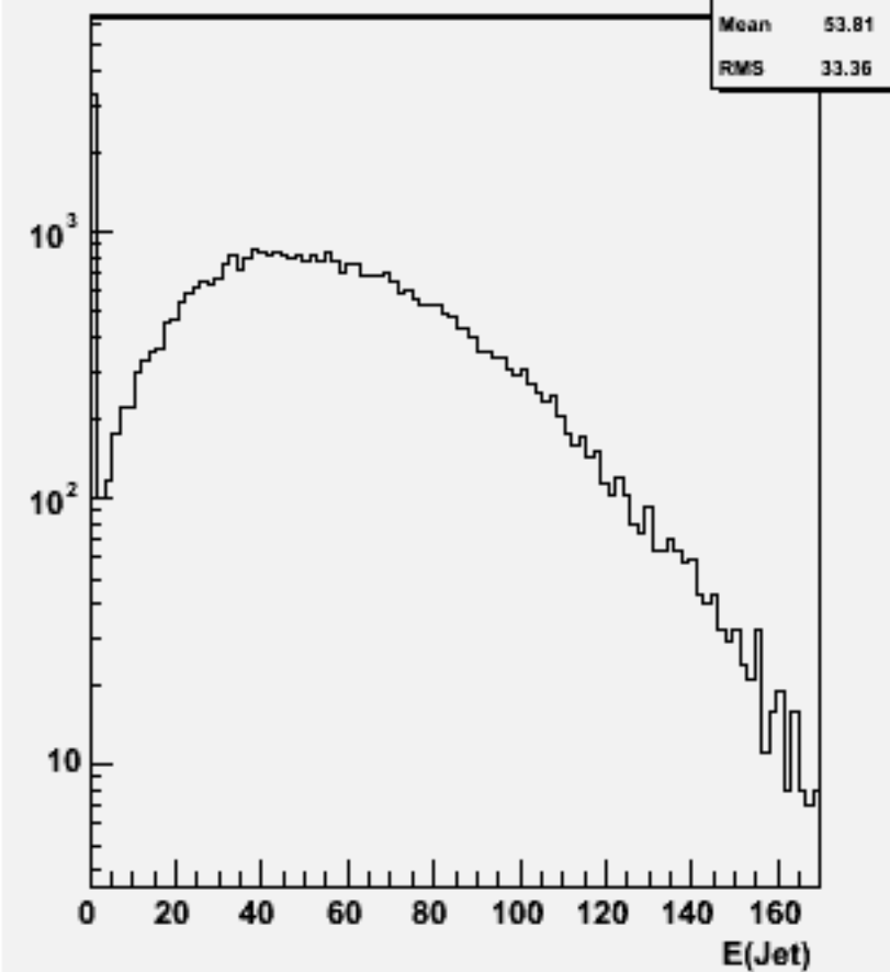
Jet energies(All jets)w102029 n2n2uubb_o
