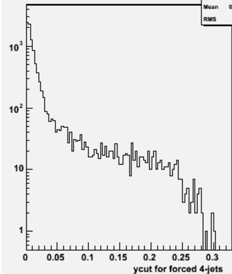
Ycut for 4-jets :w102028 n2n2uubb_o
