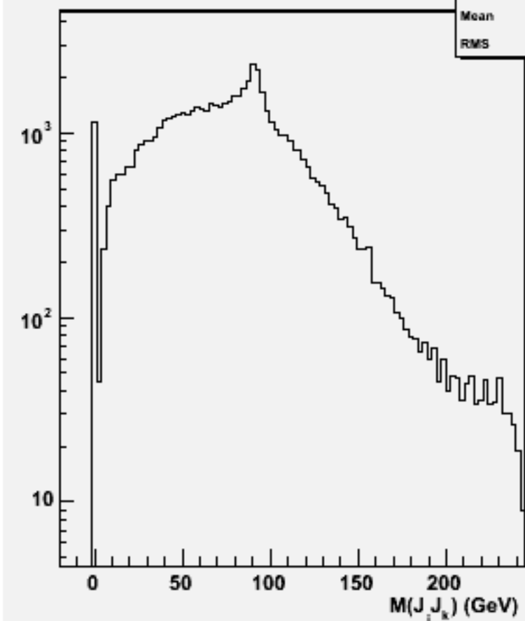
2jets mass(All comb)w102028 n2n2uubb_o
