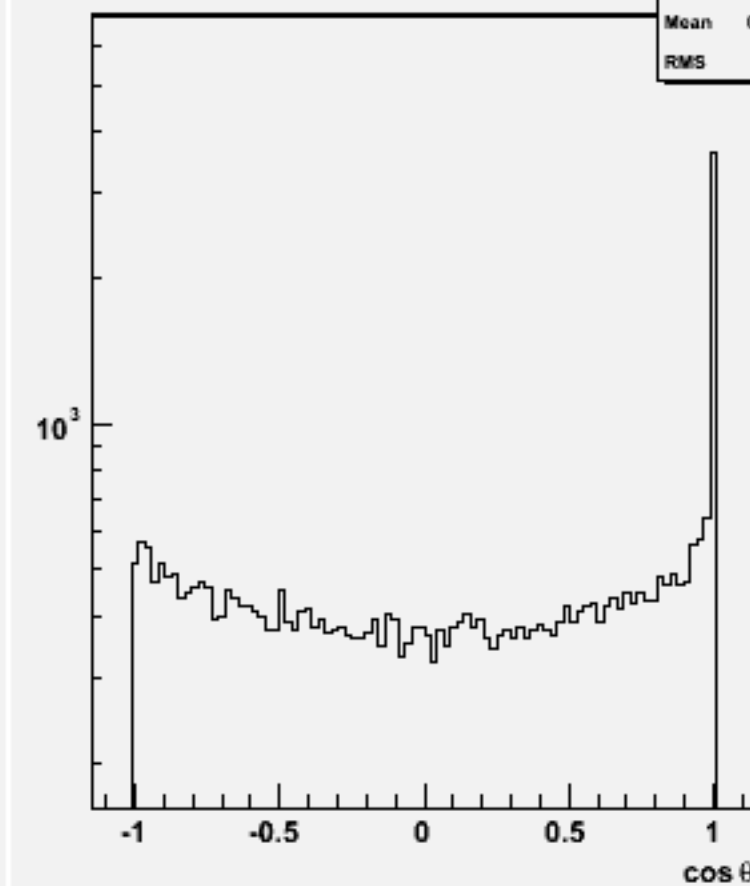
Jet cosθ (All jets)w102028 n2n2uubb_o
