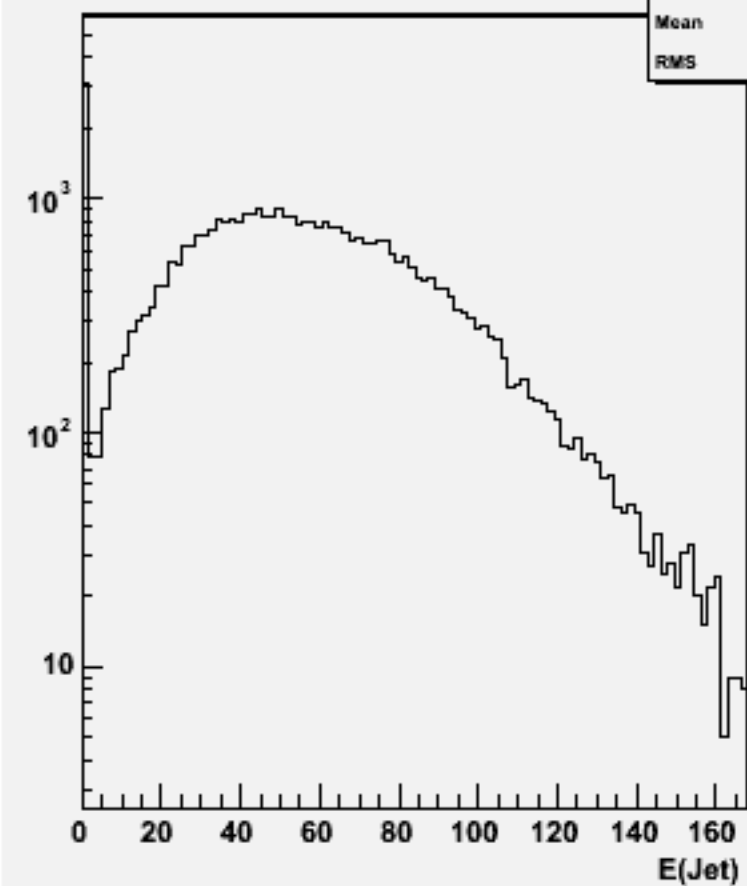
Jet energies(All jets)w102028 n2n2uubb_o
