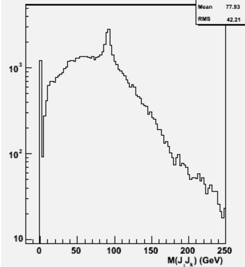
2jets mass(All comb)w102025 n2n2uuss_o
