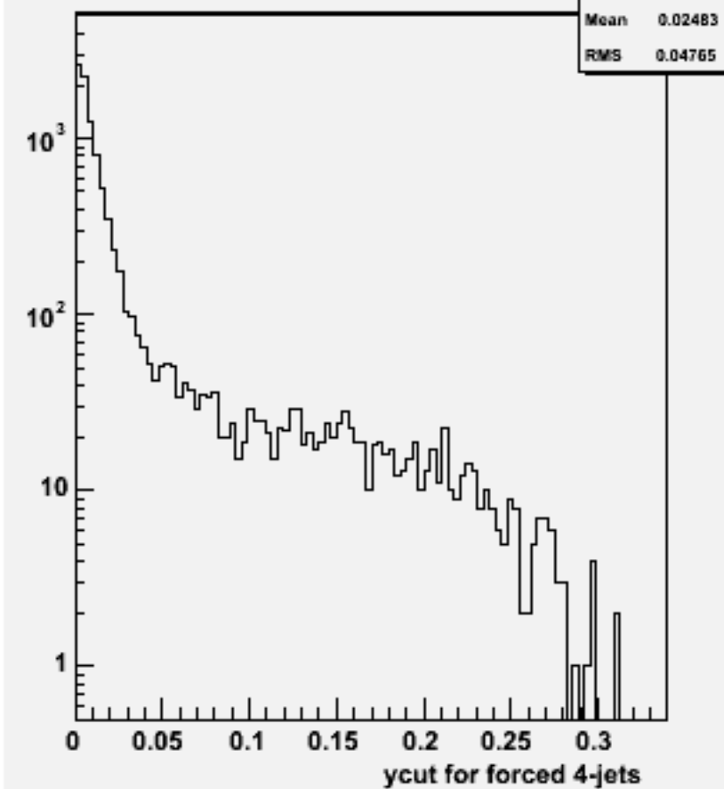
Ycut for 4-jets :w102025 n2n2uuss_o
