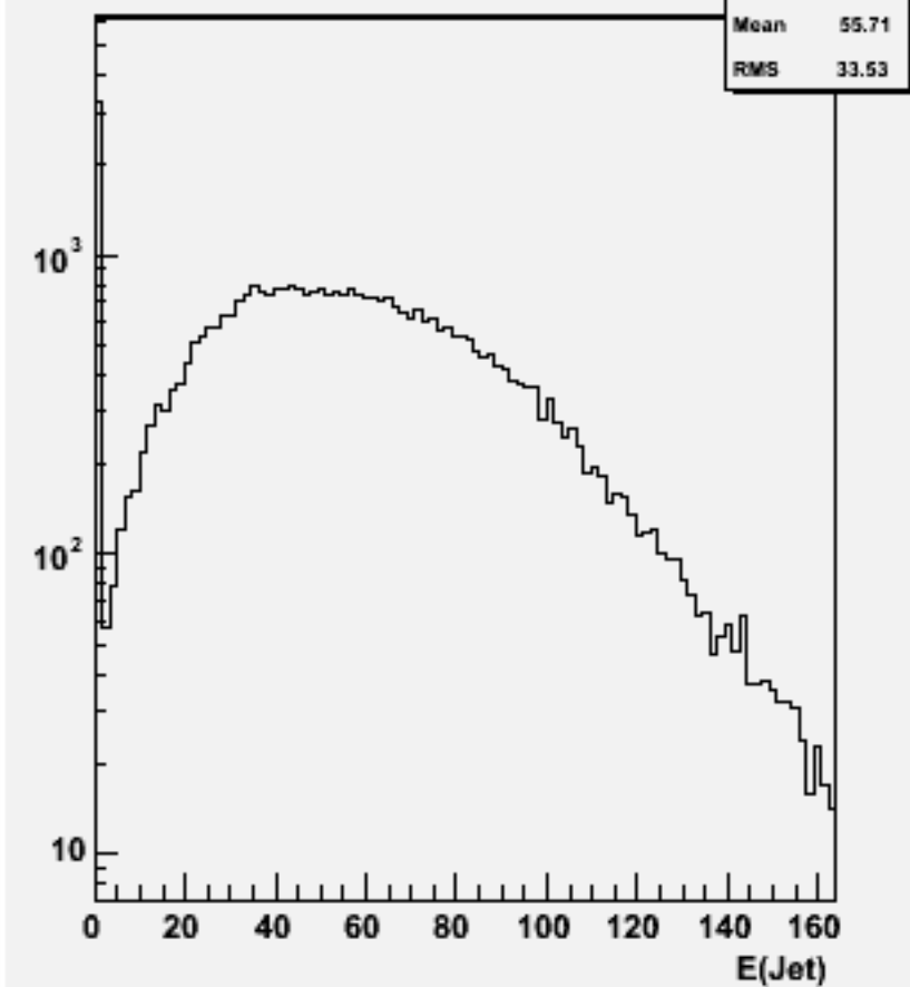
Jet energies(All jets)w102025 n2n2uuss_o
