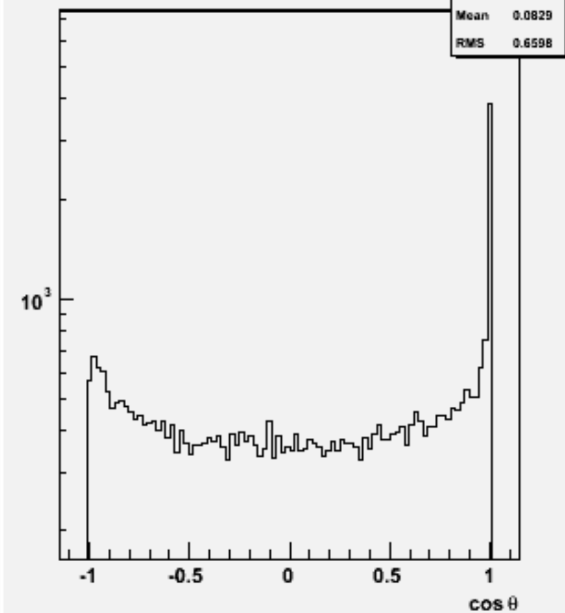
Jet cos \theta (All jets)w102025 n2n2uuss_o
