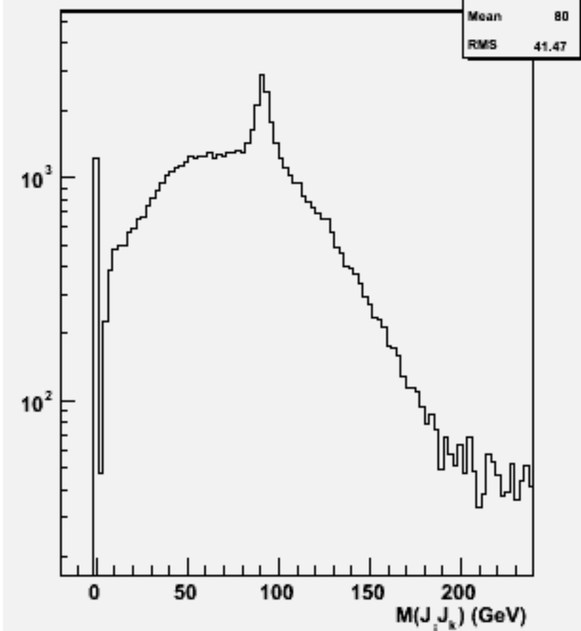
2jets mass(All comb)w102024 n2n2uuss_o
