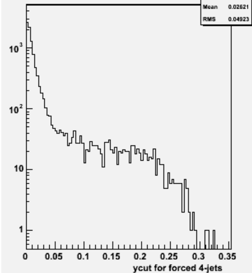
Ycut for 4-jets :w102024 n2n2uuss_o
