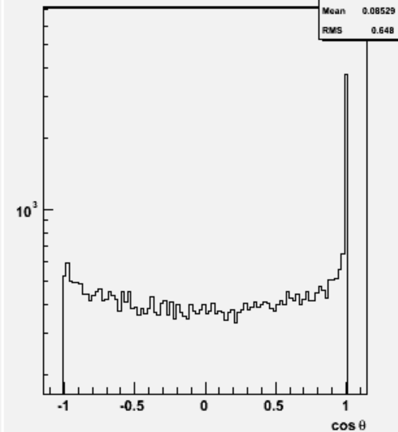
Jet cosθ (All jets)w102024 n2n2uuss_o
