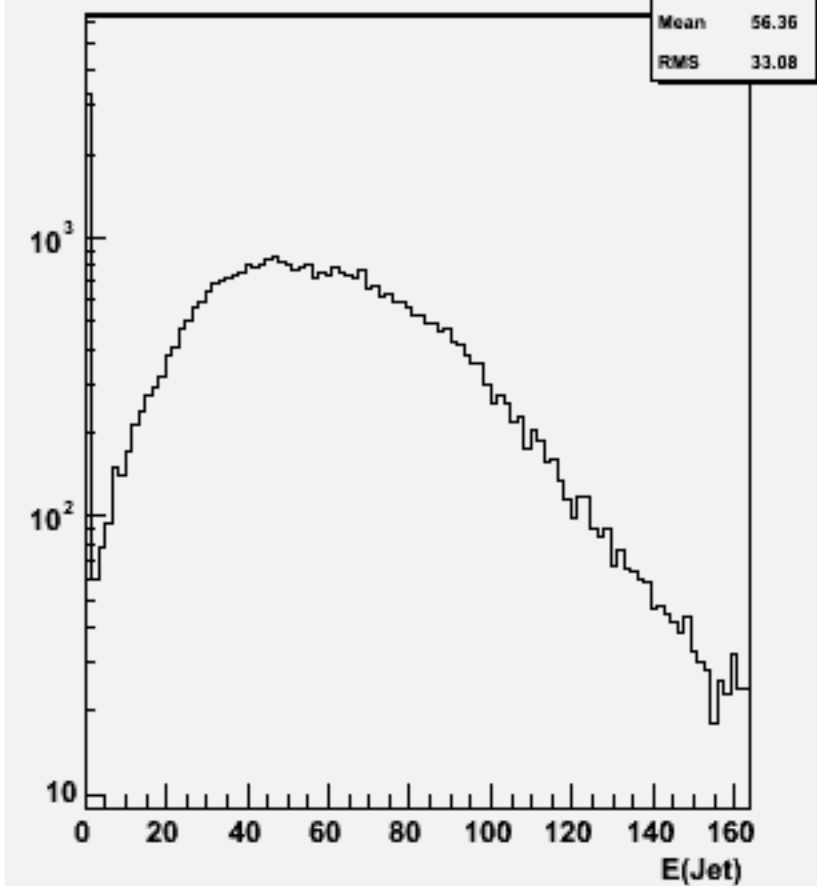
Jet energies(All jets)w102024 n2n2uuss_o
