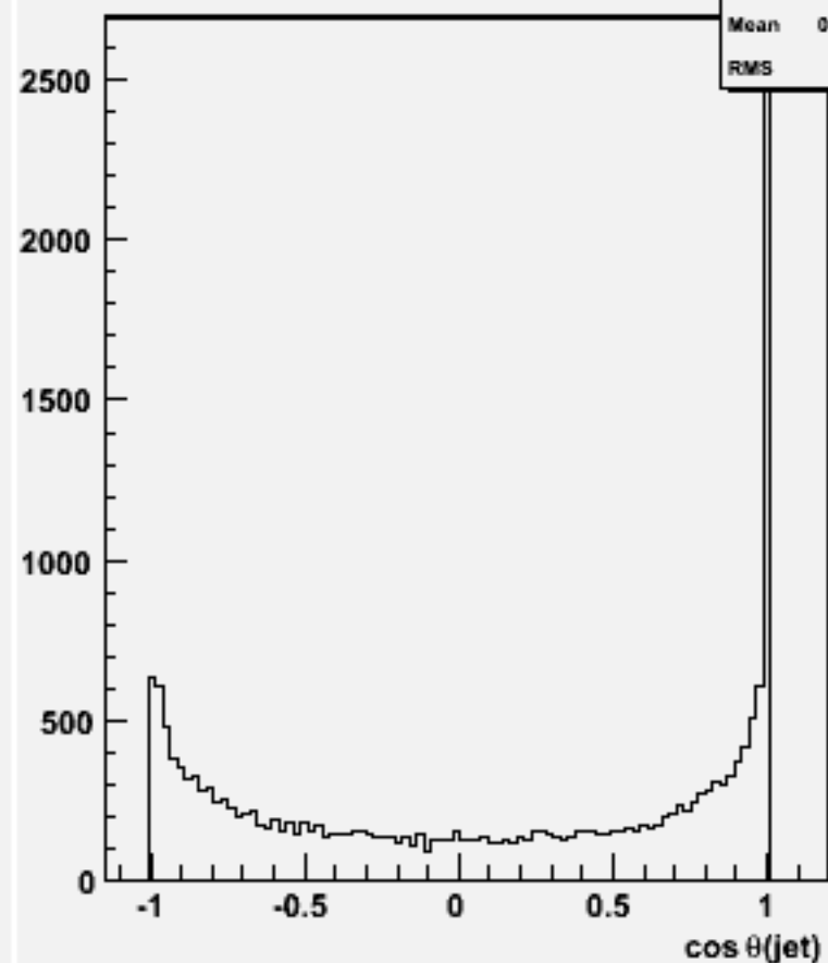
cos \theta for 2-jets :w102021 n2n2uue3e3_o
