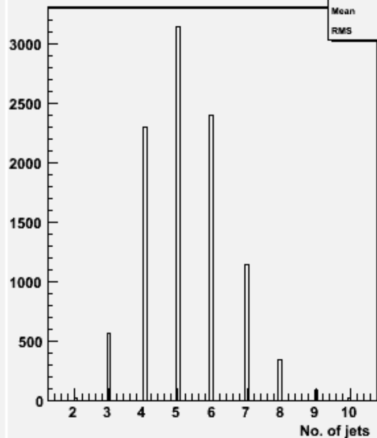
No. jets (ycut=0.001) : w102021 n2n2uue3e3_o
