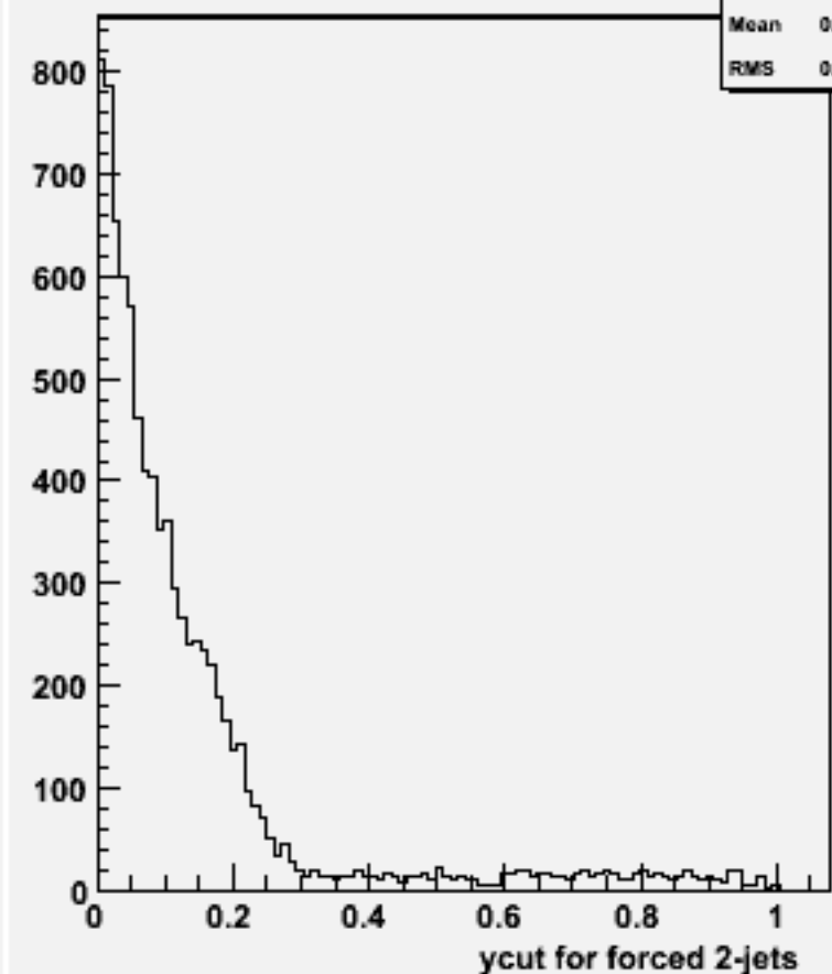
Ycut for 2-jets :w102021 n2n2uue3e3_o
