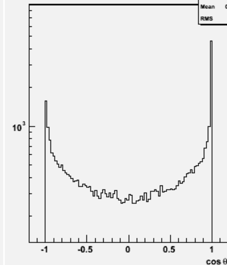
Jet cos \theta (All jets)w102021 n2n2uue3e3_o
