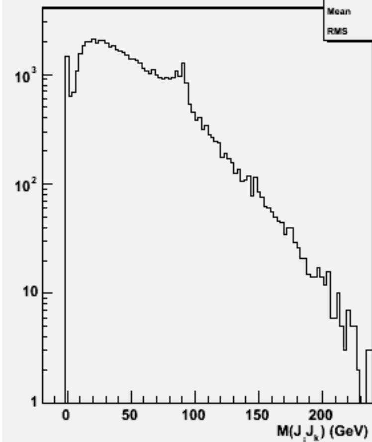
2jets mass(All comb)w102021 n2n2uue3e3_o
