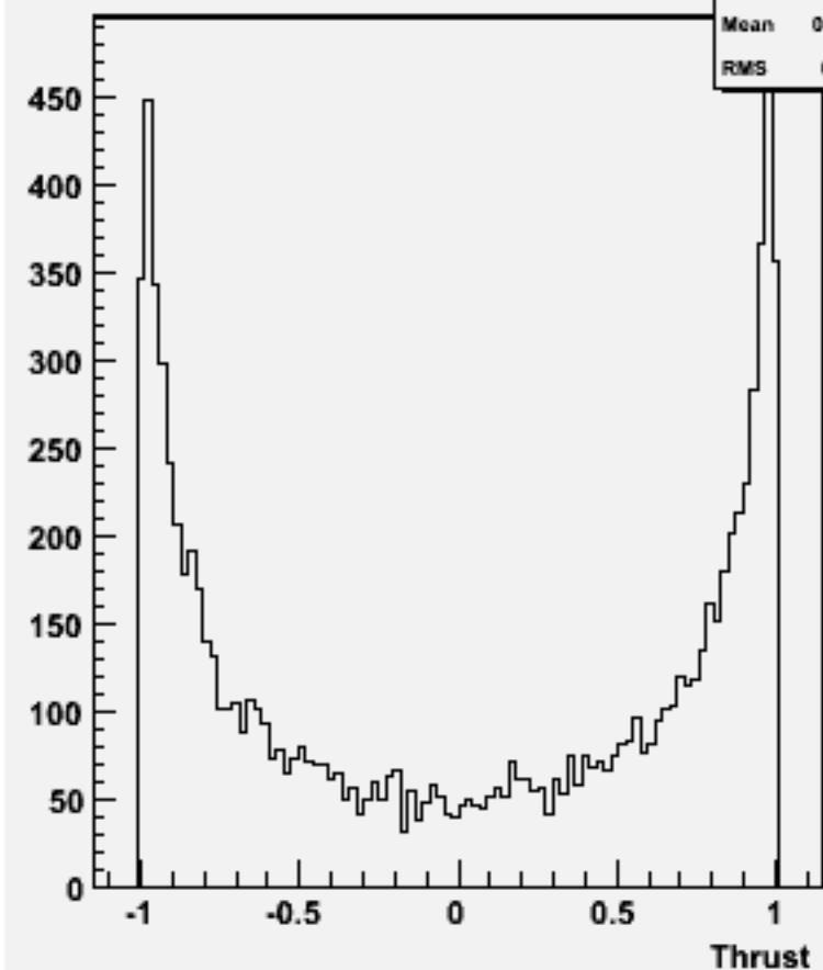
cos \Theta (thrust) w102021 n2n2uue3e3_o
