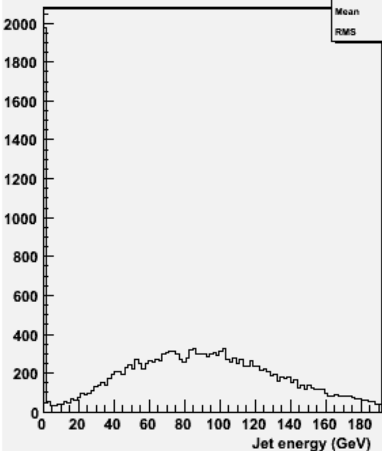
energy for 2-jets :w102021 n2n2uue3e3_o
