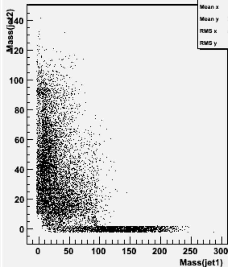
Jet mass for forced 2-jets : w102021 n2n2uue3e3_o
