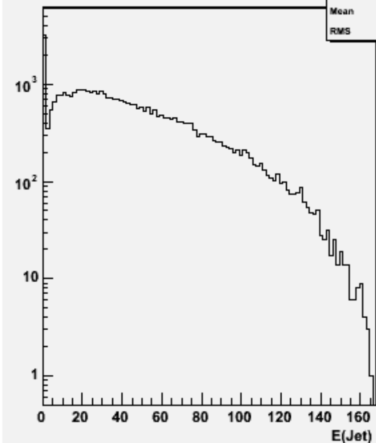
Jet energies(All jets)w102021 n2n2uue3e3_o
