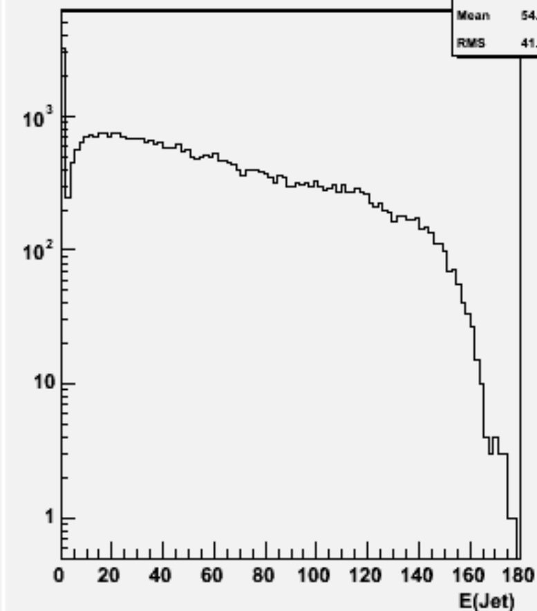
Jet energies(All jets)w102018 n2n2uue1e1_o
