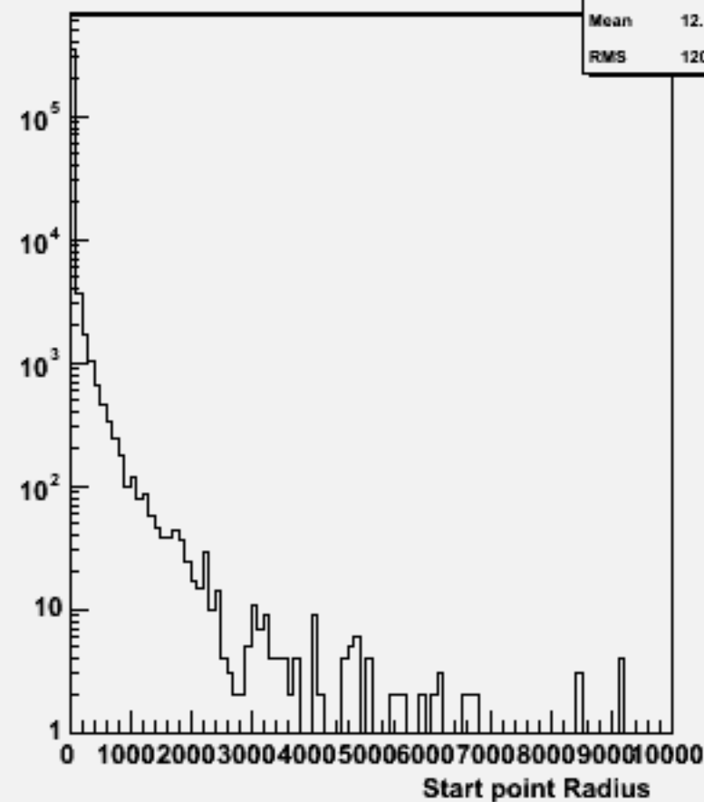
Start point R : w102018 n2n2uue1e1_o
