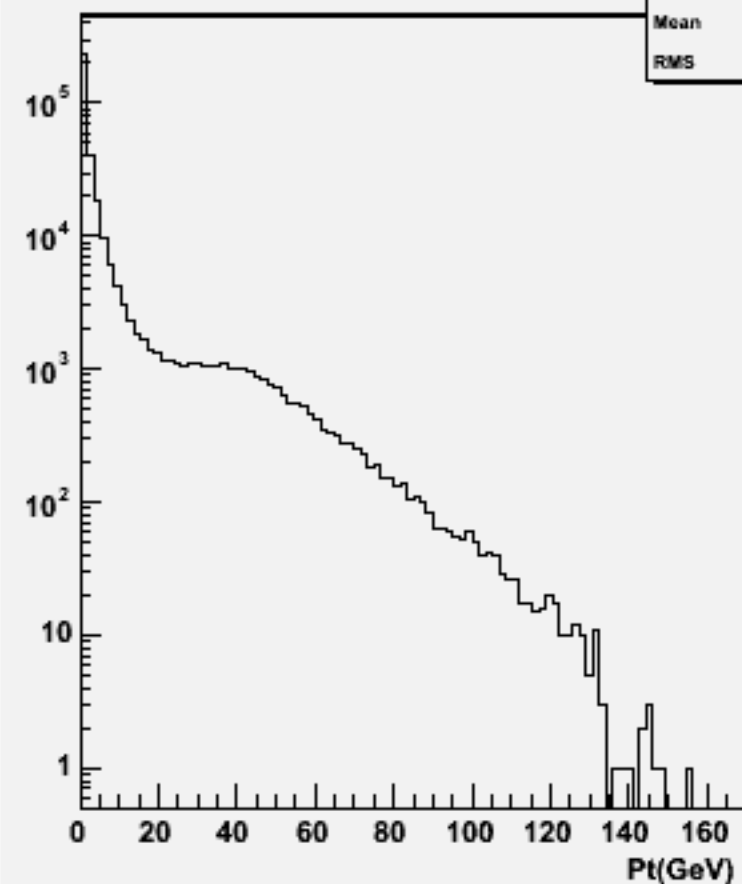
Start point Z : w102018 n2n2uue1e1_o
