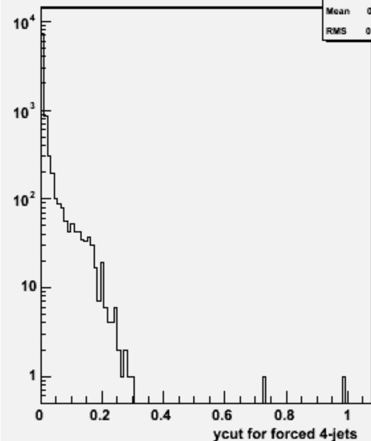
Ycut for 4-jets :w102018 n2n2uue1e1_o
