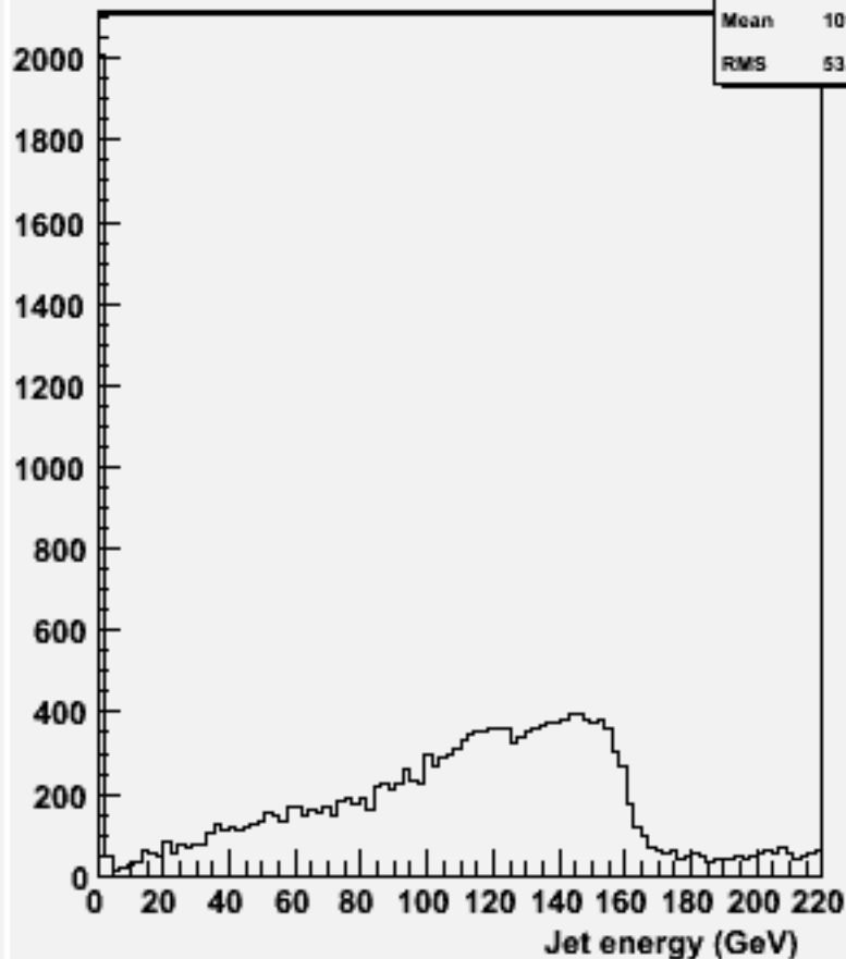
energy for 2-jets :w102018 n2n2uue1e1_o
