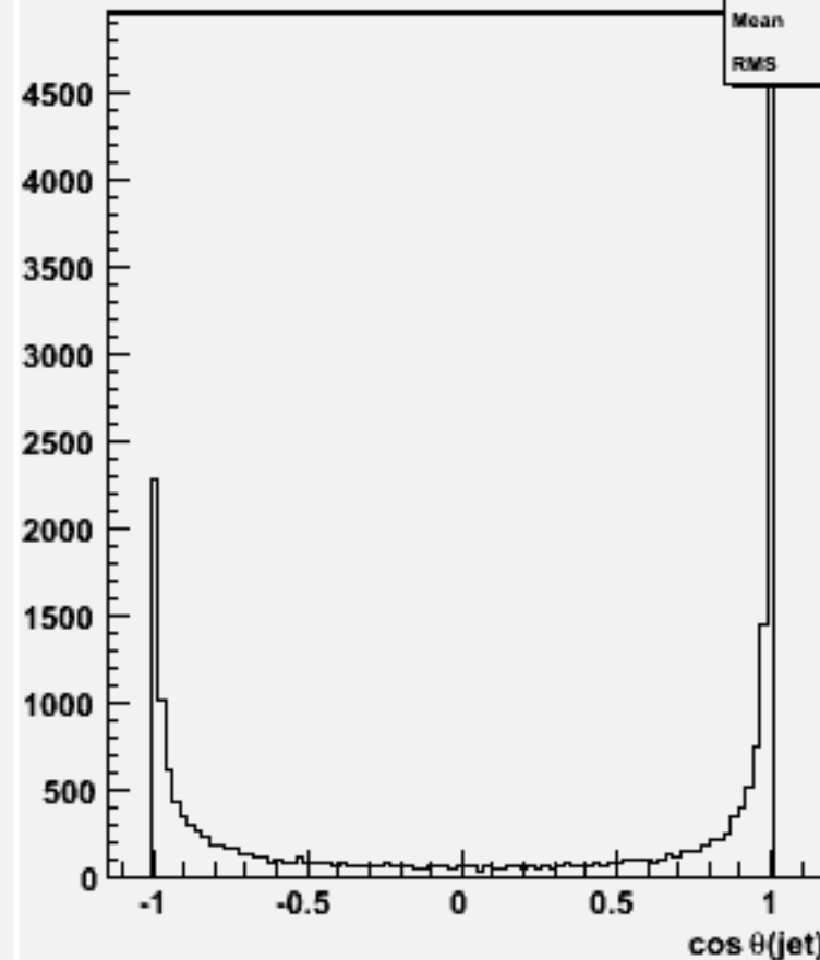
cos \theta for 2-jets :w102018 n2n2uue1e1_o
