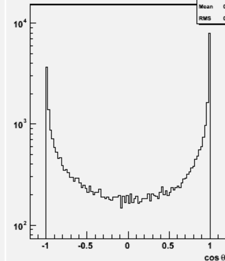
Jet cos \theta (All jets)w102018 n2n2uue1e1_o
