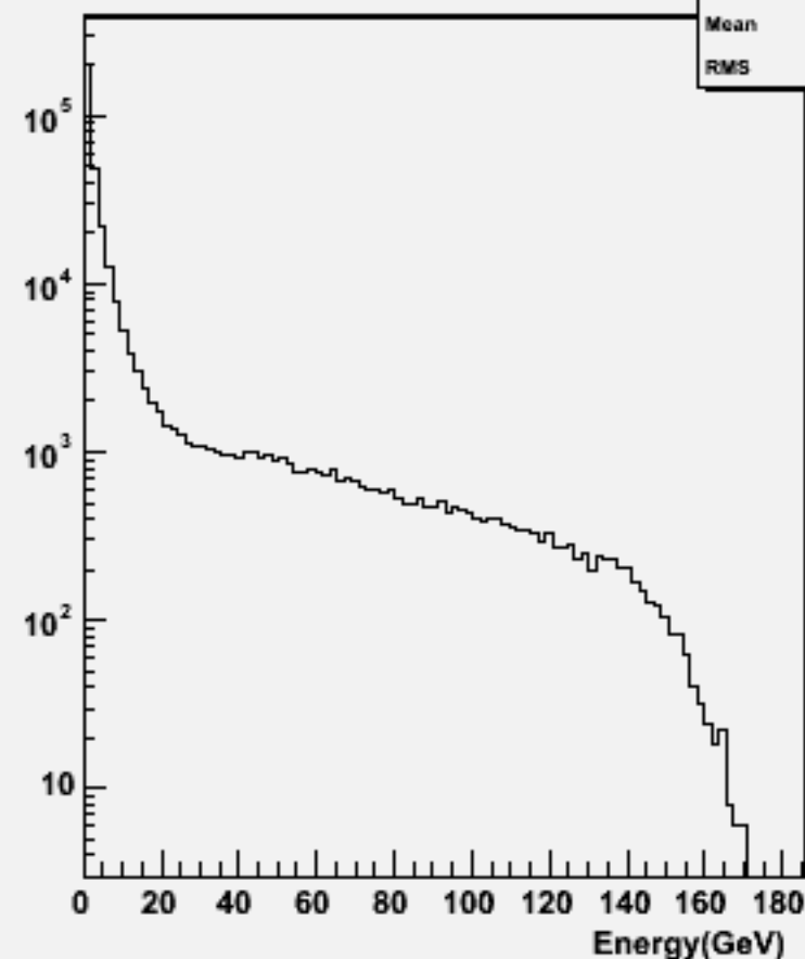
Start point R : w102018 n2n2uue1e1_o
