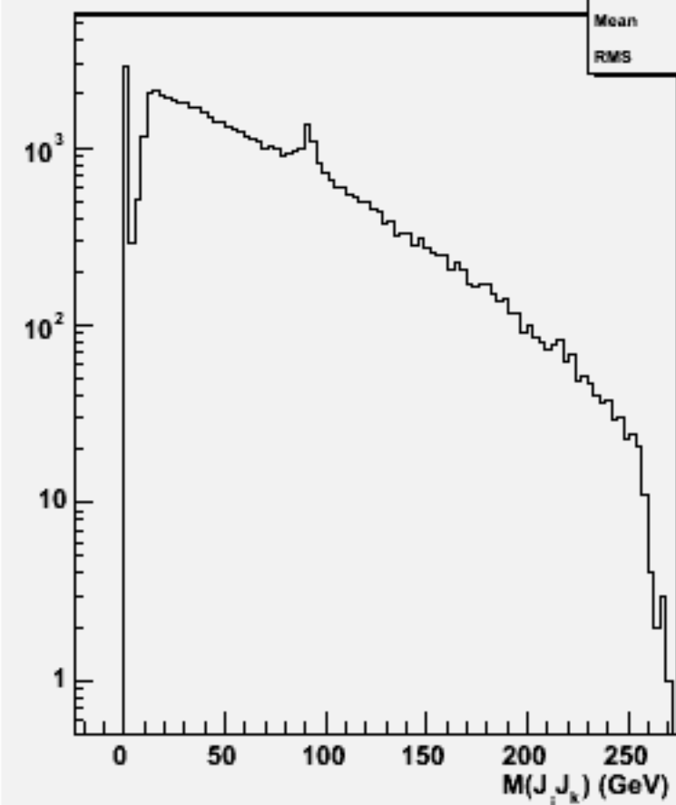
2jets mass(All comb)w102018 n2n2uue1e1_o
