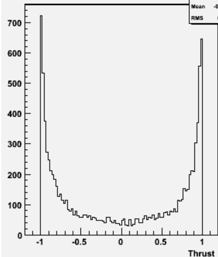
cos \Theta (thrust) w102017 n2n2uue1e1_o
