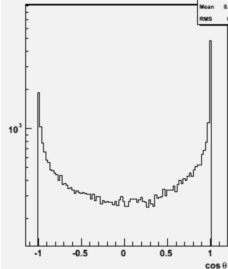
Jet cos \theta (All jets)w102017 n2n2uue1e1_o
