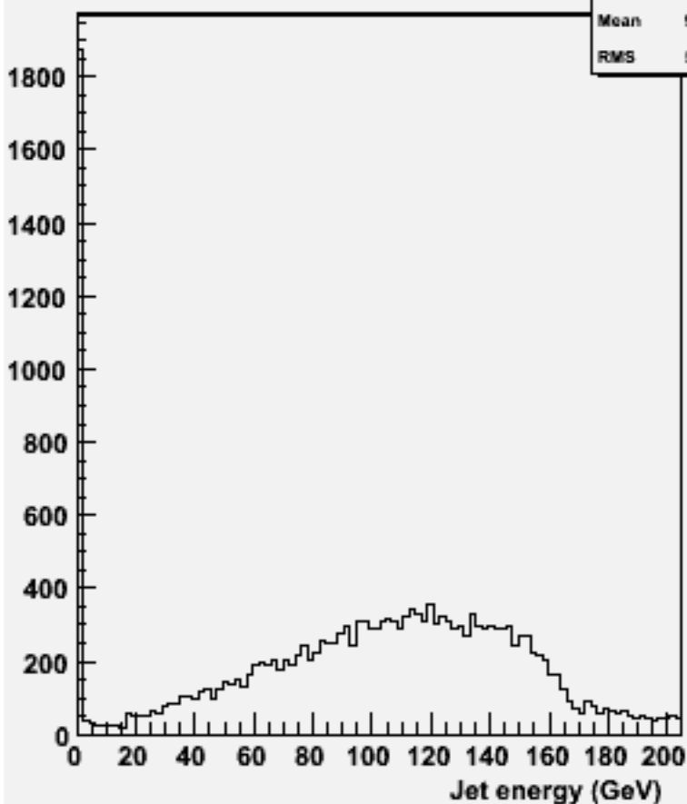
energy for 2-jets :w102017 n2n2uue1e1_o
