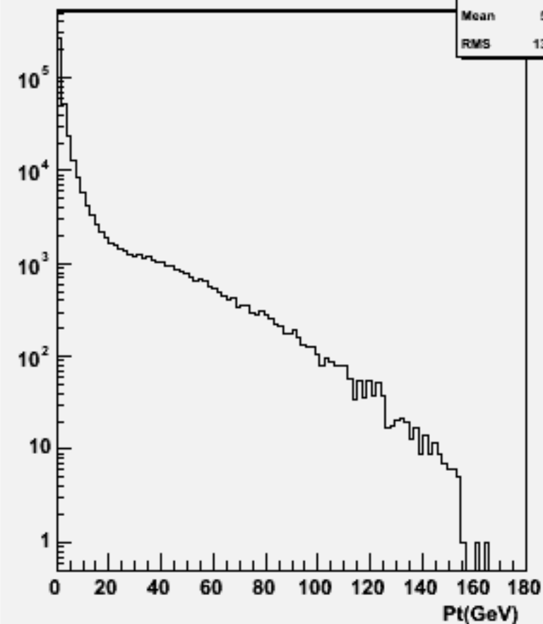
Start point Z : w102017 n2n2uue1e1_o
