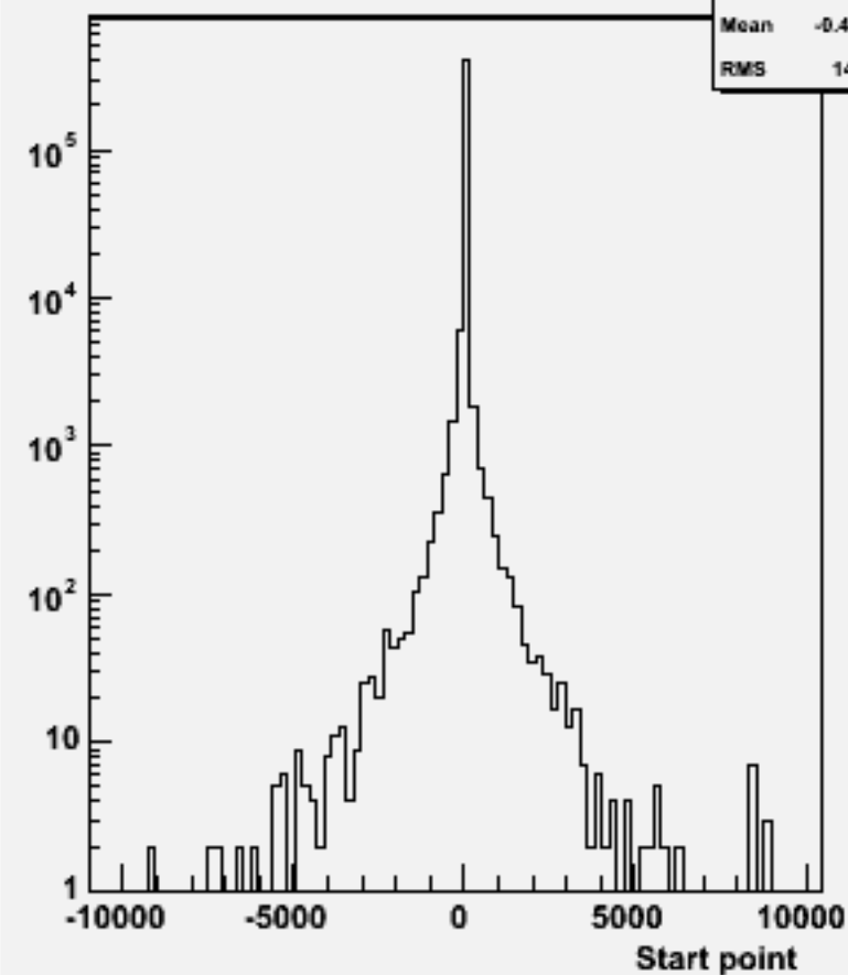
Start point Z : w102017 n2n2uue1e1_o
