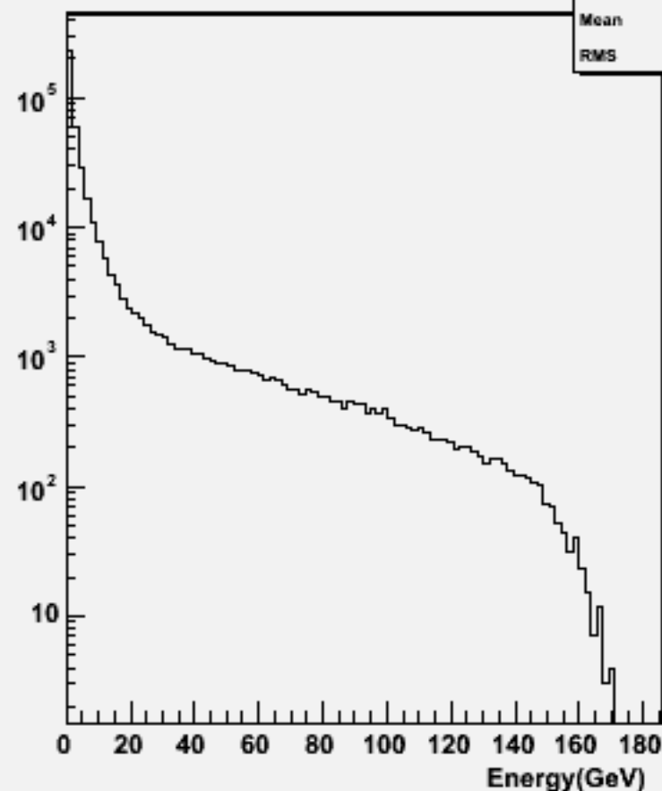
Start point R : w102017 n2n2uue1e1_o
