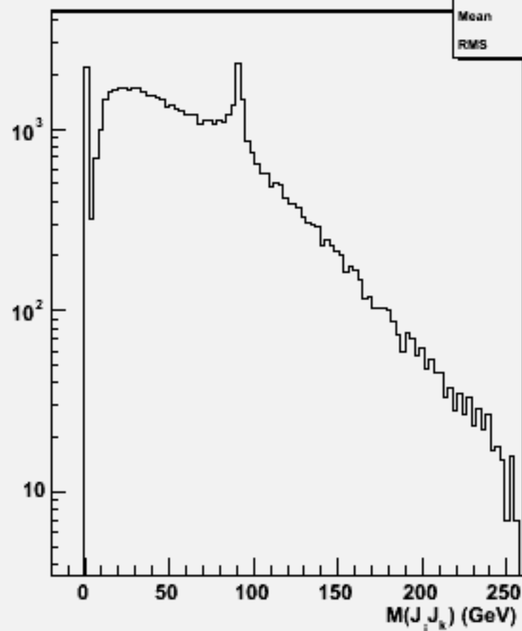
2jets mass(All comb)w102017 n2n2uue1e1_o
