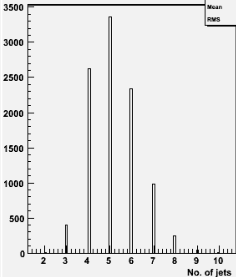
No. jets (ycut=0.001) : w102017 n2n2uue1e1_o
