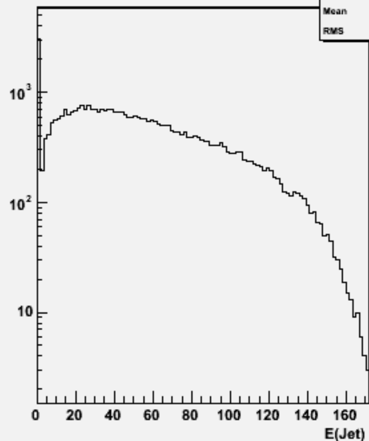
Jet energies(All jets)w102017 n2n2uue1e1_o
