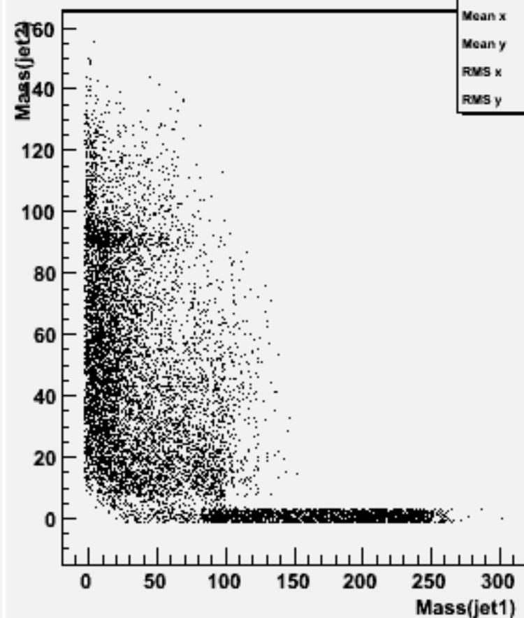
Jet mass for forced 2-jets : w102017 n2n2uue1e1_o
