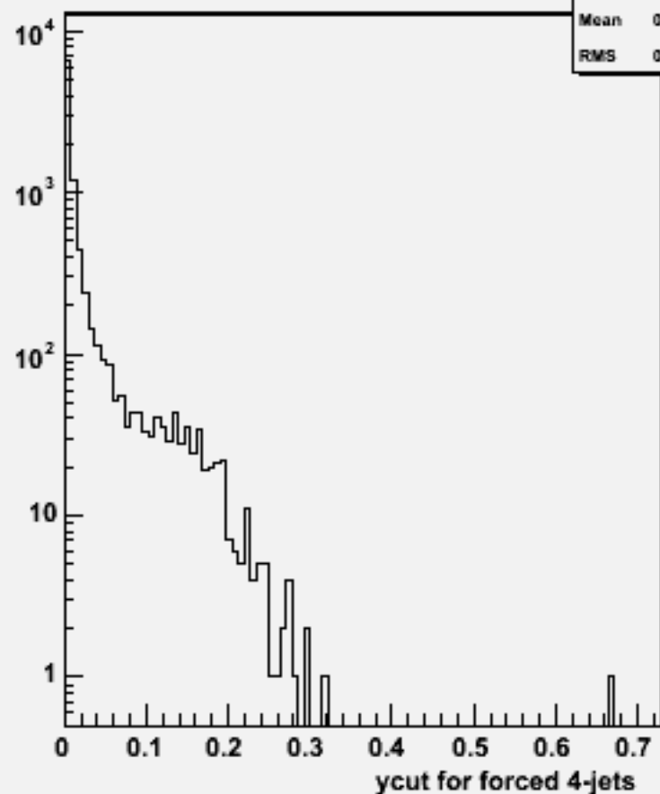
Ycut for 4-jets :w102017 n2n2uue1e1_o
