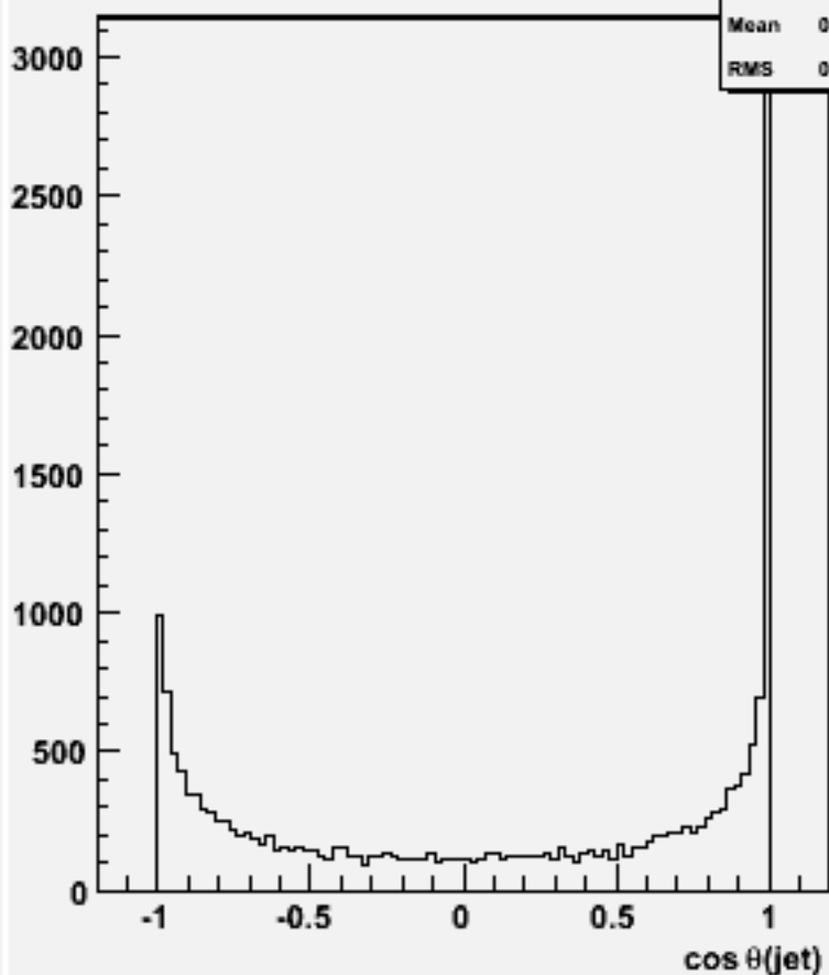
cos \theta for 2-jets :w102017 n2n2uue1e1_o
