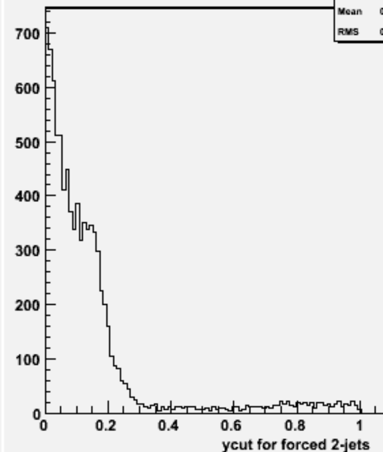
Ycut for 2-jets :w102017 n2n2uue1e1_o
