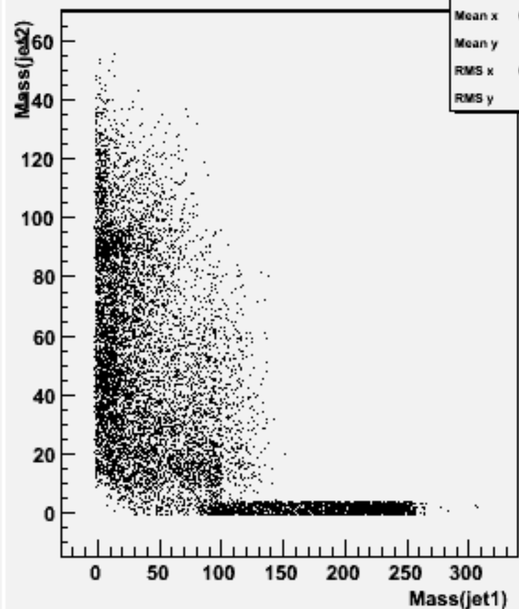
Jet mass for forced 2-jets : w102016 n2n2uue1e1_o
