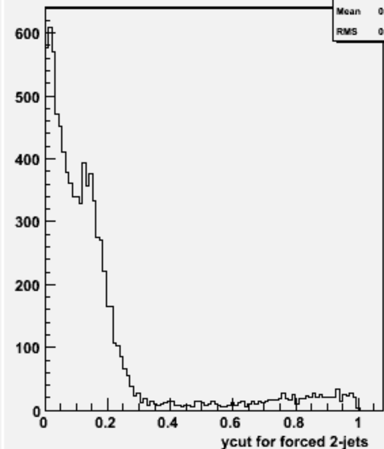
Ycut for 2-jets :w102016 n2n2uue1e1_o
