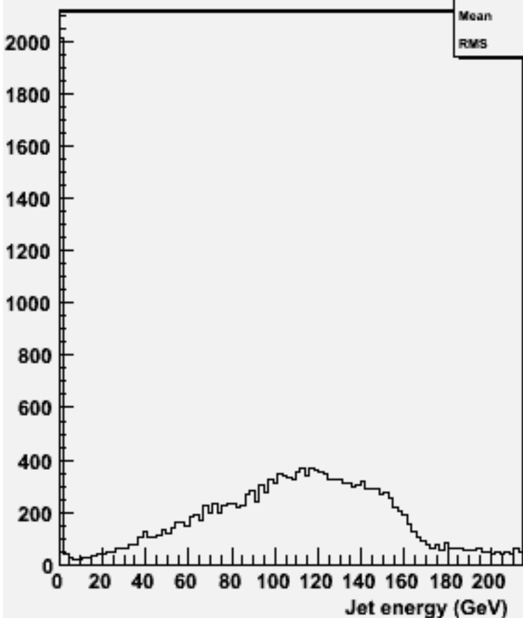
energy for 2-jets :w102016 n2n2uue1e1_o
