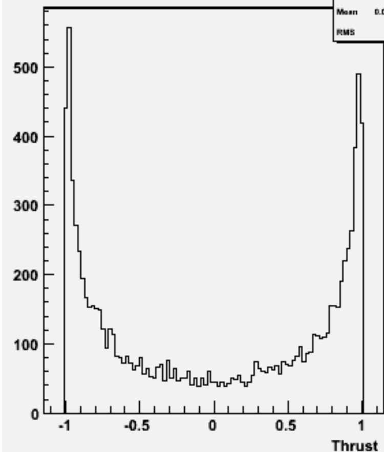
cos \Theta (thrust) w102016 n2n2uue1e1_o
