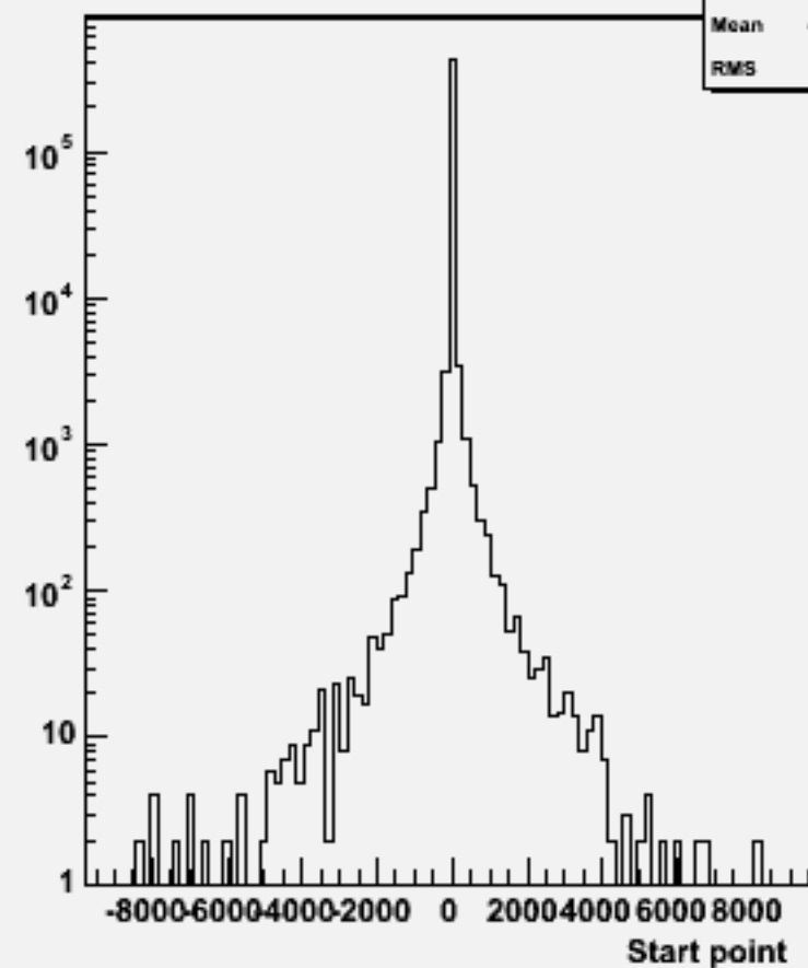
Start point Z : w102016 n2n2uue1e1_o
