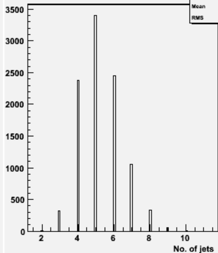
No. jets (ycut=0.001) : w102016 n2n2uue1e1_o
