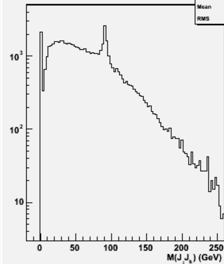
2jets mass(All comb)w102016 n2n2uue1e1_o
