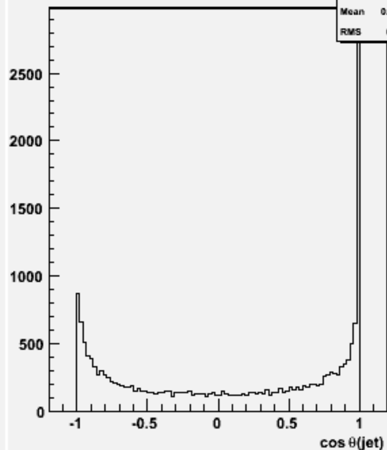
cos \theta for 2-jets :w102016 n2n2uue1e1_o
