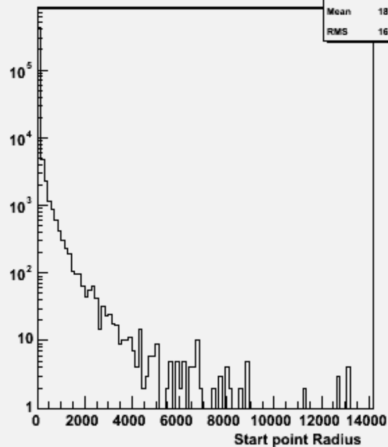
Start point R : w102016 n2n2uue1e1_o
