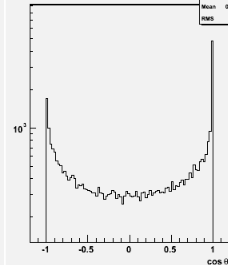
Jet cos \theta (All jets)w102016 n2n2uue1e1_o
