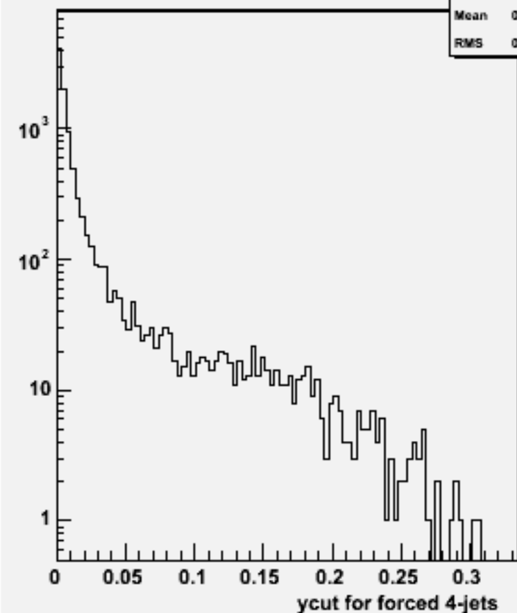
Ycut for 4-jets :w102016 n2n2uue1e1_o
