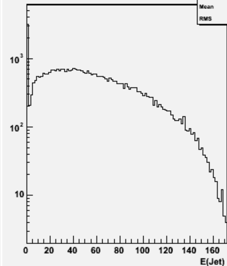
Jet energies(All jets)w102016 n2n2uue1e1_o
