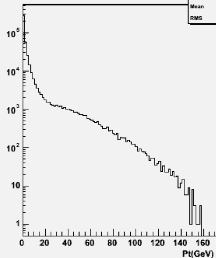
Start point Z : w102016 n2n2uue1e1_o
