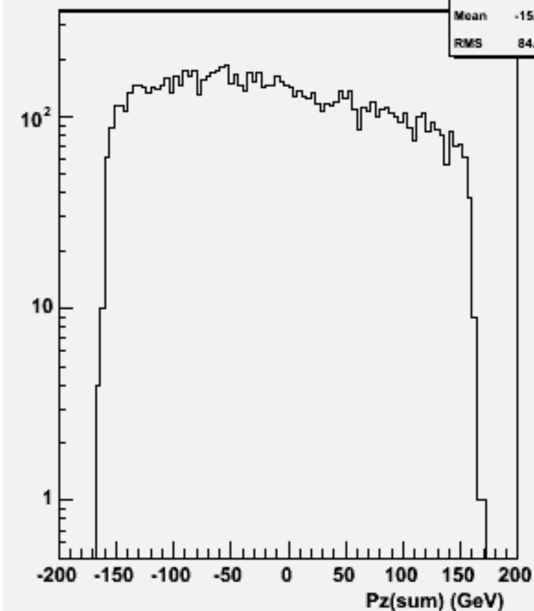
Pz Sum: w102015 n2n2uue1e1_o
