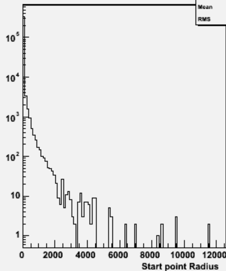
Start point R : w102015 n2n2uue1e1_o
