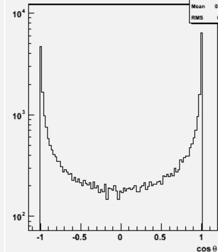
Jet cos \theta (All jets)w102015 n2n2uue1e1_o
