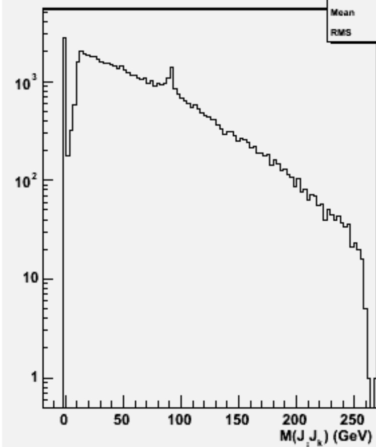
2jets mass(All comb)w102015 n2n2uue1e1_o
