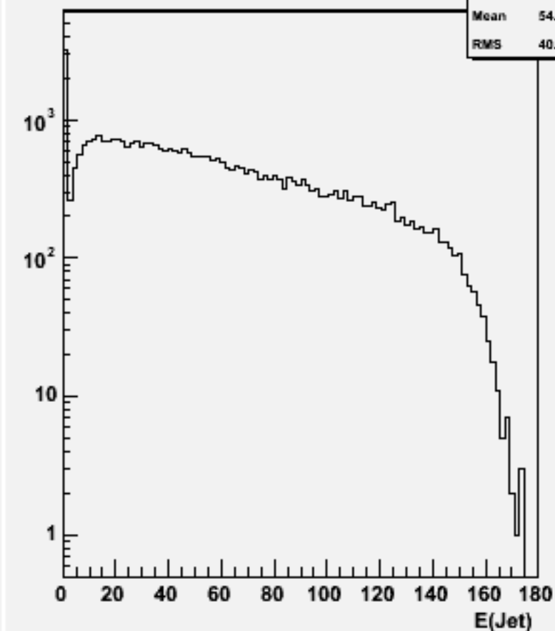
Jet energies(All jets)w102015 n2n2uue1e1_o
