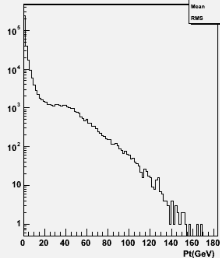
Start point Z : w102015 n2n2uue1e1_o
