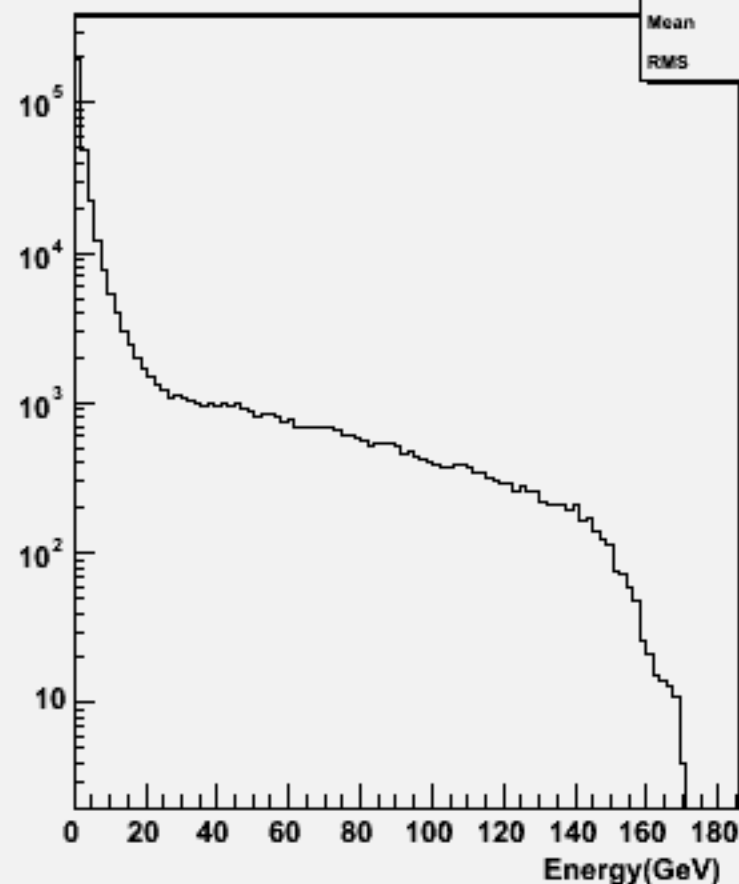
Start point R : w102015 n2n2uue1e1_o
