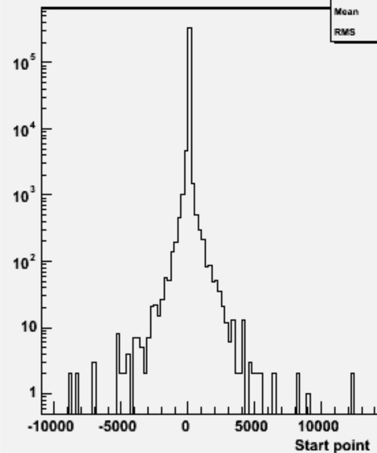
Start point Z : w102015 n2n2uue1e1_o
