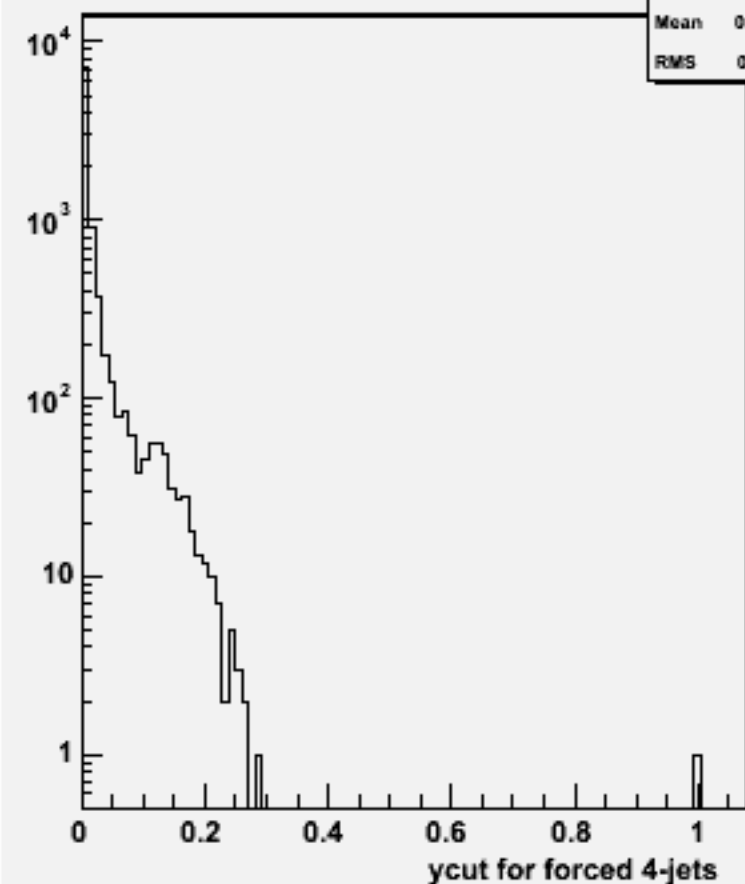
Ycut for 4-jets :w102015 n2n2uue1e1_o
