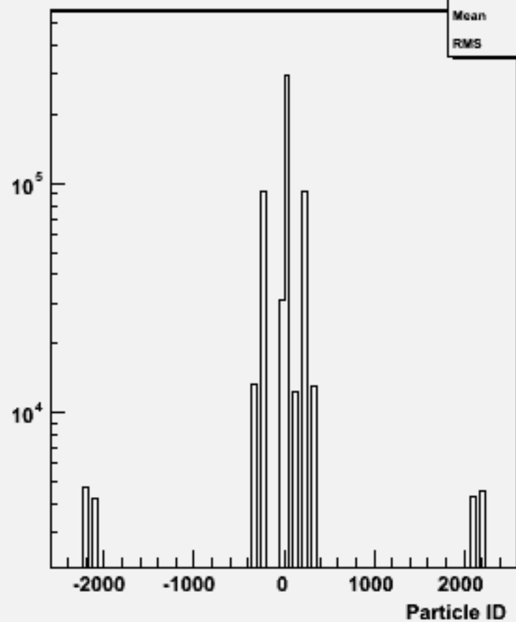
Particle ID : w102013 n2n2n3n3bb_o
