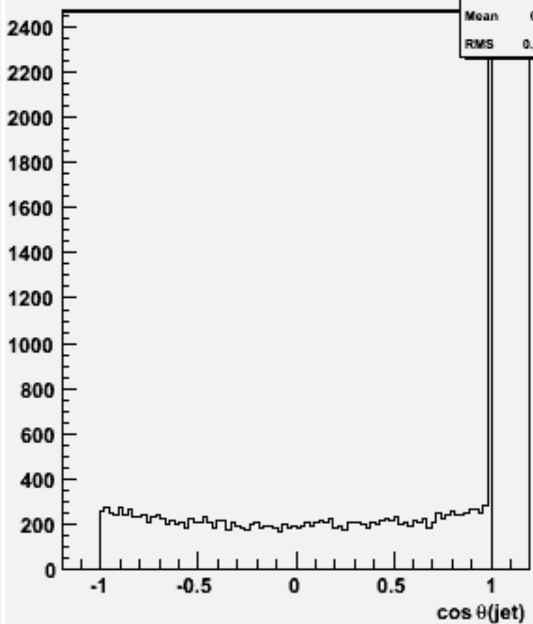
cos \theta for 2-jets :w102013 n2n2n3n3bb_o
