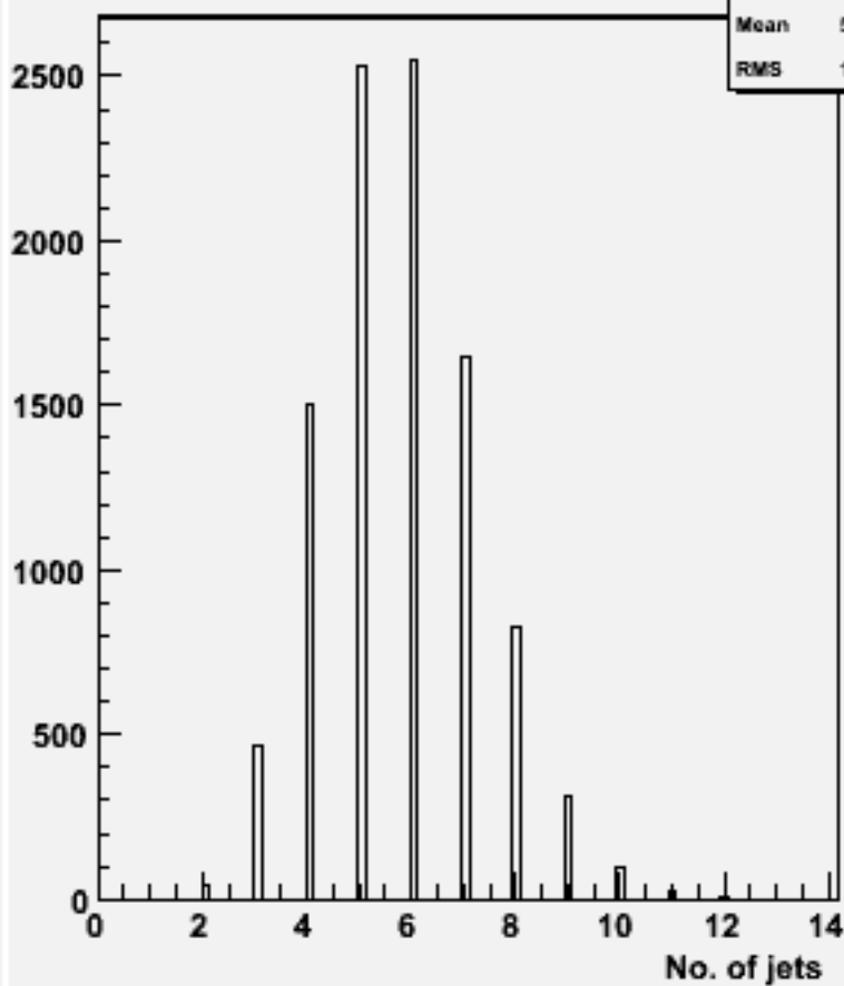
No. jets (ycut=0.001) : w102013 n2n2n3n3bb_o
