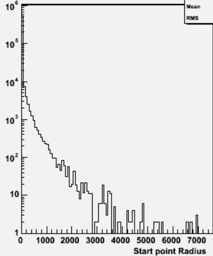
Start point R : w102013 n2n2n3n3bb_o
