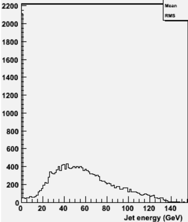
energy for 2-jets :w102013 n2n2n3n3bb_o
