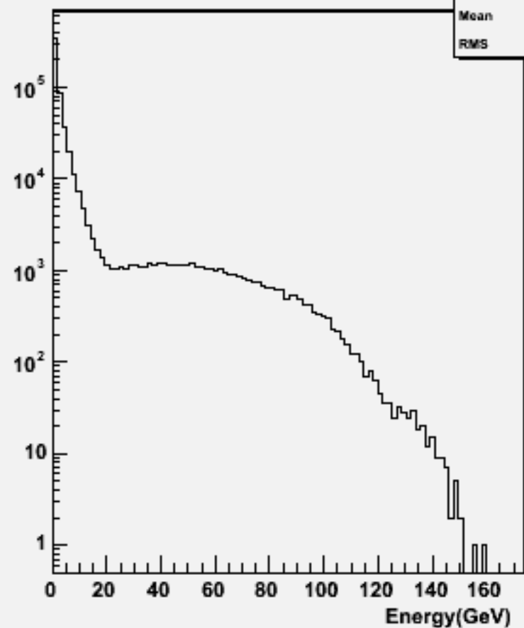
Particle Energy : w102013 n2n2n3n3bb_o
