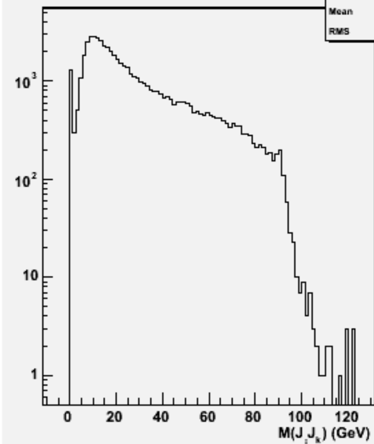
2jets mass(All comb)w102013 n2n2n3n3bb_o
