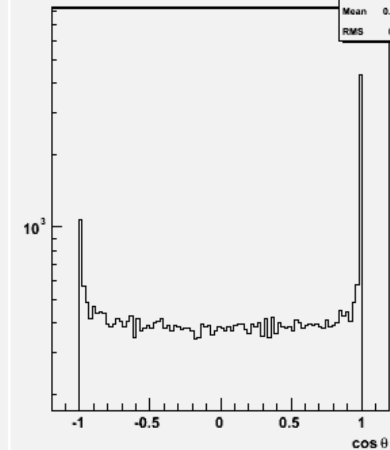
Jet cos \theta (All jets)w102013 n2n2n3n3bb_o
