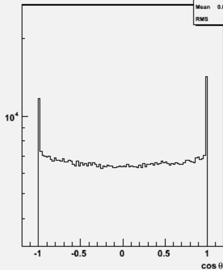
Particle cosθ : w102013 n2n2n3n3bb_o
