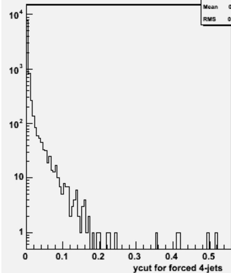
Ycut for 4-jets :w102013 n2n2n3n3bb_o
