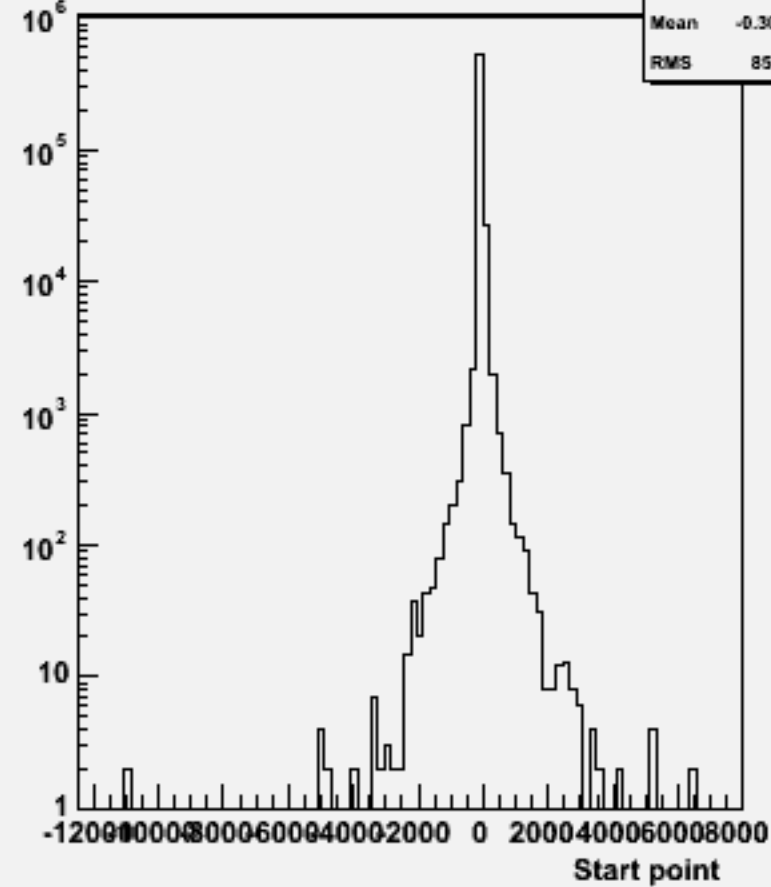
Start point Z : w102013 n2n2n3n3bb_o
