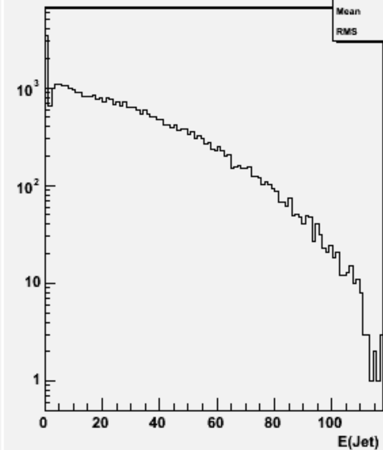
Jet energies(All jets)w102013 n2n2n3n3bb_o
