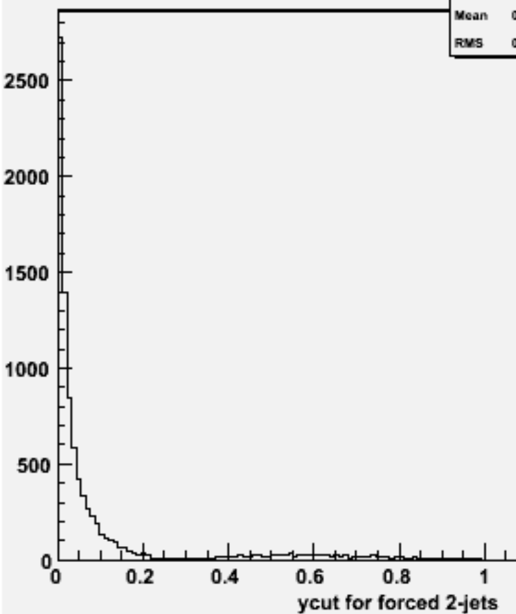
Ycut for 2-jets :w102013 n2n2n3n3bb_o
