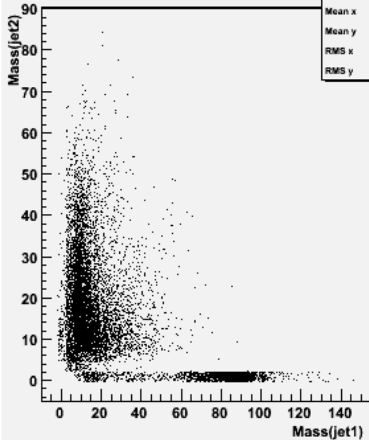
Jet mass for forced 2-jets : w102013 n2n2n3n3bb_o
