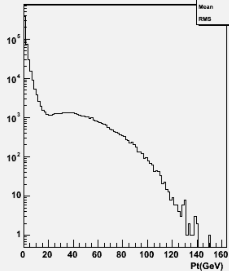
Particle Pt : w102013 n2n2n3n3bb_o
