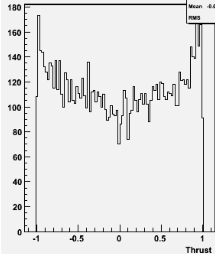
cos \Theta (thrust) w102013 n2n2n3n3bb_o
