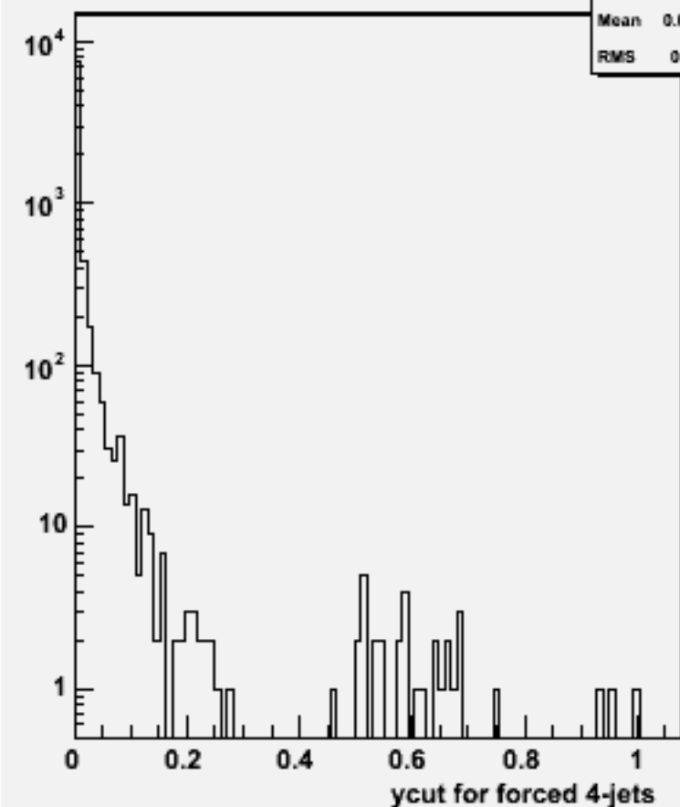
Ycut for 4-jets :w102008 n2n2n3n3ss_o
