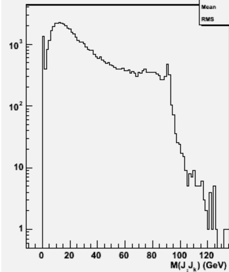
2jets mass(All comb)w102008 n2n2n3n3ss_o
