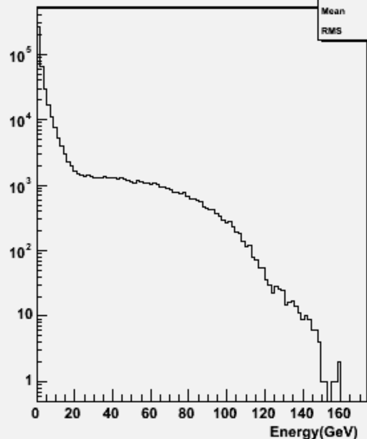
Start point R : w102008 n2n2n3n3ss_o
