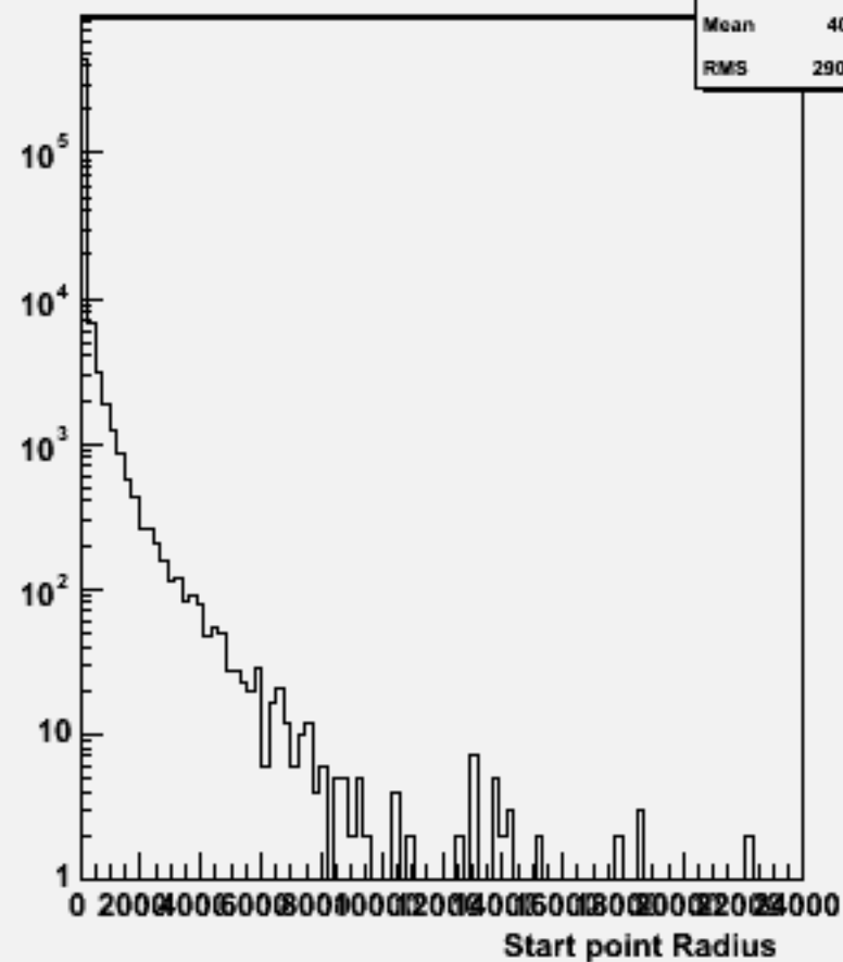
Start point R : w102008 n2n2n3n3ss_o
