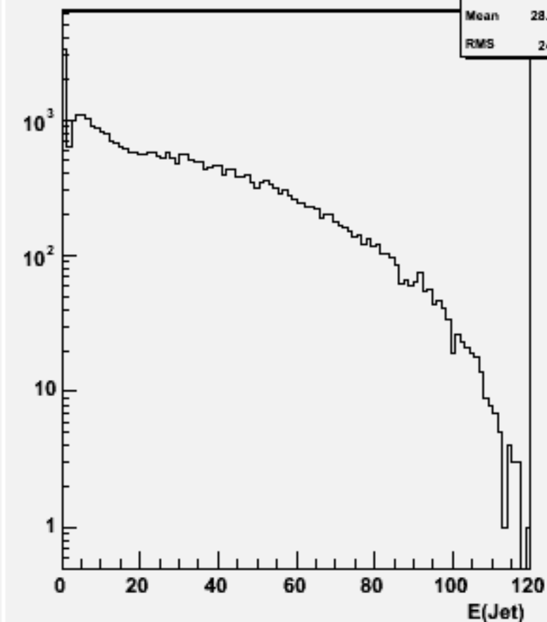
Jet energies(All jets)w102008 n2n2n3n3ss_o
