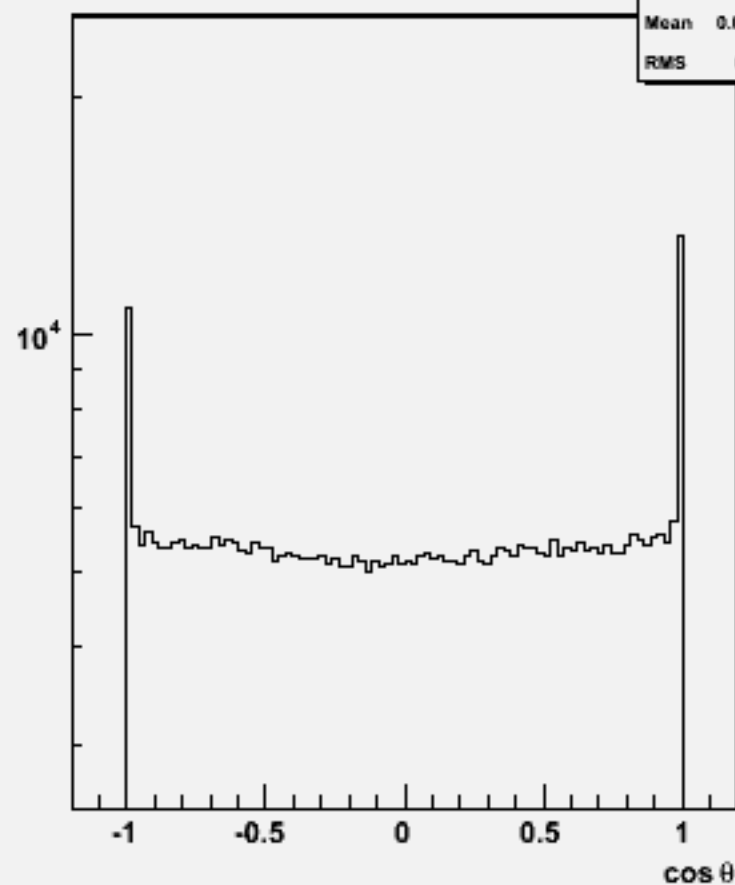
Particle cos θ : w102008 n2n2n3n3ss_o
