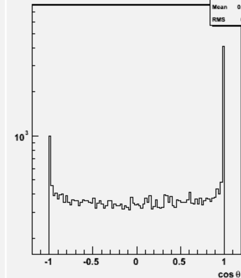
Jet cos \theta (All jets)w102008 n2n2n3n3ss_o
