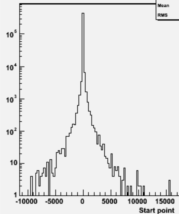
Start point Z : w102008 n2n2n3n3ss_o
