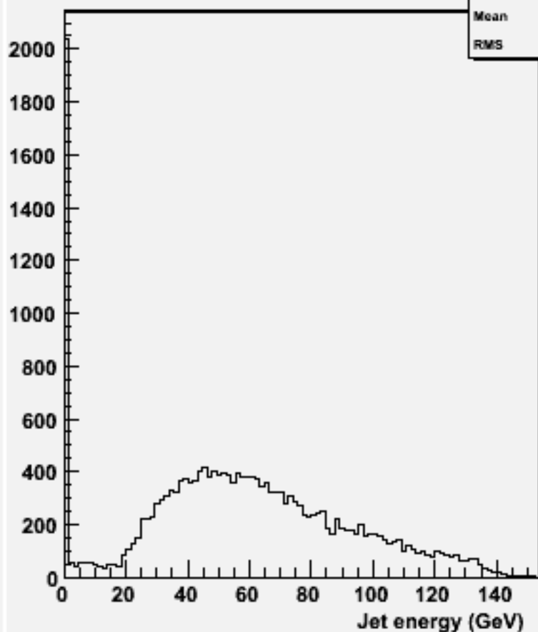
energy for 2-jets :w102008 n2n2n3n3ss_o
