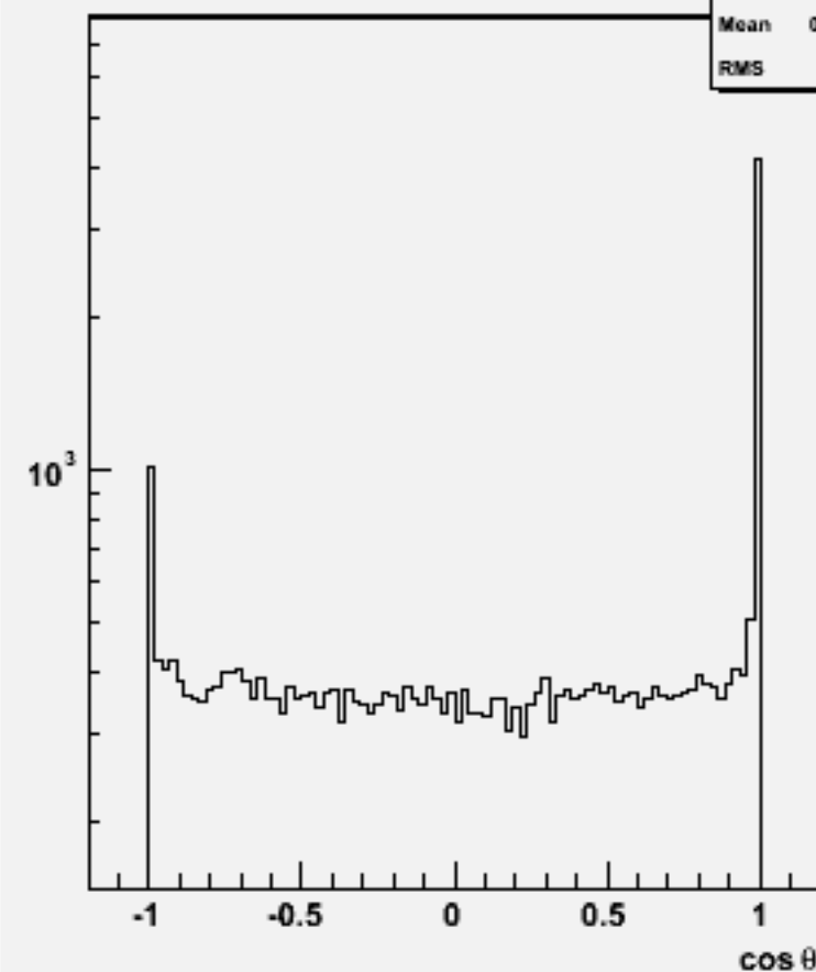
Jet cos \theta (All jets)w102004 n2n2n3n3dd_o
