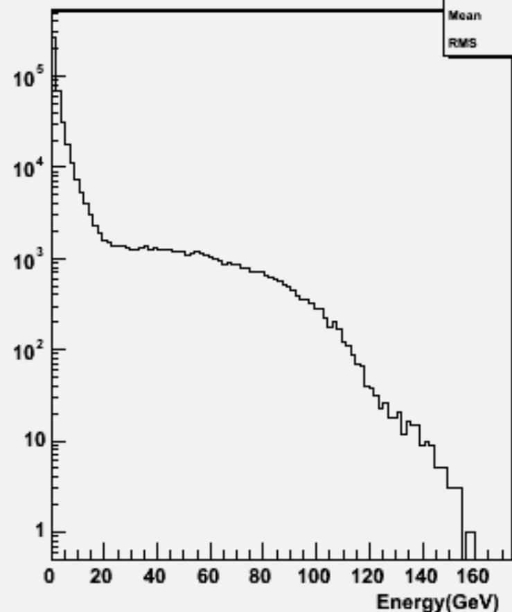
Particle Energy : w102004 n2n2n3n3dd_o
