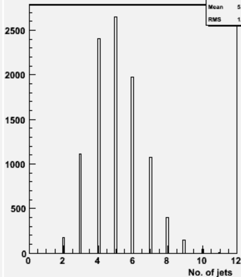
No. jets (ycut=0.001) : w102004 n2n2n3n3dd_o
