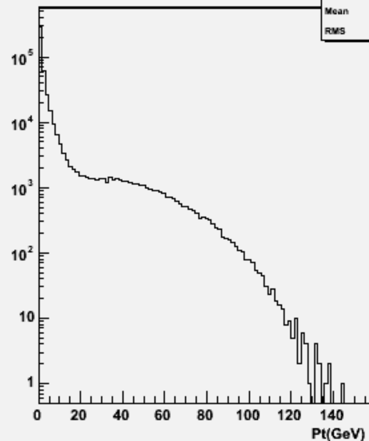
Particle Pt : w102004 n2n2n3n3dd_o
