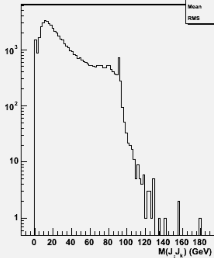
2jets mass(All comb)w102004 n2n2n3n3dd_o
