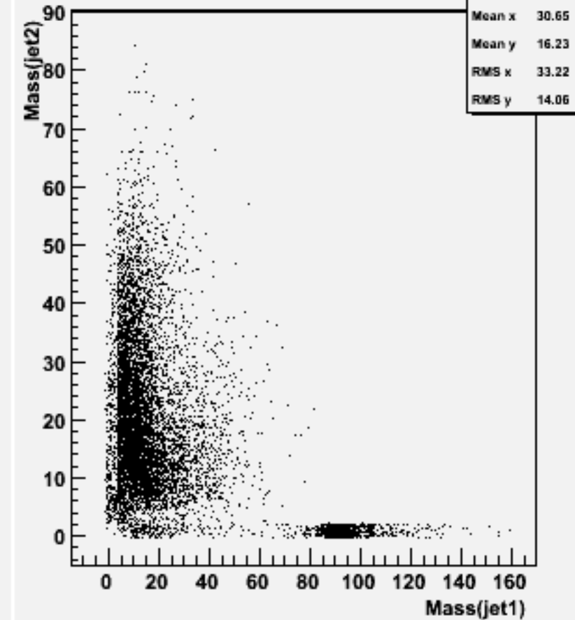
Jet mass for forced 2-jets : w102004 n2n2n3n3dd_o
