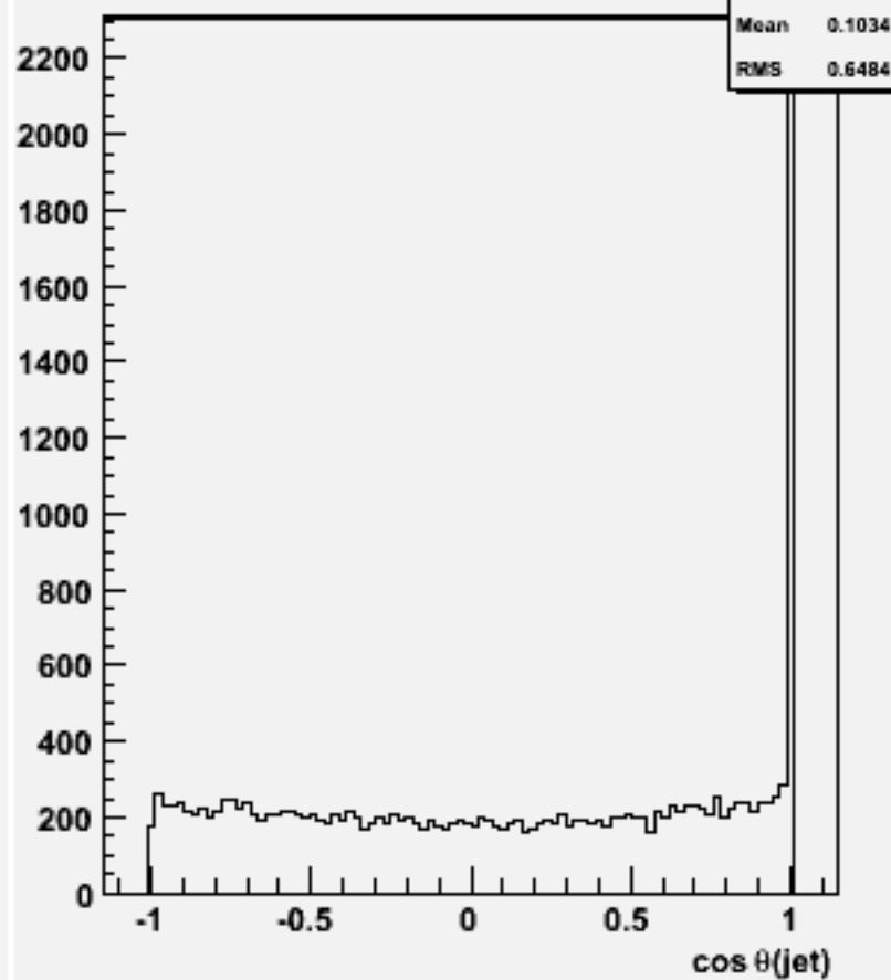
cos \theta for 2-jets :w102004 n2n2n3n3dd_o
