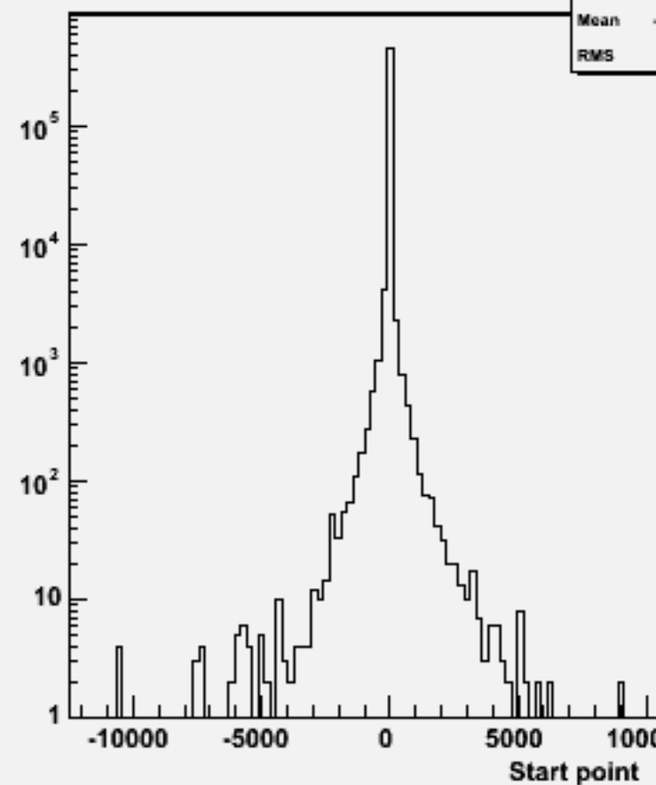
Start point Z : w102004 n2n2n3n3dd_o
