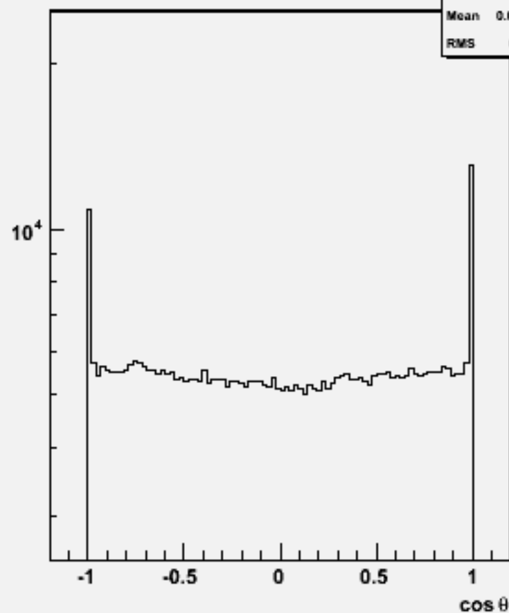
Particle cos θ : w102004 n2n2n3n3dd_o
