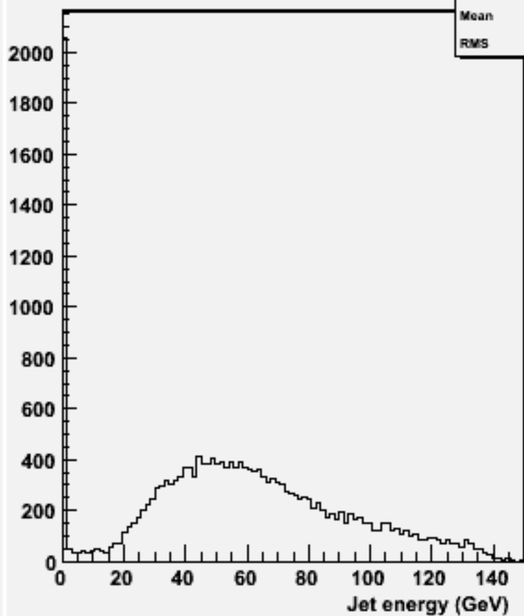
energy for 2-jets :w102004 n2n2n3n3dd_o
