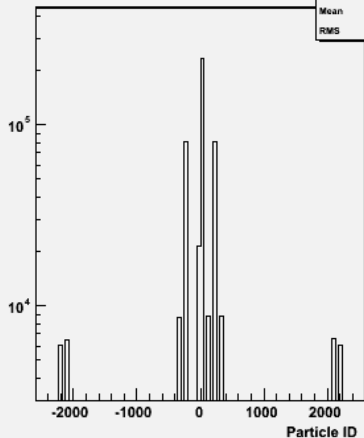
Particle ID : w102004 n2n2n3n3dd_o
