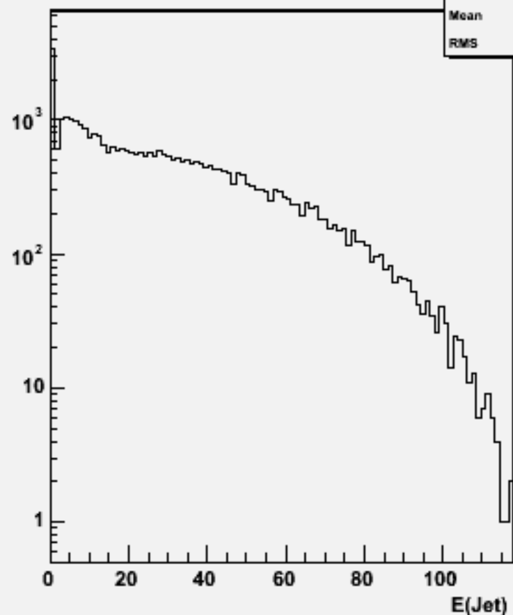
Jet energies(All jets)w102004 n2n2n3n3dd_o
