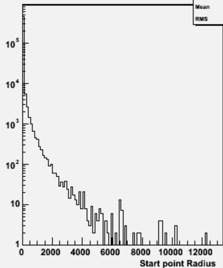
Start point R : w102004 n2n2n3n3dd_o
