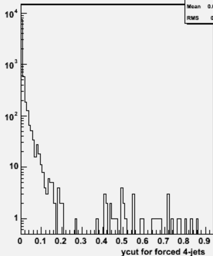
Ycut for 4-jets :w102004 n2n2n3n3dd_o
