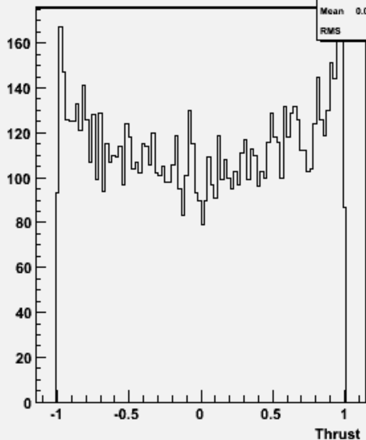
cos \Theta (thrust) w102004 n2n2n3n3dd_o
