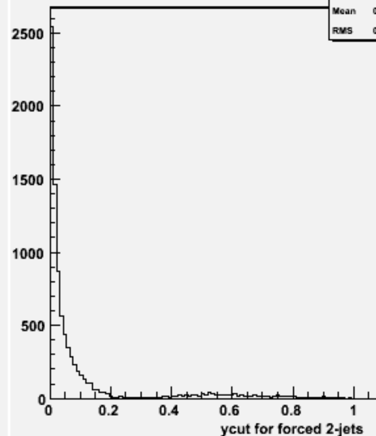
Ycut for 2-jets :w102004 n2n2n3n3dd_o
