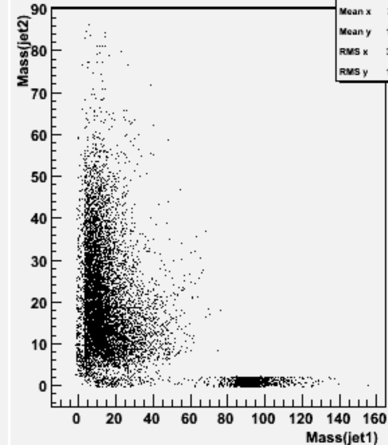
Jet mass for forced 2-jets : w101992 n2n2n2n2ss_o
