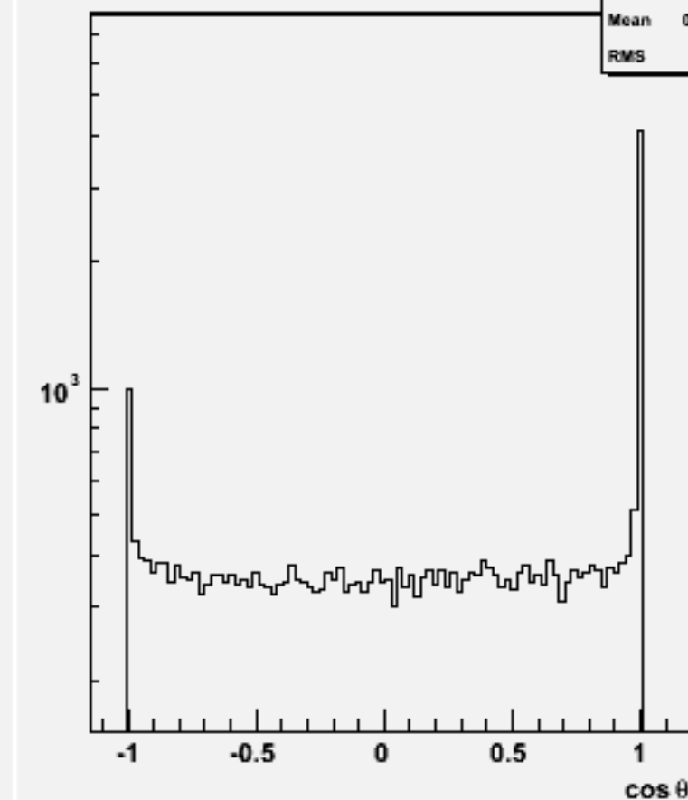
Jet cos \theta (All jets)w101992 n2n2n2n2ss_o
