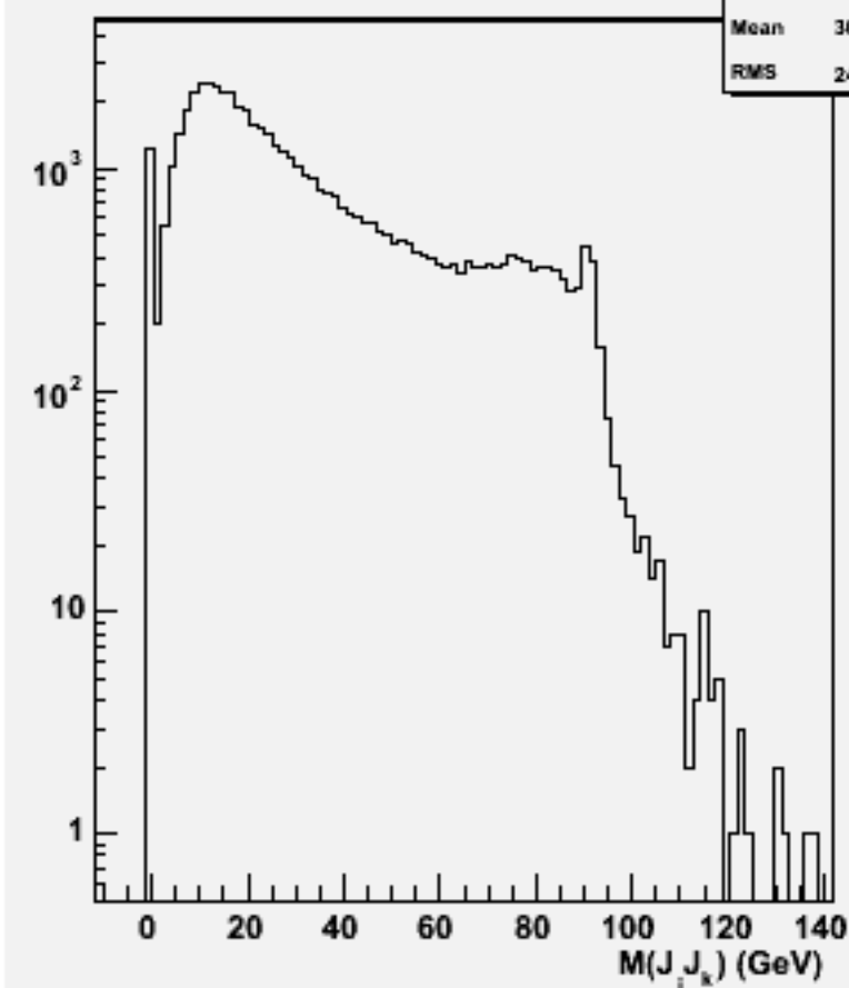
2jets mass(All comb)w101992 n2n2n2n2ss_o
