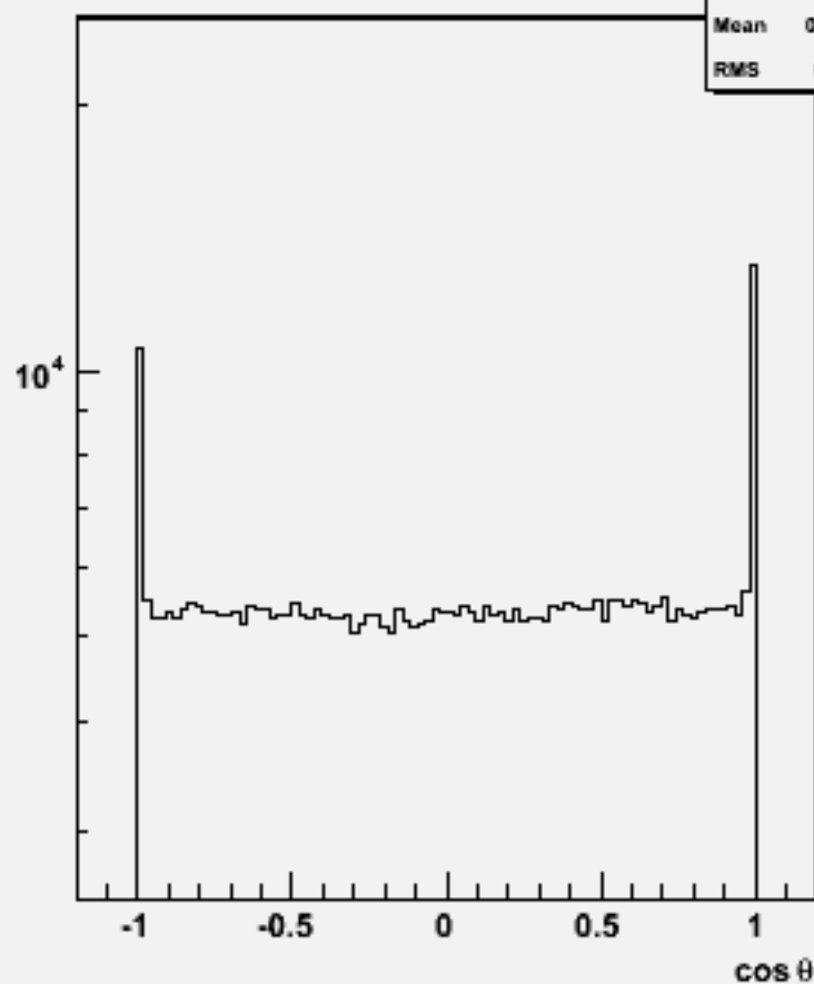
Particle cosθ : w101992 n2n2n2n2ss_o
