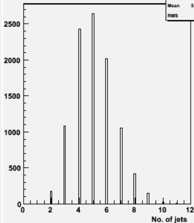
No. jets (ycut=0.001) : w101992 n2n2n2n2ss_o
