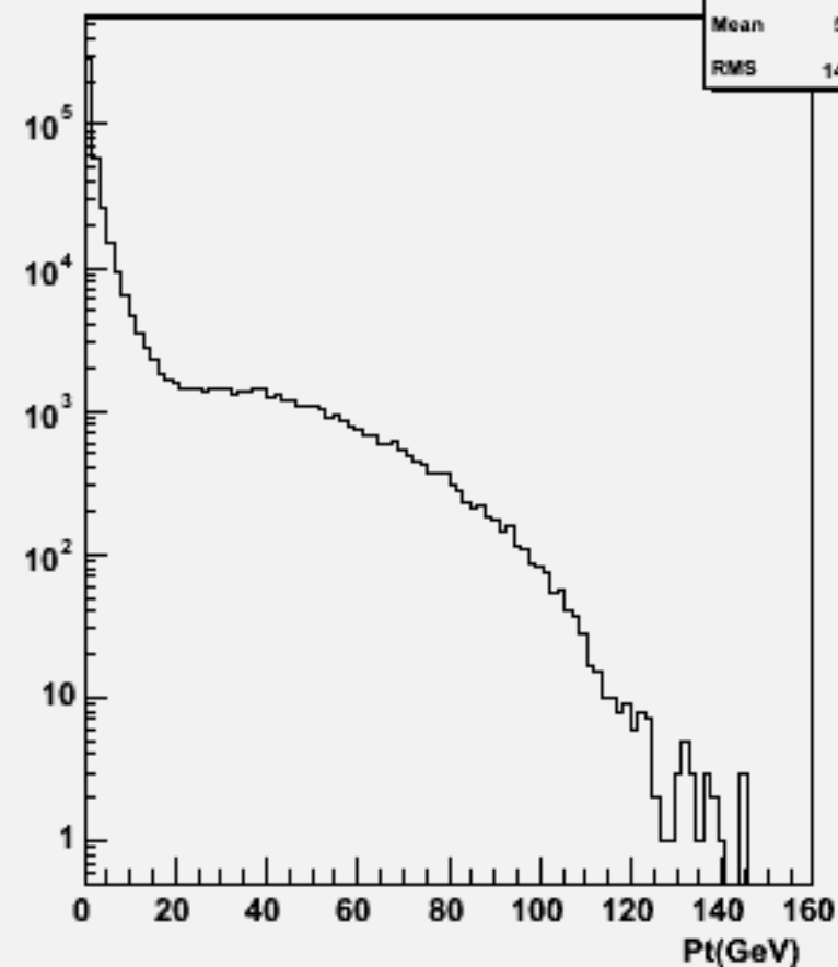
Particle Pt : w101992 n2n2n2n2ss_o
