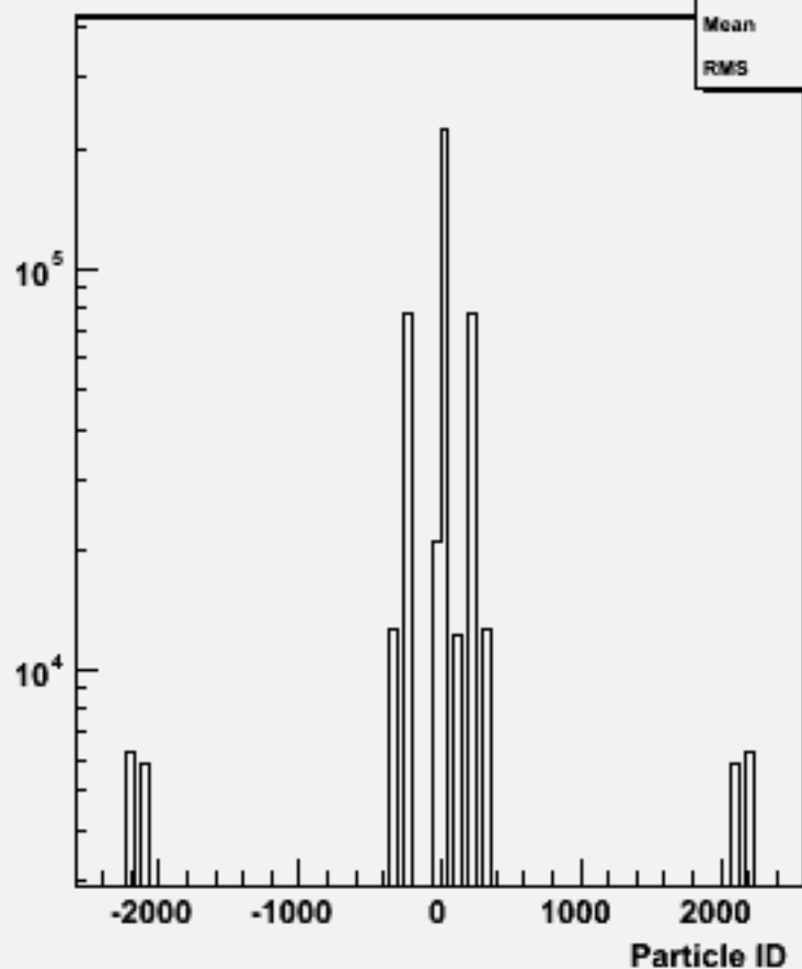
Particle ID : w101992 n2n2n2n2ss_o
