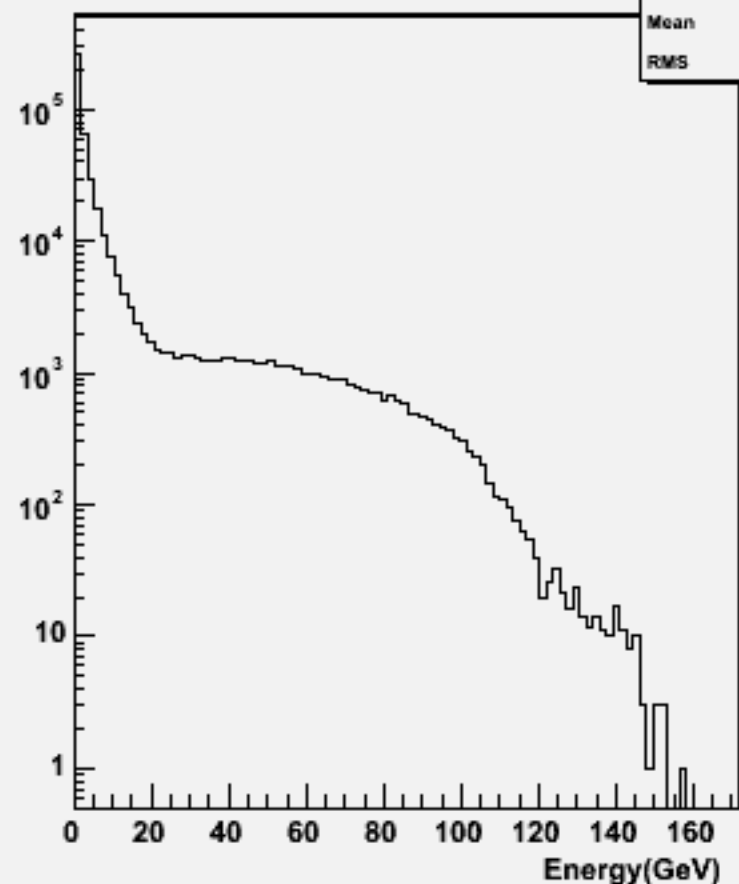
Particle Energy : w101992 n2n2n2n2ss_o
