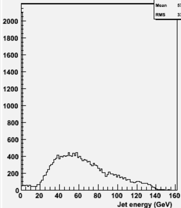
energy for 2-jets :w101992 n2n2n2n2ss_o
