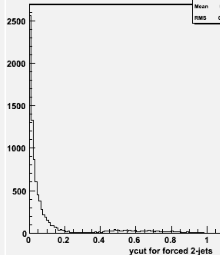
Ycut for 2-jets :w101992 n2n2n2n2ss_o
