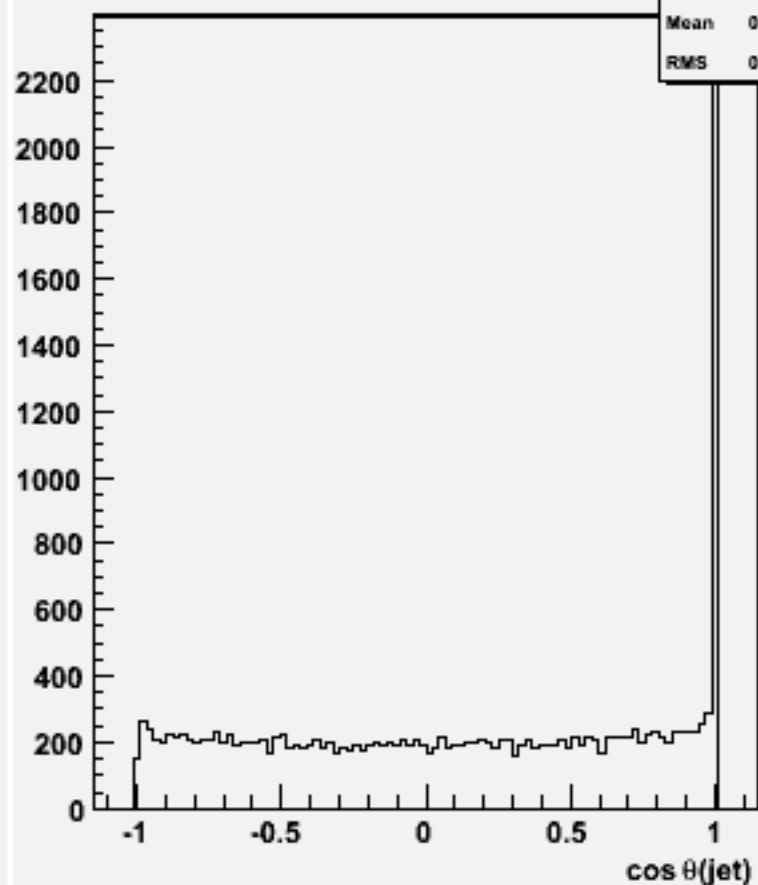
cos \theta for 2-jets :w101992 n2n2n2n2ss_o
