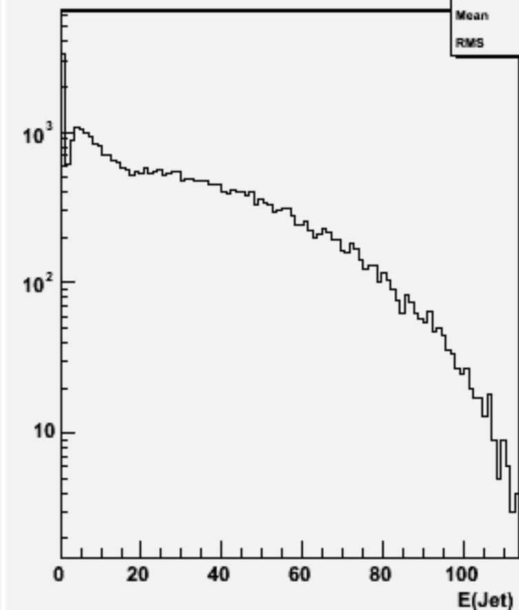
Jet energies(All jets)w101992 n2n2n2n2ss_o
