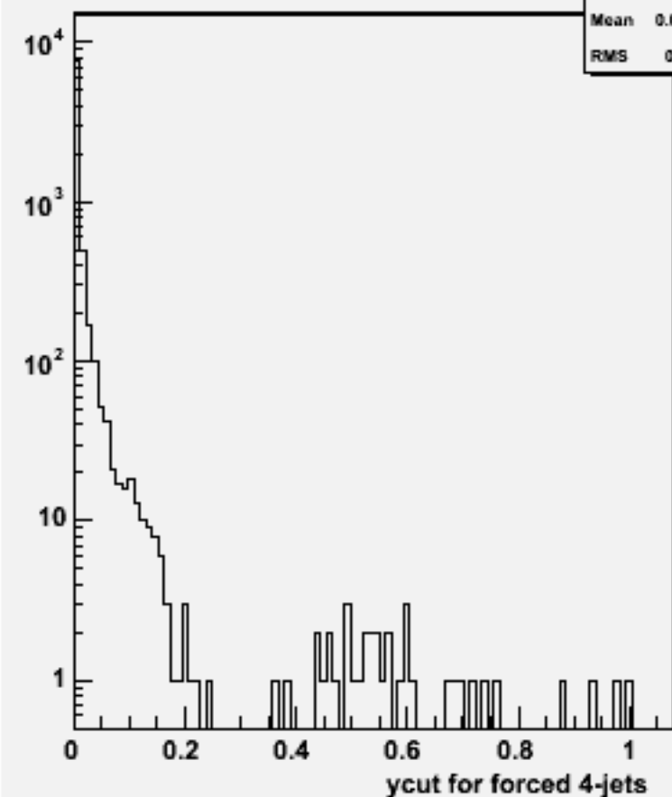
Ycut for 4-jets :w101992 n2n2n2n2ss_o
