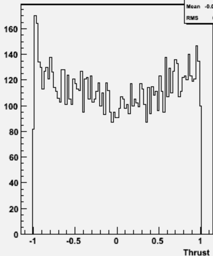
cos \Theta (thrust) w101992 n2n2n2n2ss_o
