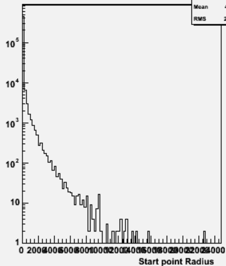
Start point R : w101992 n2n2n2n2ss_o
