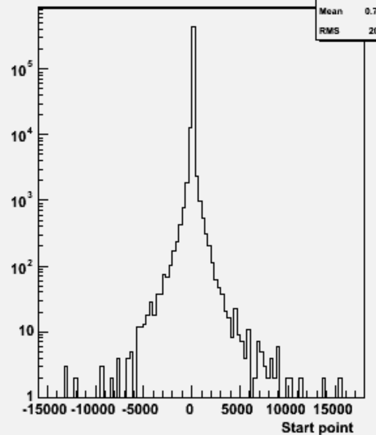
Start point Z : w101992 n2n2n2n2ss_o
