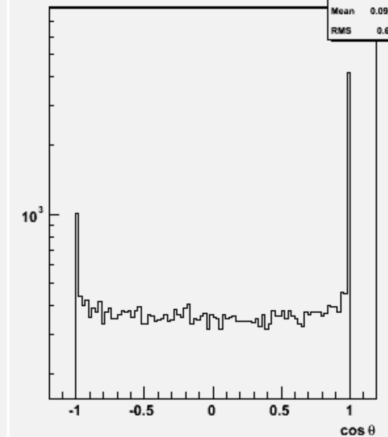
Jet cos \theta (All jets)w101988 n2n2n2n2dd_o
