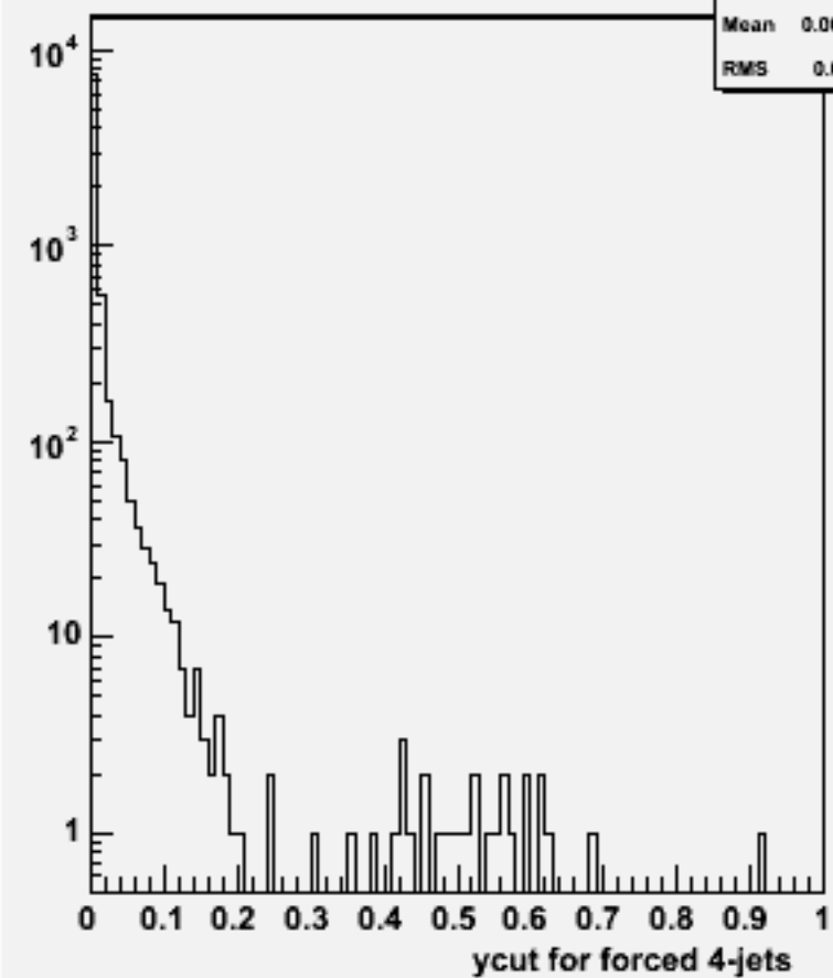
Ycut for 4-jets :w101988 n2n2n2n2dd_o
