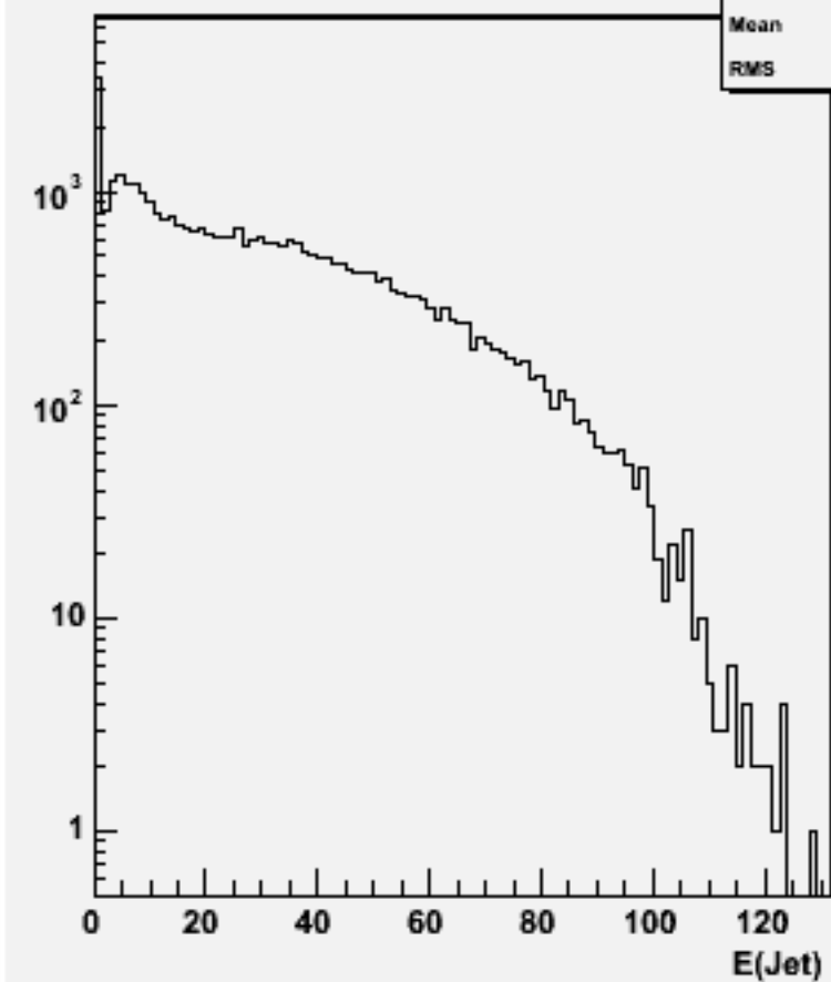
Jet energies(All jets)w101988 n2n2n2n2dd_o
