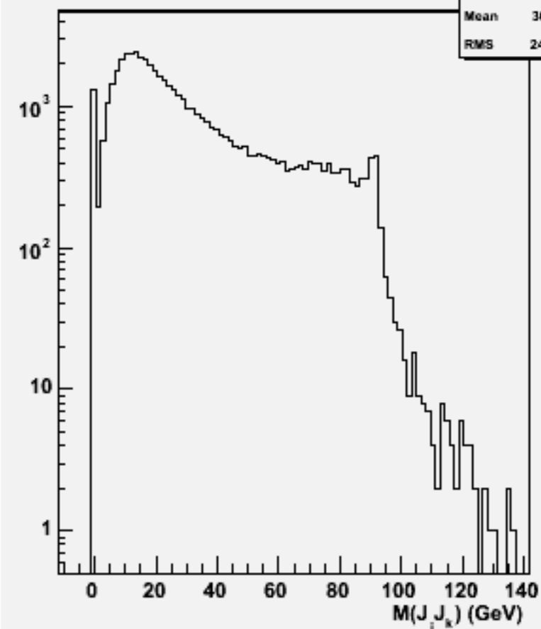
2jets mass(All comb)w101988 n2n2n2n2dd_o
