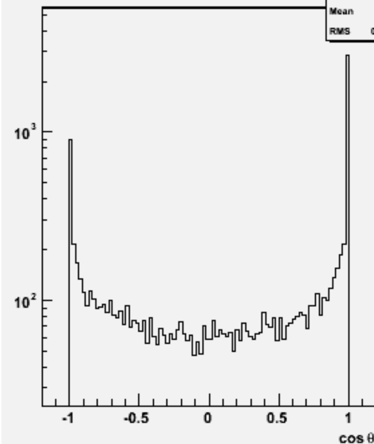
Jet cos \theta (All jets)w101984 n2n2n2n2e3e3_o
