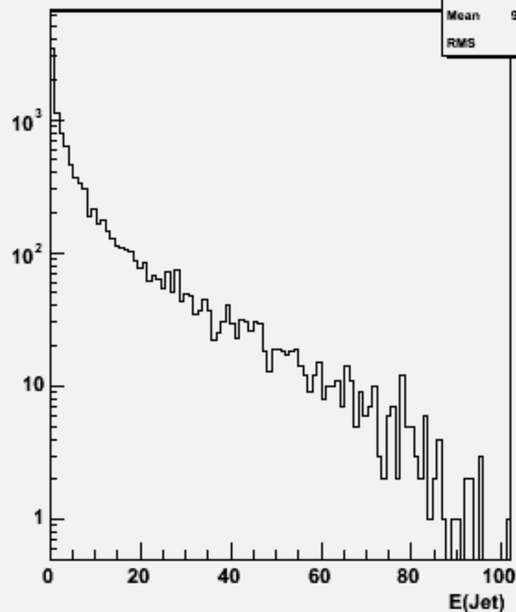
Jet energies(All jets)w101984 n2n2n2n2e3e3_o
