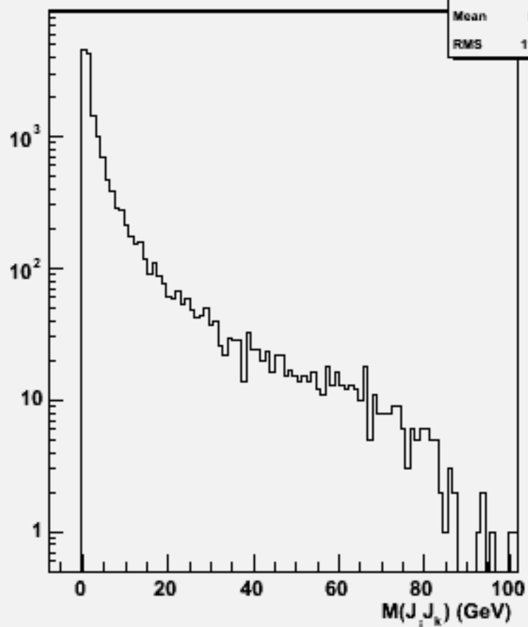
2jets mass(All comb)w101984 n2n2n2n2e3e3_o
