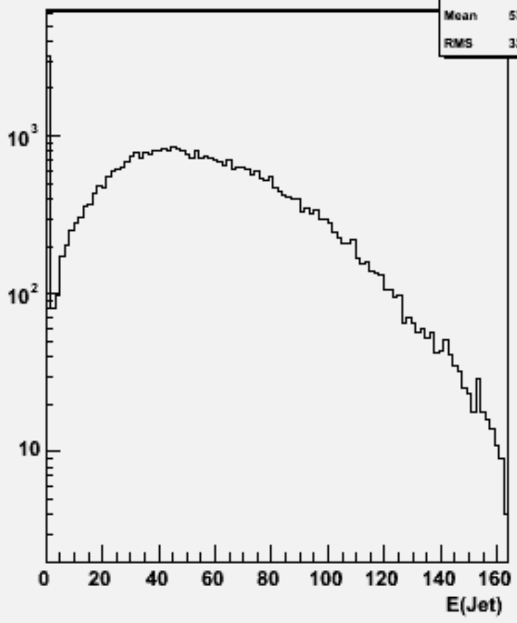
Jet energies(All jets)w101977 n1n1ccbb_o
