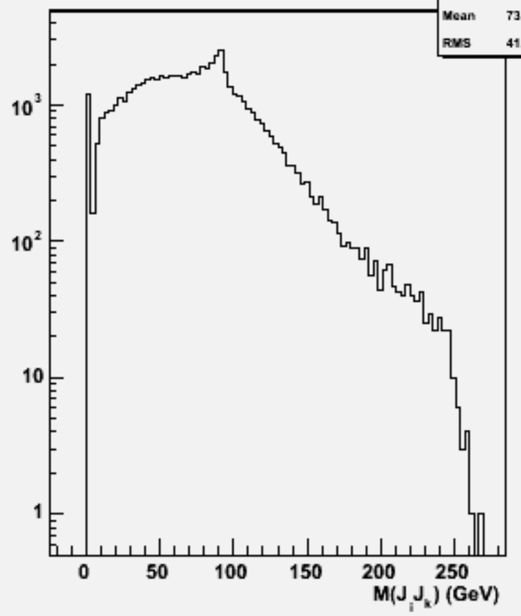
2jets mass(All comb)w101977 n1n1ccbb_o
