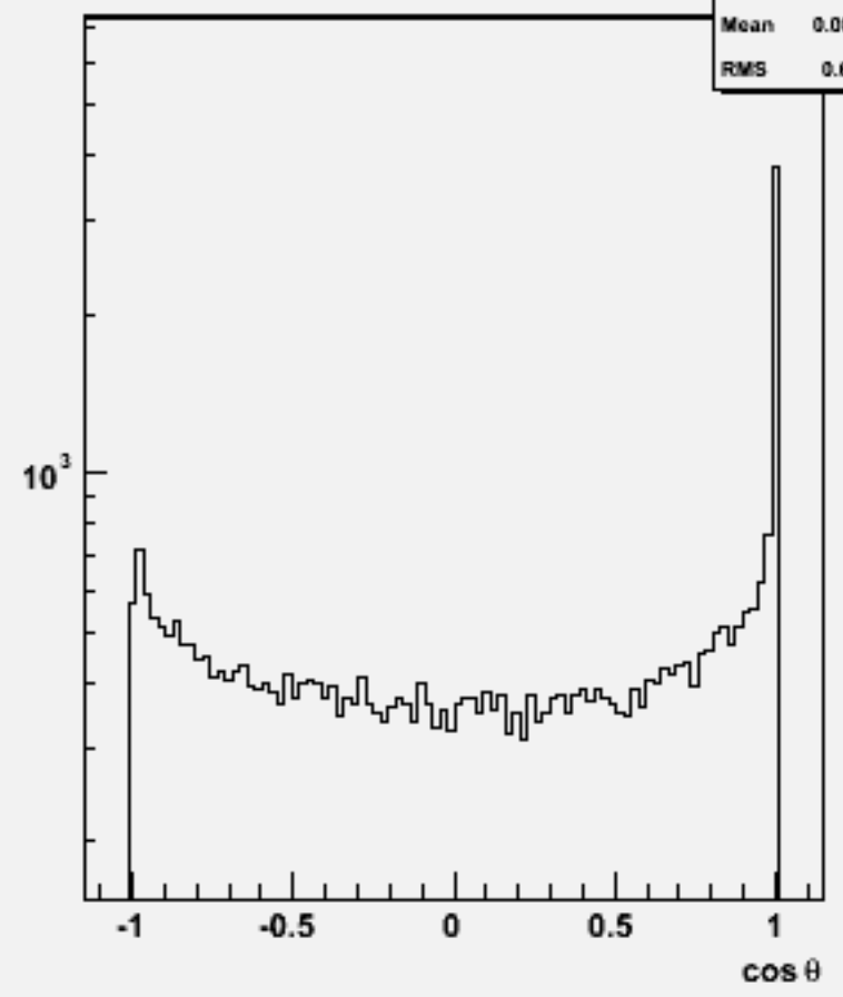
Jet cosθ (All jets)w101977 n1n1ccbb_o
