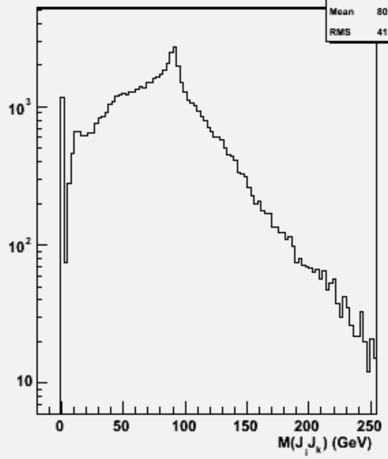
2jets mass(All comb)w101976 n1n1ccbb_o
