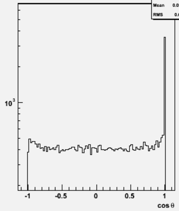
Jet cosθ (All jets)w101976 n1n1ccbb_o
