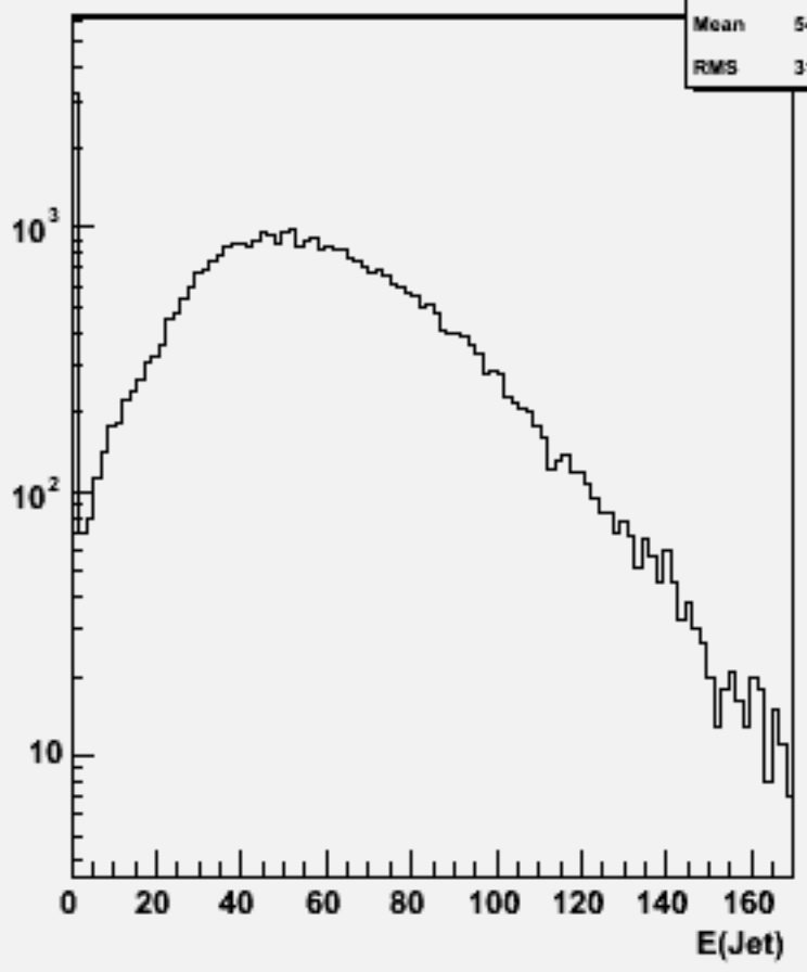
Jet energies(All jets)w101976 n1n1ccbb_o
