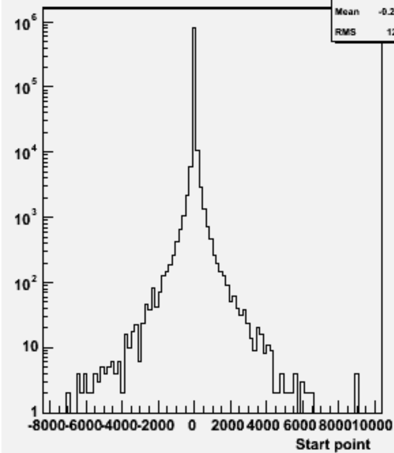
Start point Z : w101972 n1n1ccdd_o
