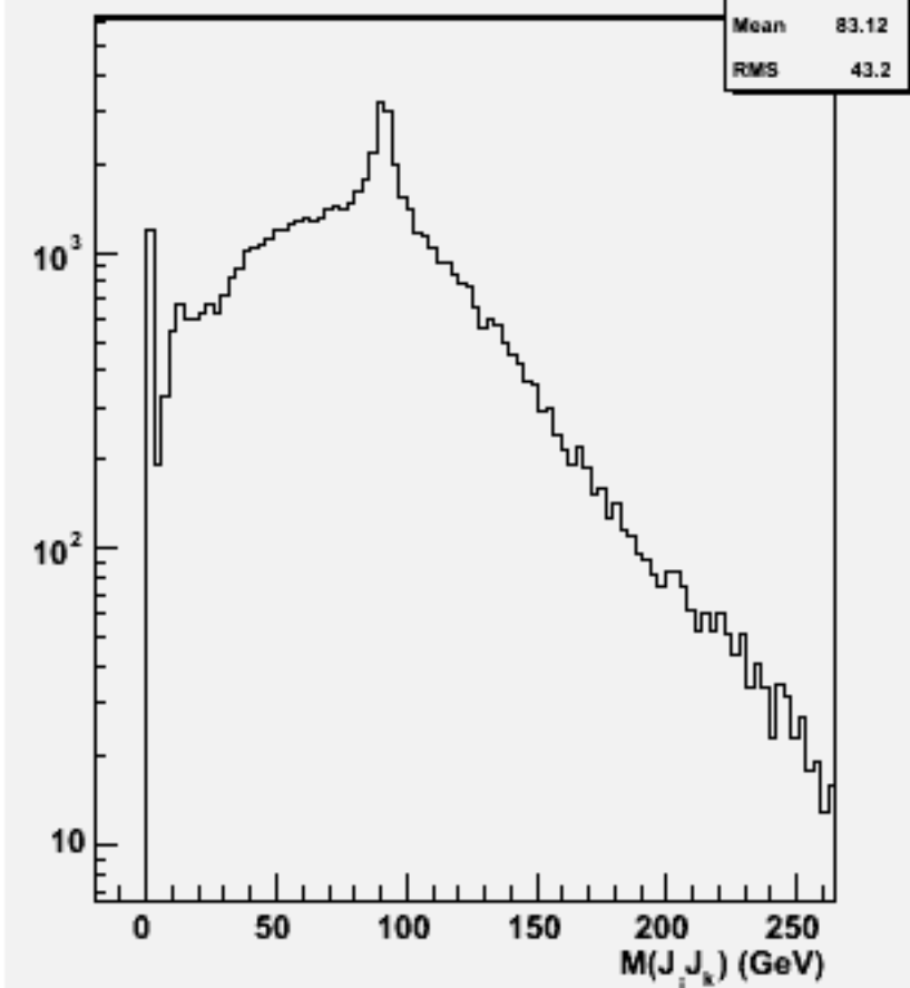
2jets mass(All comb)w101972 n1n1ccdd_o
