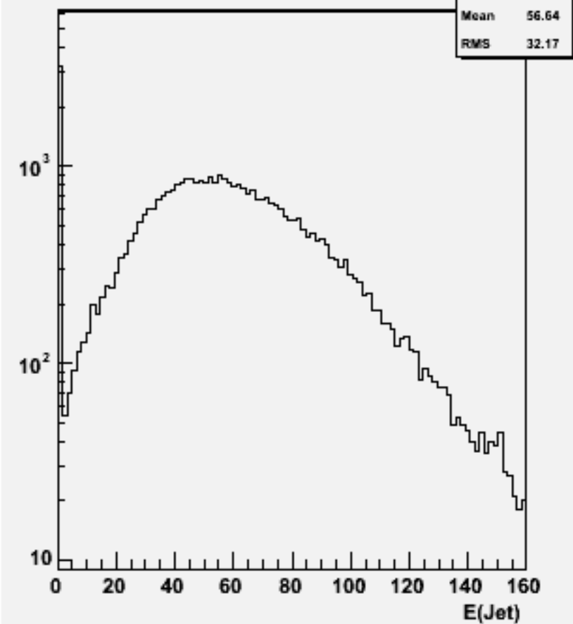
Jet energies(All jets)w101972 n1n1ccdd_o
