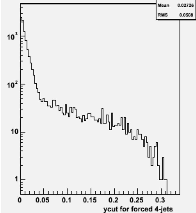
Ycut for 4-jets :w101972 n1n1ccdd_o
