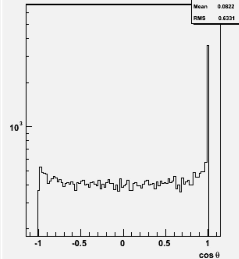
Jet cos \theta (All jets)w101972 n1n1ccdd_o
