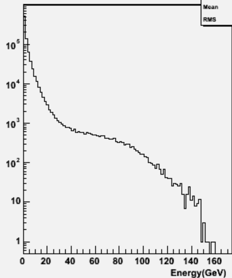
Particle Energy : w101972 n1n1ccdd_o
