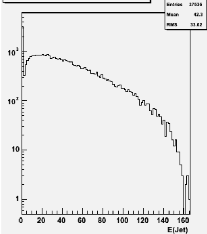
Jet energies(All jets)w101969 n1n1cce3e3_o
