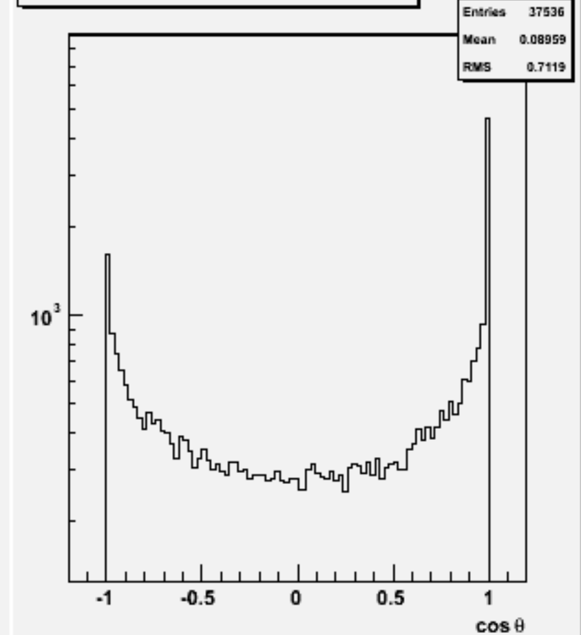
Jet cos \theta (All jets)w101969 n1n1cce3e3_o
