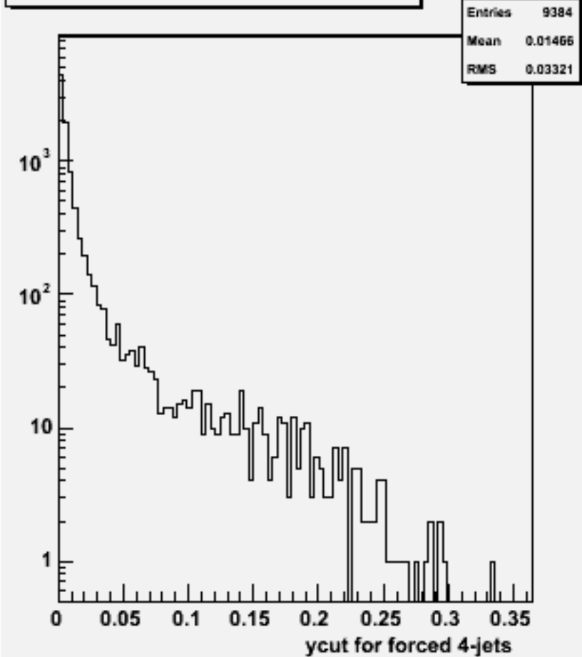
Ycut for 4-jets :w101969 n1n1cce3e3_o
