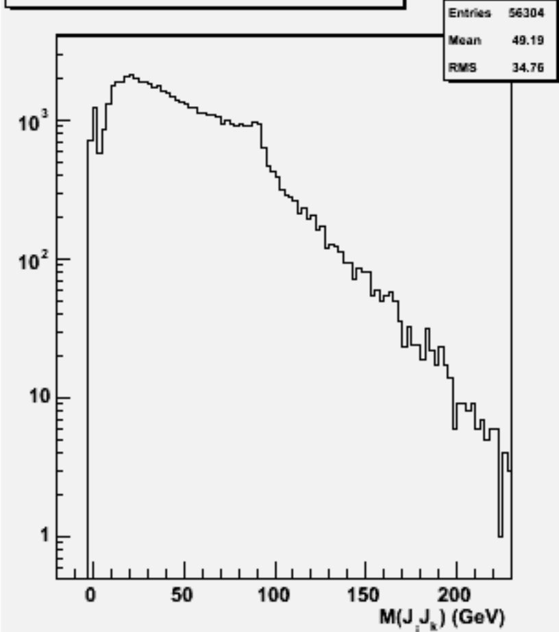
2jets mass(All comb)w101969 n1n1cce3e3_o
