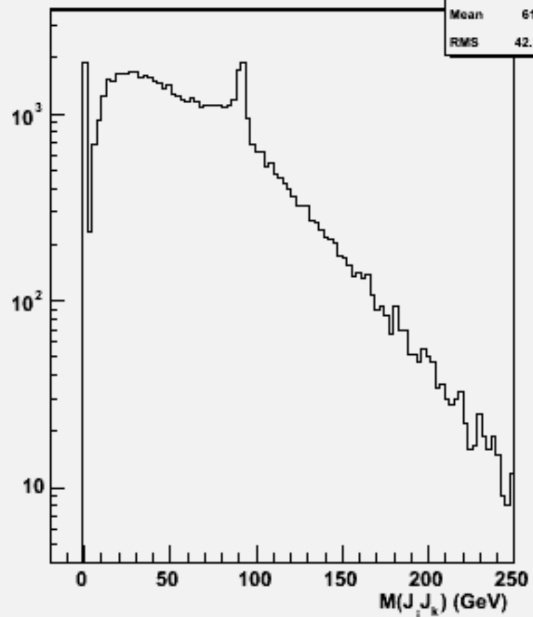
2jets mass(All comb)w101965 n1n1cce2e2_o
