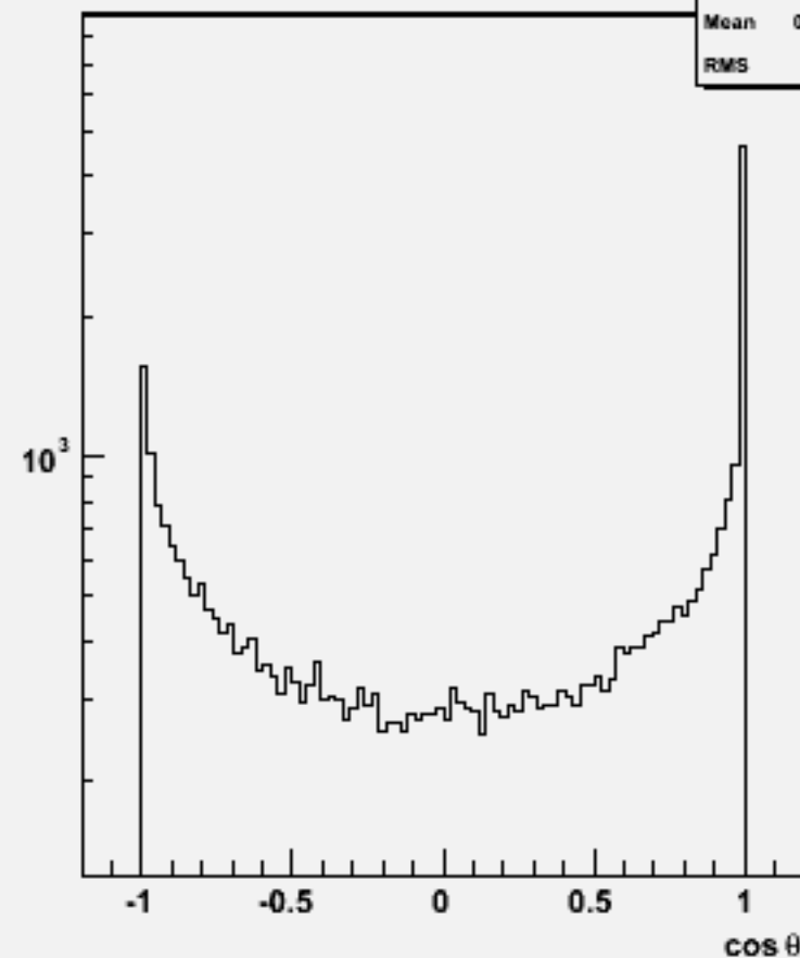
Jet cos \theta (All jets)w101965 n1n1cce2e2_o
