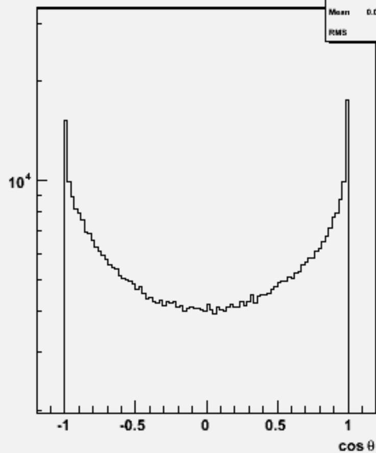
Particle cosθ : w101965 n1n1cce2e2_o
