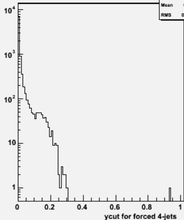
Ycut for 4-jets :w101965 n1n1cce2e2_o
