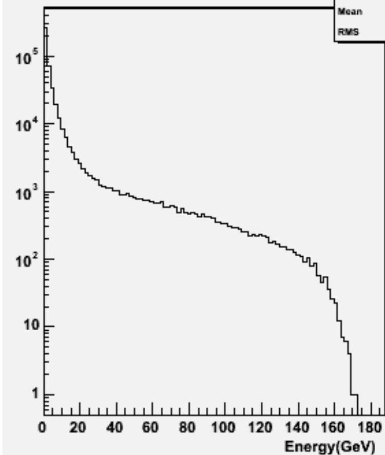
Start point R : w101965 n1n1cce2e2_o
