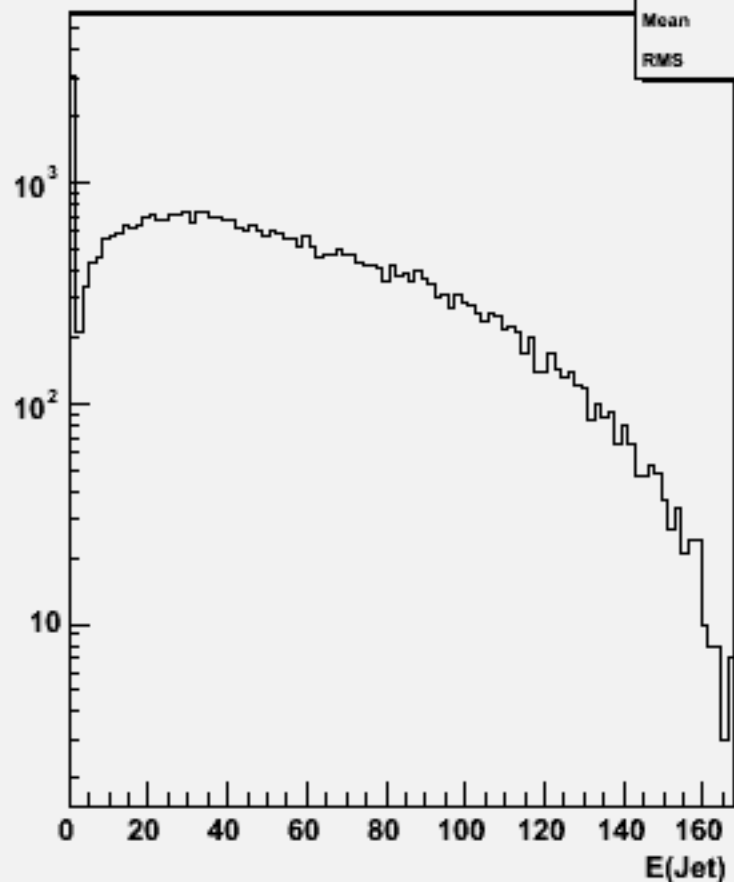
Jet energies(All jets)w101965 n1n1cce2e2_o
