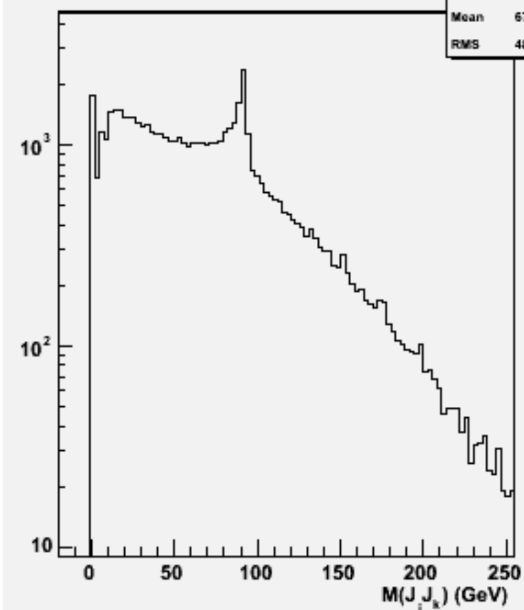
2jets mass(All comb)w101964 n1n1cce2e2_o
