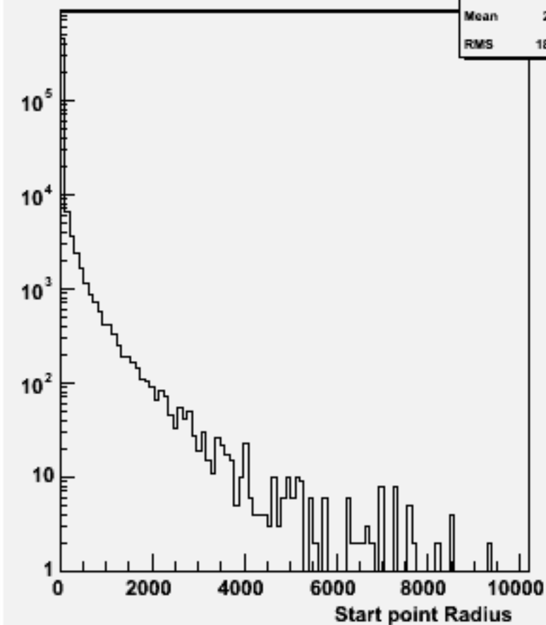
Start point R : w101964 n1n1cce2e2_o
