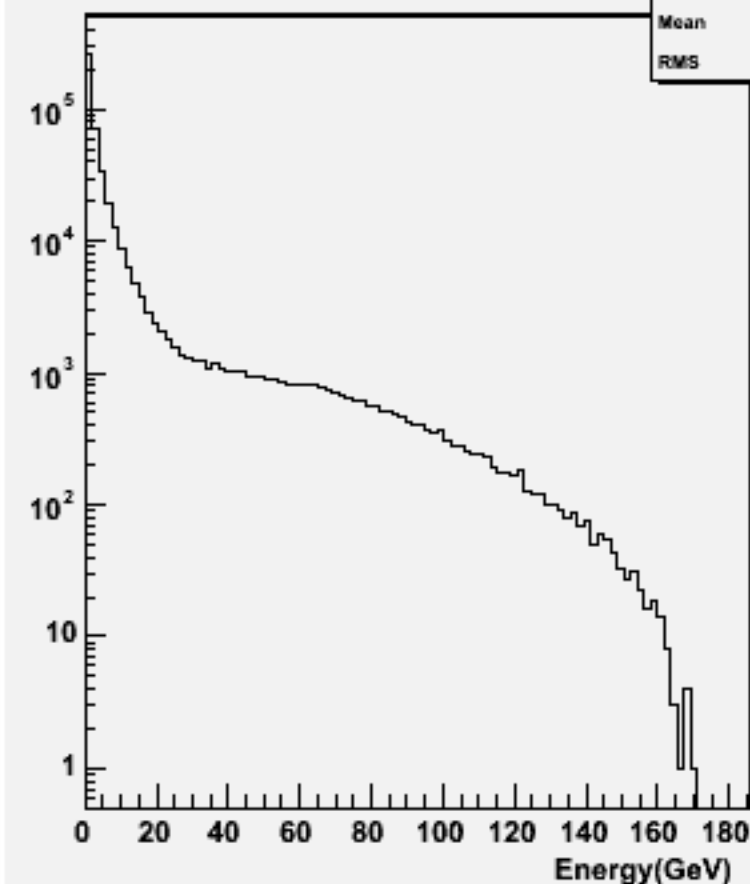
Particle Energy : w101964 n1n1cce2e2_o
