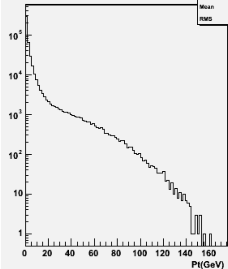
Particle Pt : w101964 n1n1cce2e2_o
