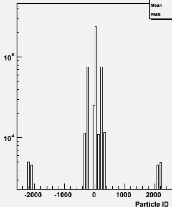
Particle ID : w101964 n1n1cce2e2_o
