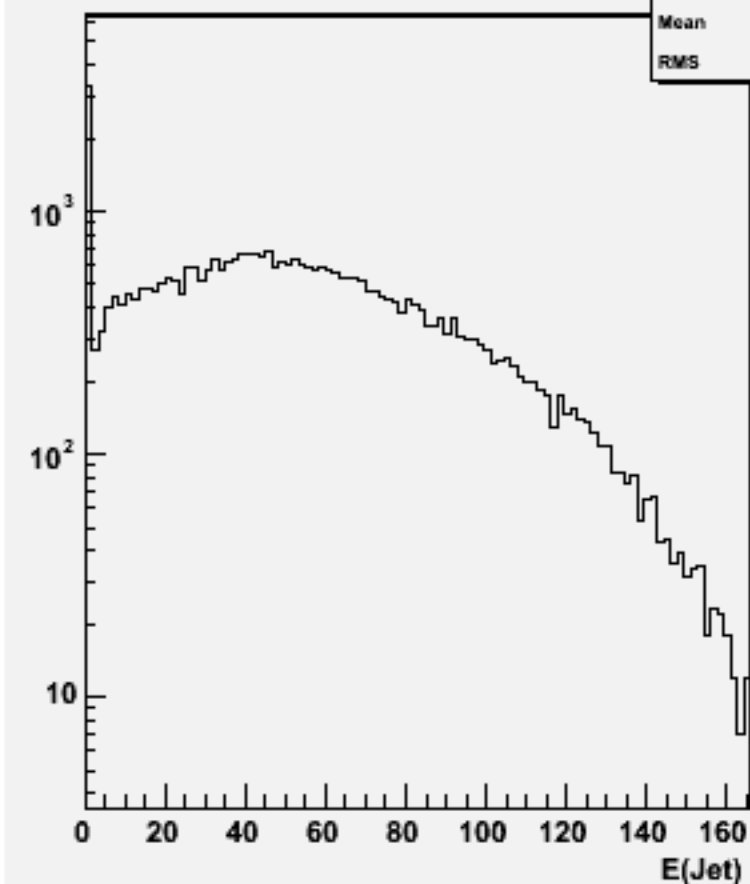
Jet energies(All jets)w101964 n1n1cce2e2_o
