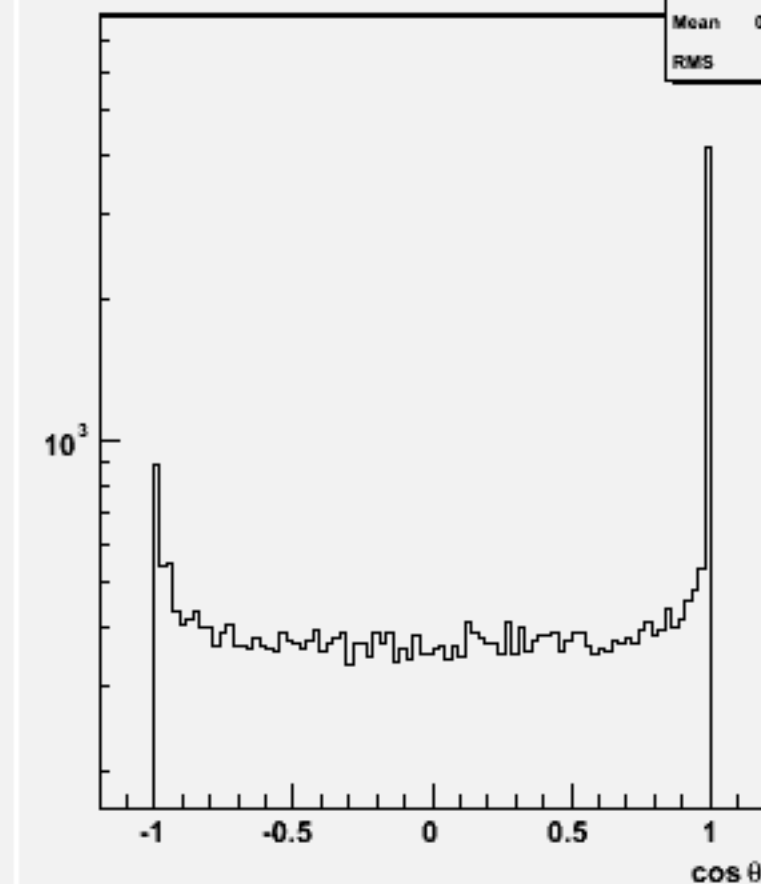
Jet cos \theta (All jets)w101964 n1n1cce2e2_o
