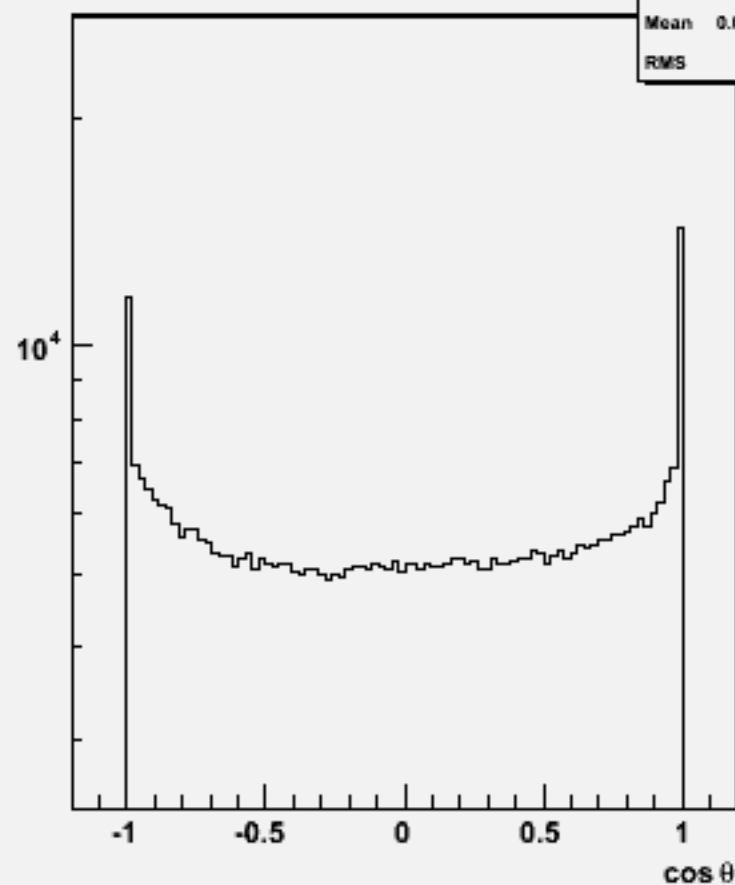
Particle cosθ : w101964 n1n1cce2e2_o
