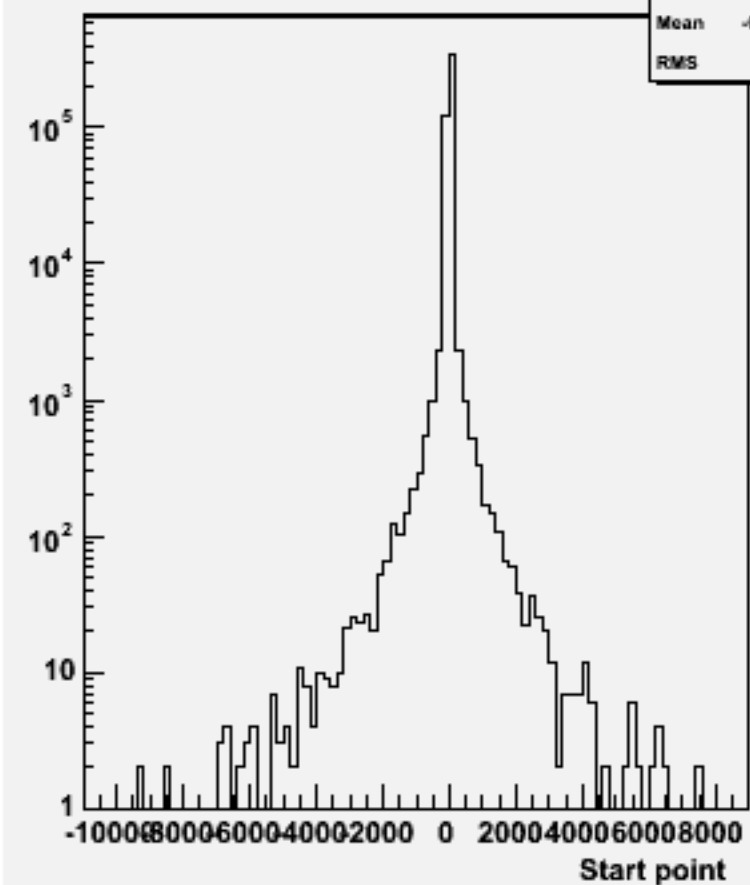
Start point Z : w101964 n1n1cce2e2_o
