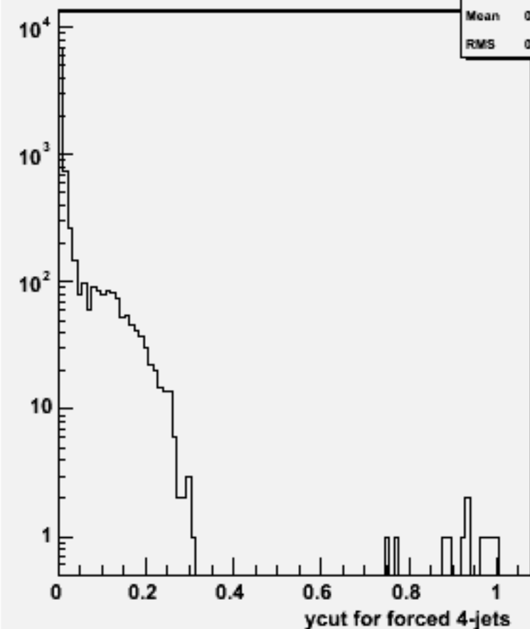
Ycut for 4-jets :w101964 n1n1cce2e2_o
