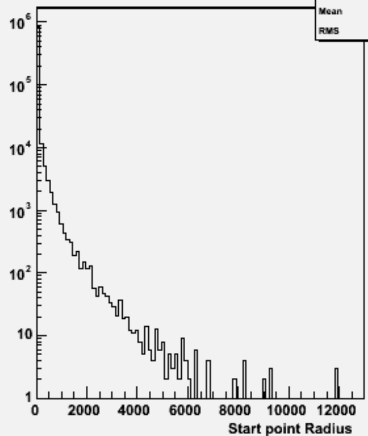
Start point R : w101961 n1n1uubb_o
