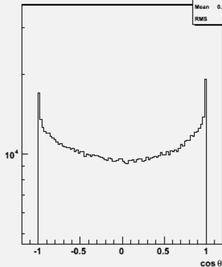
Particle cos \theta : w101961 n1n1uubb_o
