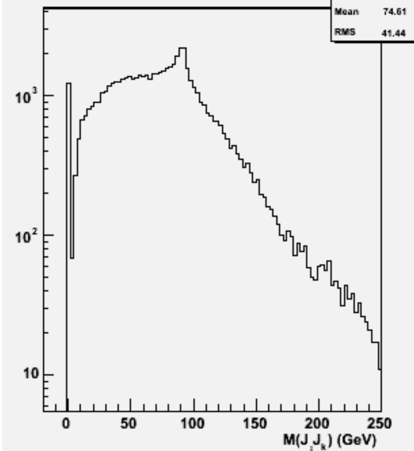
2jets mass(All comb)w101961 n1n1uubb_o
