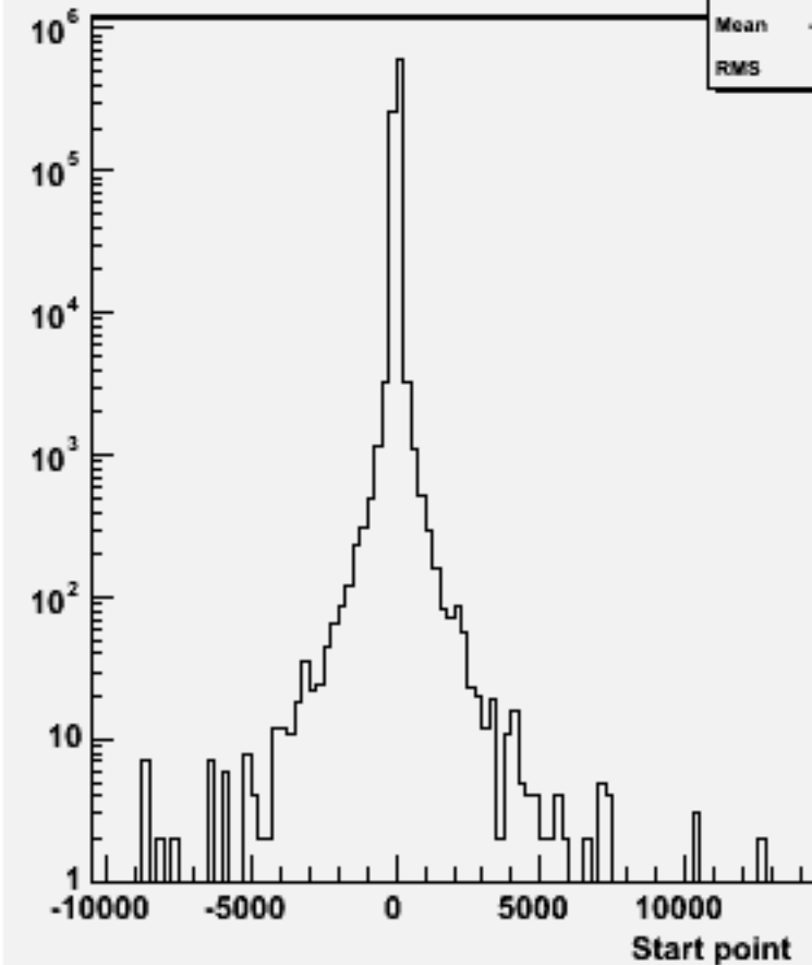
Start point Z : w101961 n1n1uubb_o
