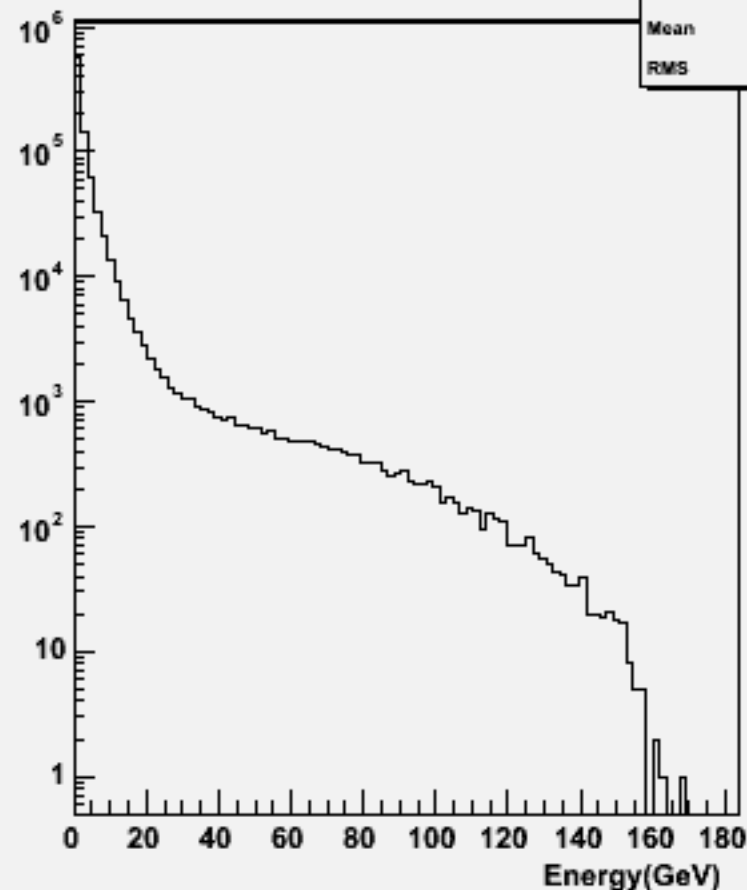
Particle Energy : w101961 n1n1uubb_o
