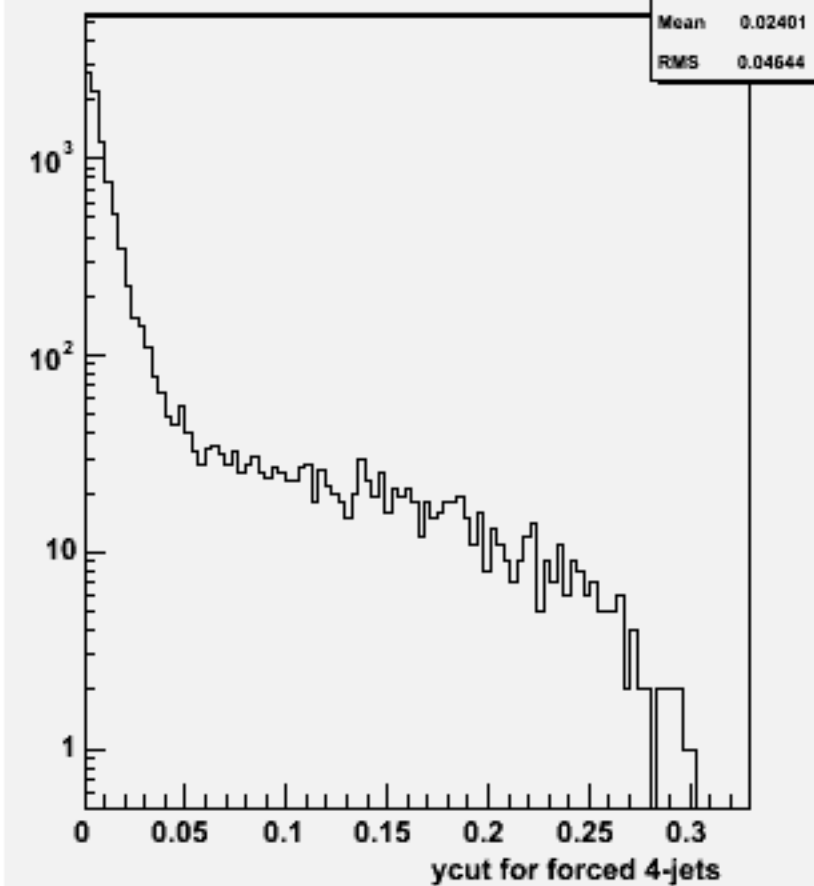
Ycut for 4-jets :w101961 n1n1uubb_o
