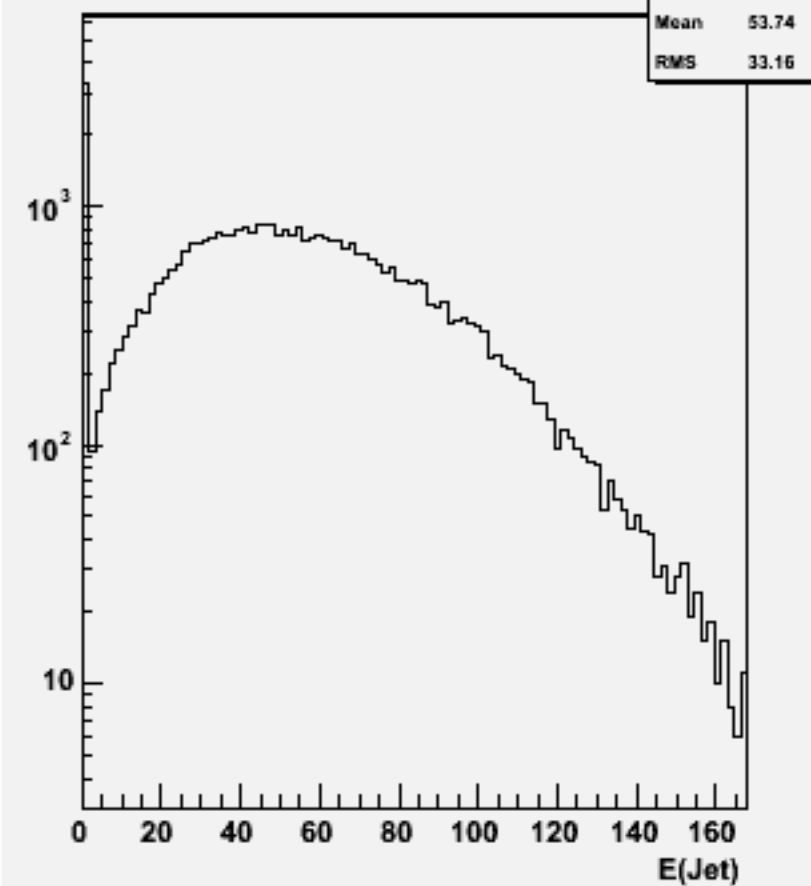
Jet energies(All jets)w101961 n1n1uubb_o
