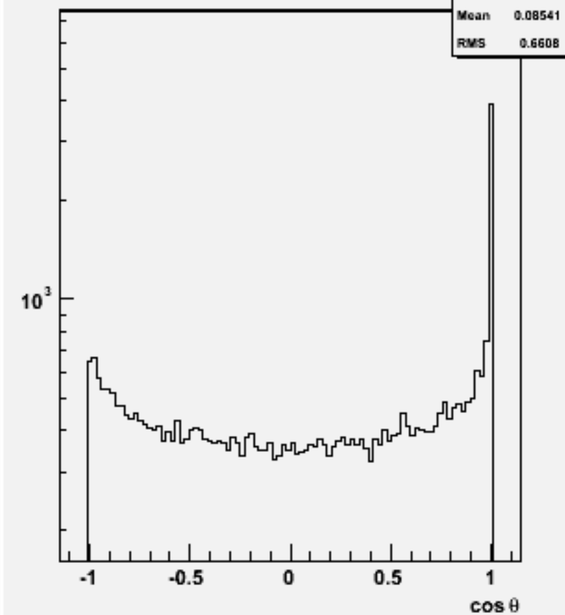
Jet cos \theta (All jets)w101961 n1n1uubb_o
