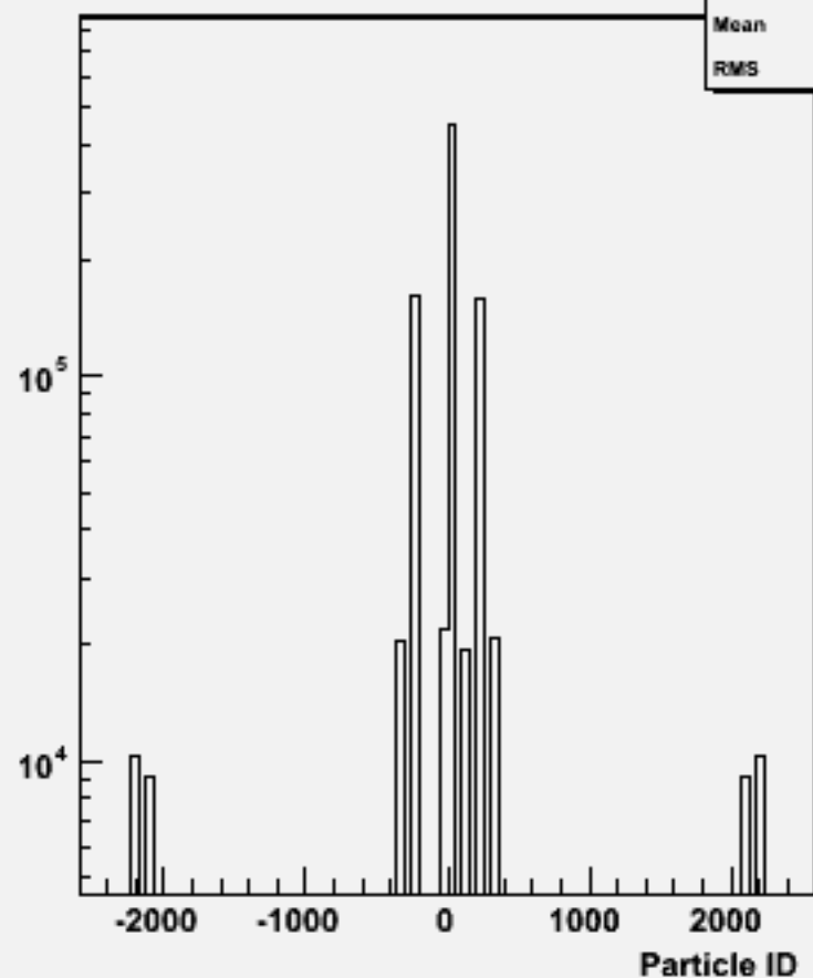
Particle ID : w101961 n1n1uubb_o
