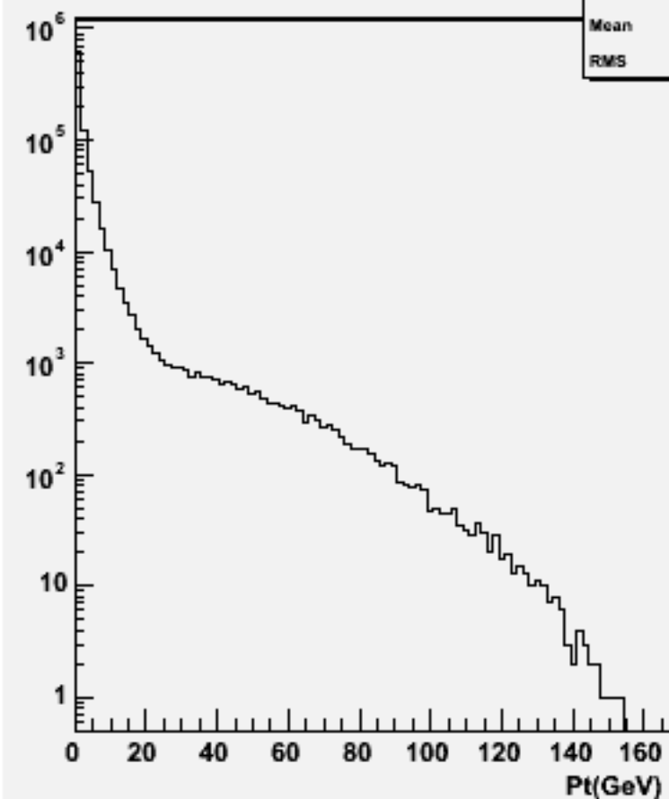
Particle Pt : w101961 n1n1uubb_o
