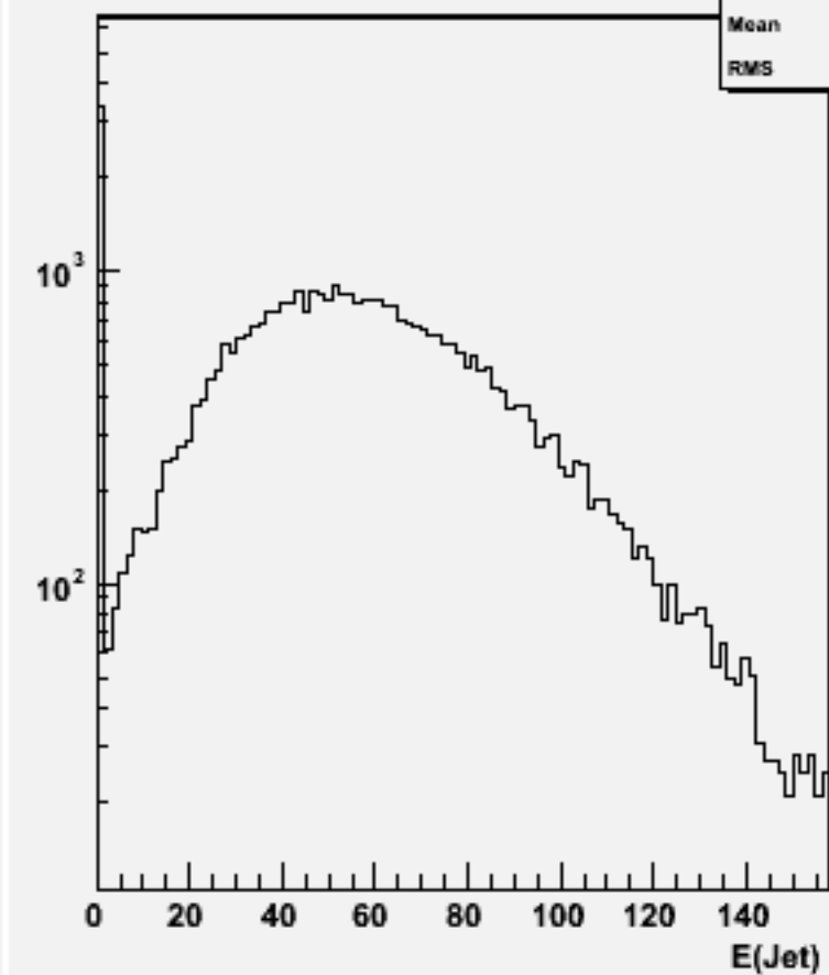
Jet energies(All jets)w101960 n1n1uubb_o
