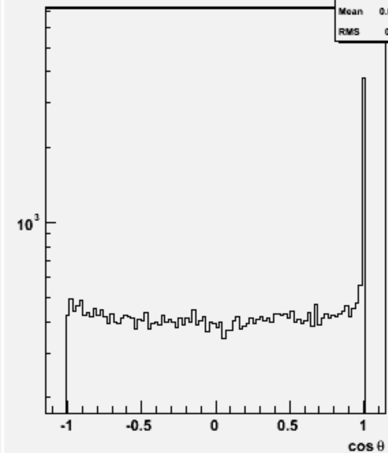
Jet cosθ (All jets)w101960 n1n1uubb_o
