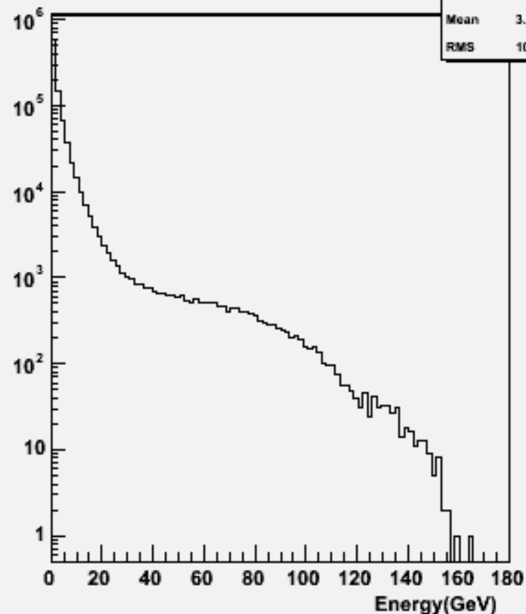
Particle Energy : w101960 n1n1uubb_o
