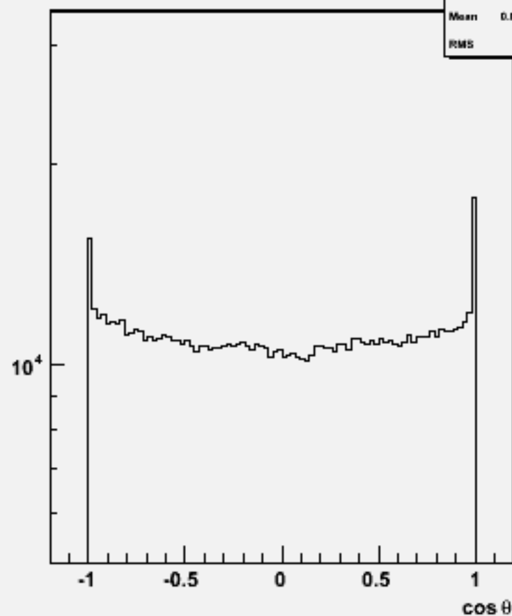
Particle cos \theta : w101960 n1n1uubb_o
