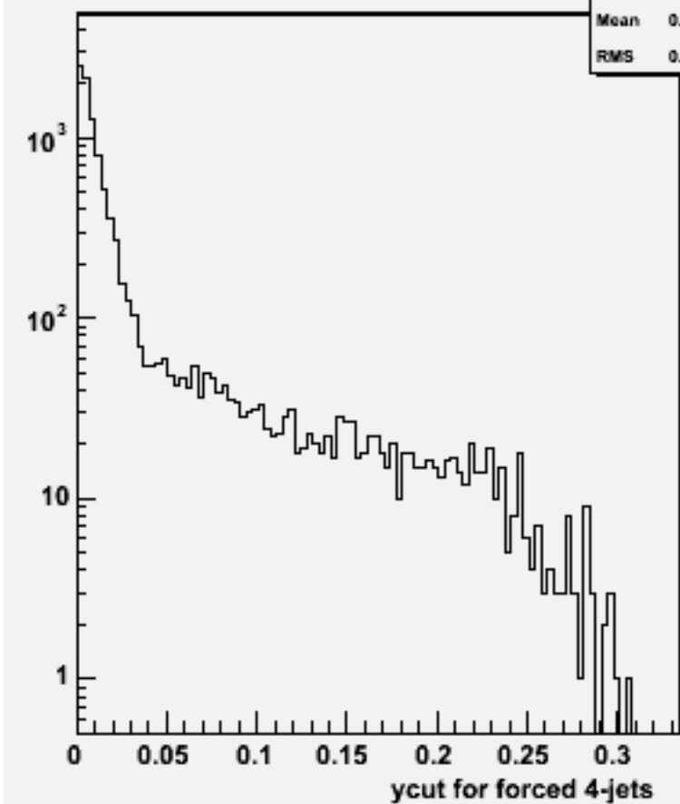
Ycut for 4-jets :w101960 n1n1uubb_o
