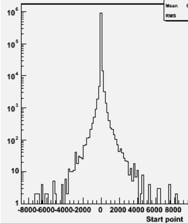
Start point Z : w101960 n1n1uubb_o
