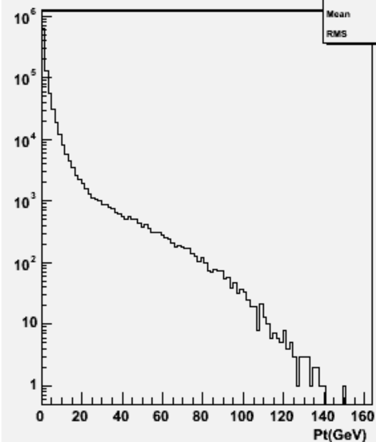
Particle Pt : w101960 n1n1uubb_o
