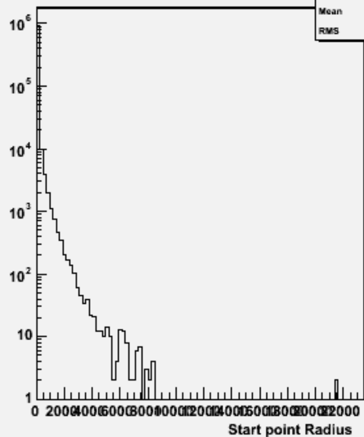
Start point R : w101960 n1n1uubb_o
