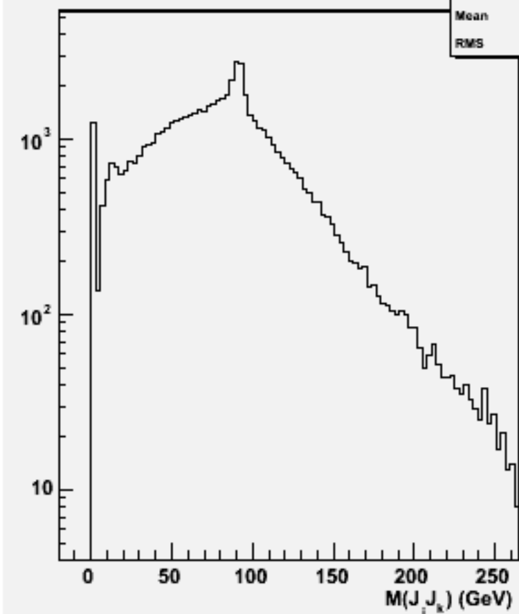
2jets mass(All comb)w101960 n1n1uubb_o
