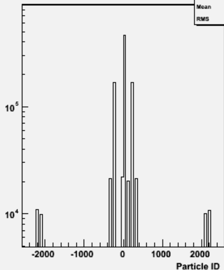
Particle ID : w101960 n1n1uubb_o
