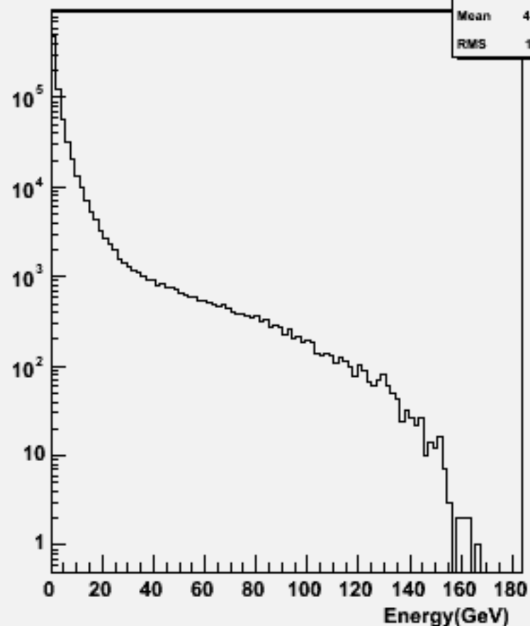
Particle Energy : w101957 n1n1uuss_o
