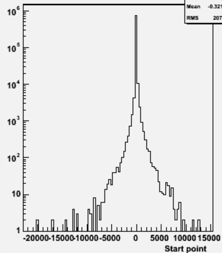
Start point Z : w101957 n1n1uuss_o
