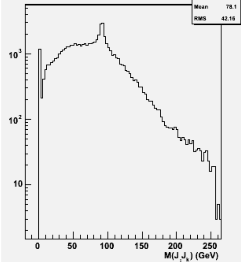
2jets mass(All comb)w101957 n1n1uuss_o
