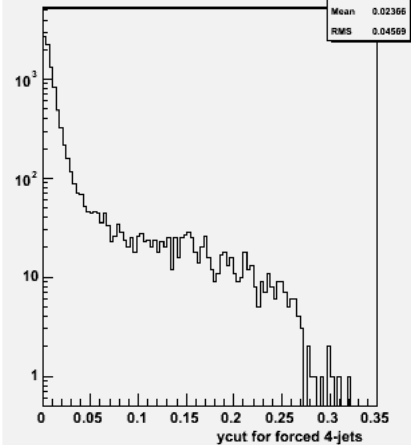
Ycut for 4-jets :w101957 n1n1uuss_o
