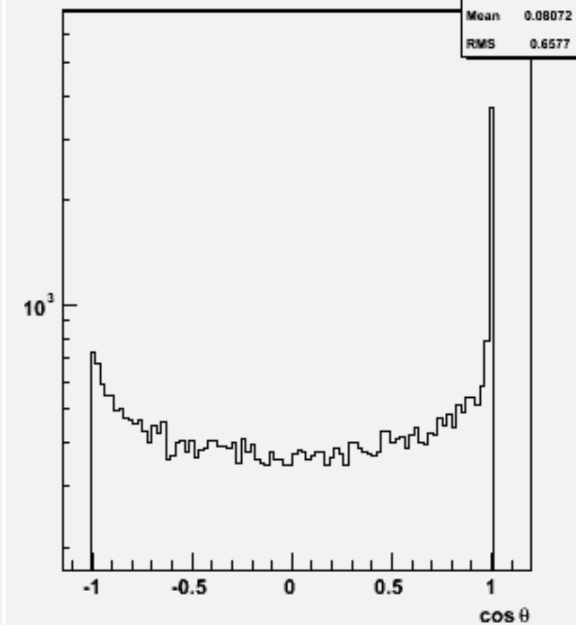
Jet cos \theta (All jets)w101957 n1n1uuss_o
