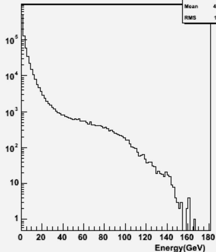
Particle Energy : w101956 n1n1uuss_o
