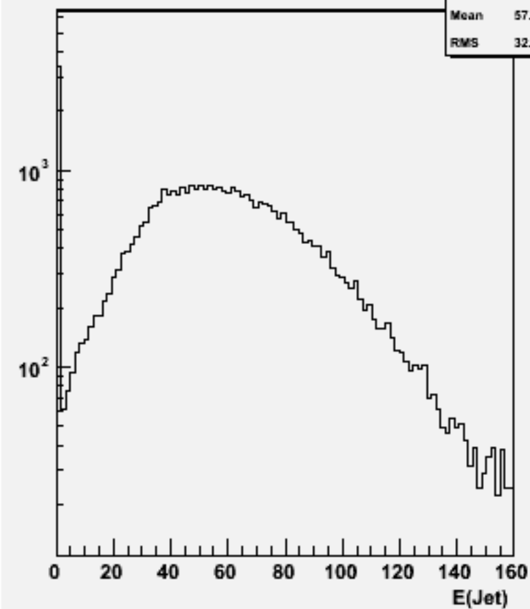
Jet energies(All jets)w101956 n1n1uuss_o
