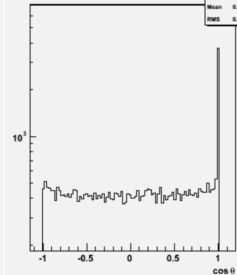
Jet cos \theta (All jets)w101956 n1n1uuss_o
