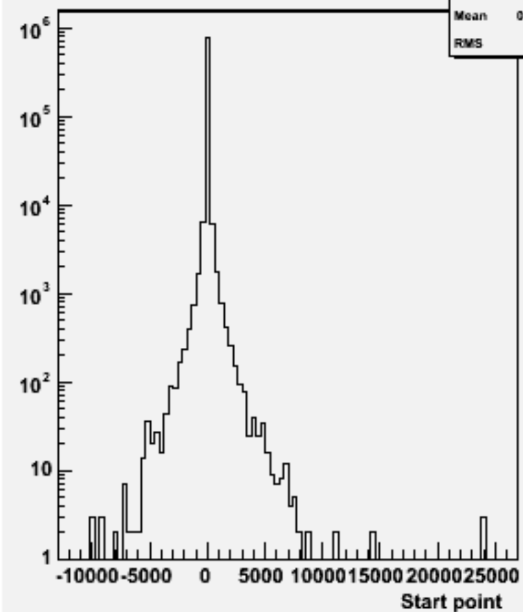
Start point Z : w101956 n1n1uuss_o
