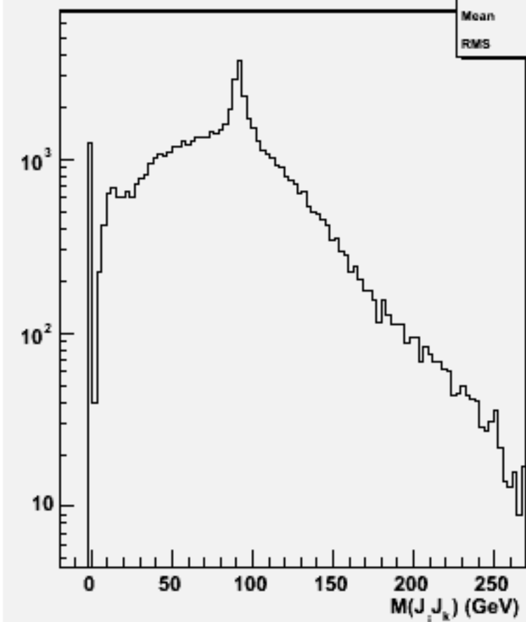
2jets mass(All comb)w101956 n1n1uuss_o
