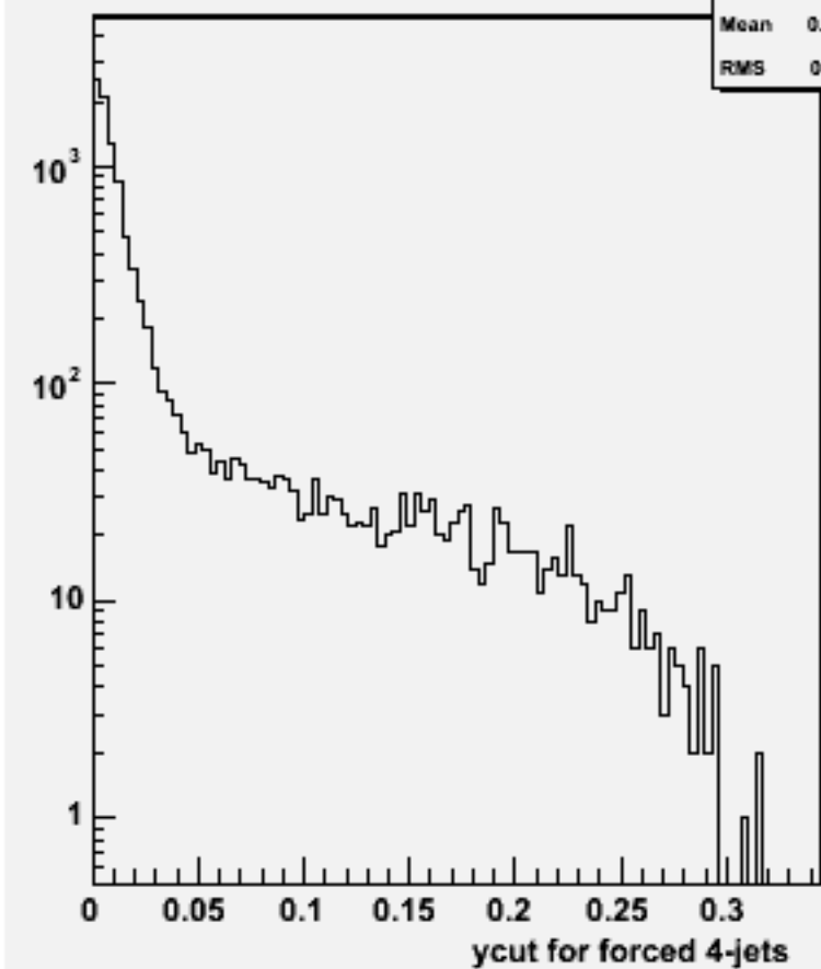
Ycut for 4-jets :w101956 n1n1uuss_o
