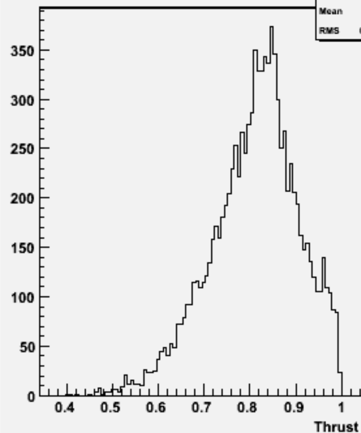
Thrust w101953 n1n1uue3e3_o
