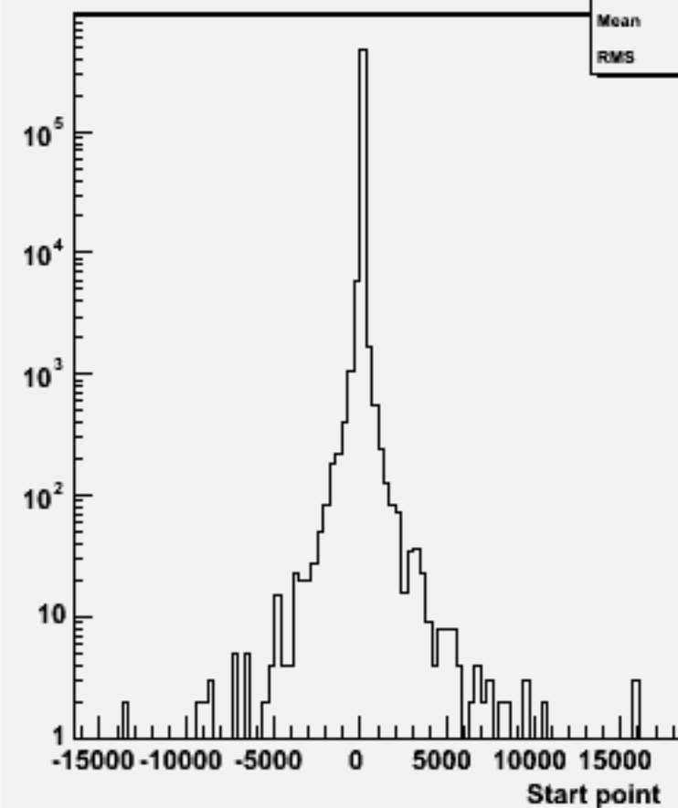
Start point Z : w101953 n1n1uue3e3_o
