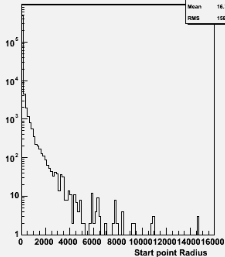
Start point R : w101953 n1n1uue3e3_o
