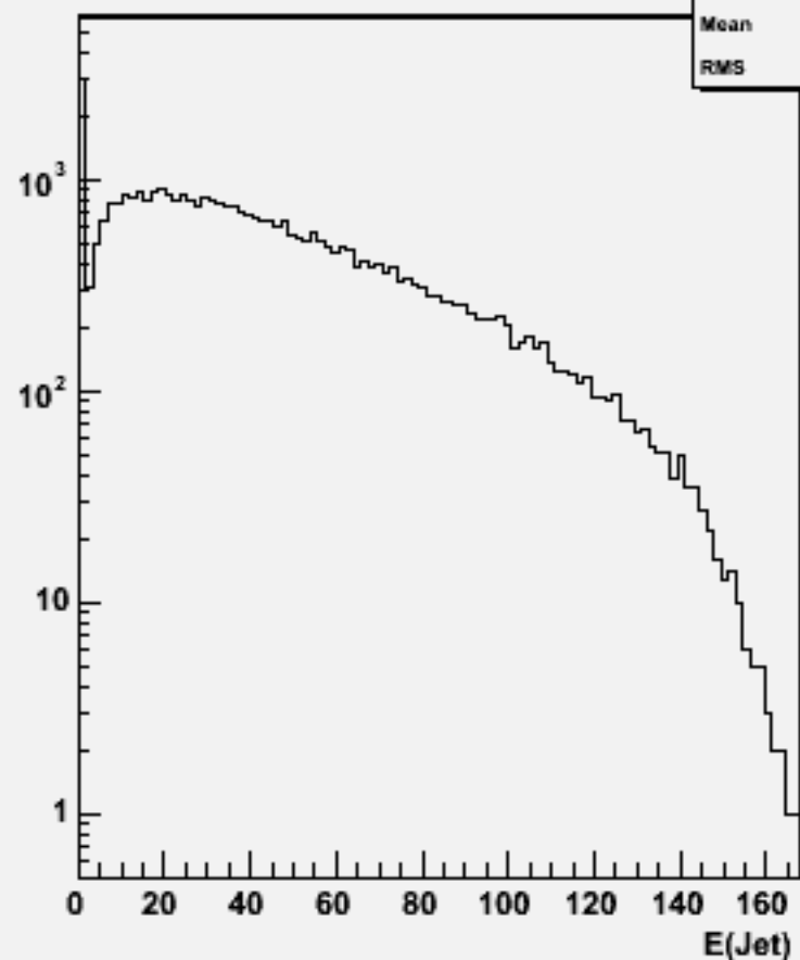
Jet energies(All jets)w101953 n1n1uue3e3_o
