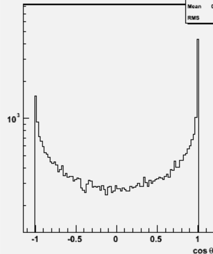
Jet cos \theta (All jets)w101953 n1n1uue3e3_o
