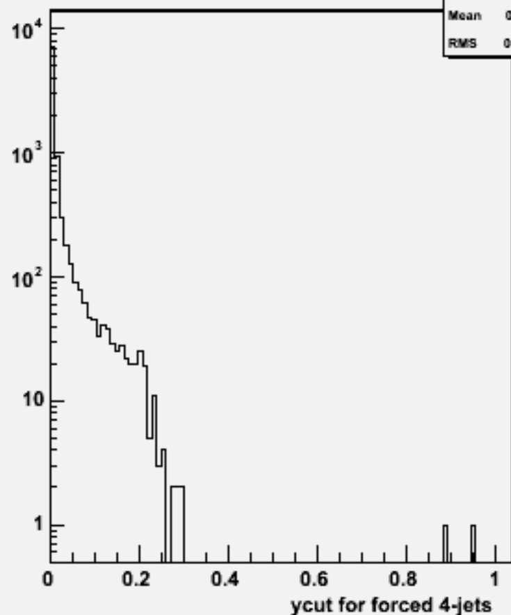
Ycut for 4-jets :w101953 n1n1uue3e3_o
