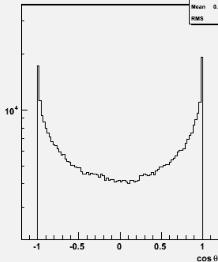
Particle cosθ : w101953 n1n1uue3e3_o
