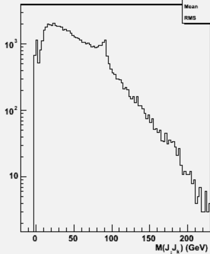
2jets mass(All comb)w101953 n1n1uue3e3_o
