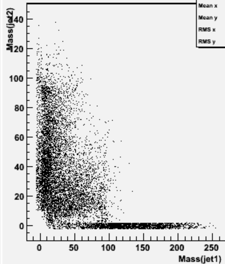
Jet mass for forced 2-jets : w101953 n1n1uue3e3_o
