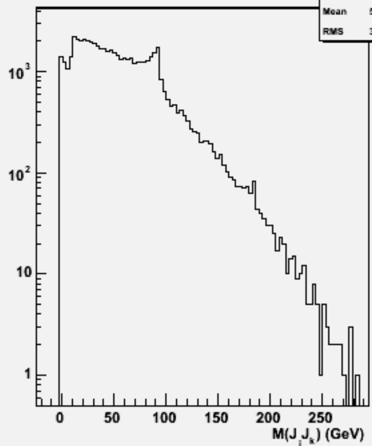
2jets mass(All comb)w101952 n1n1uue3e3_o
