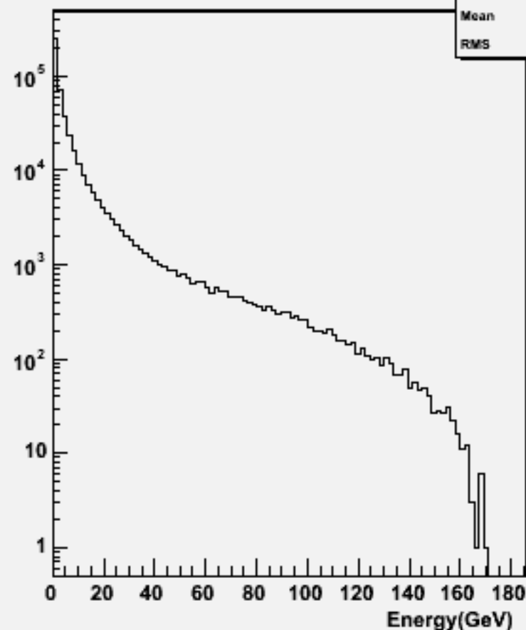
Start point R : w101952 n1n1uue3e3_o
