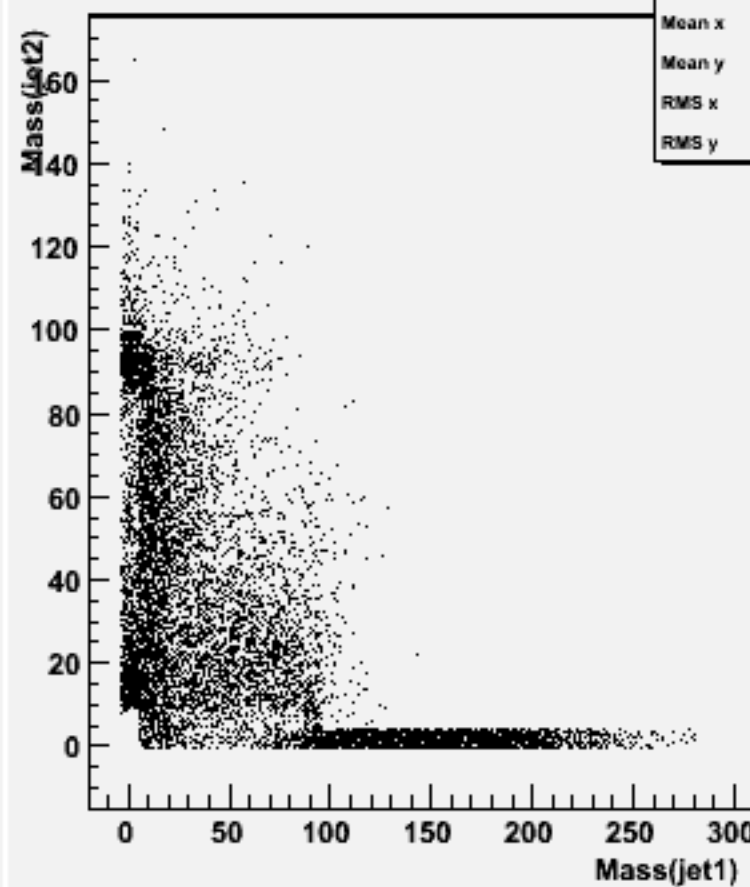
Jet mass for forced 2-jets : w101952 n1n1uue3e3_o
