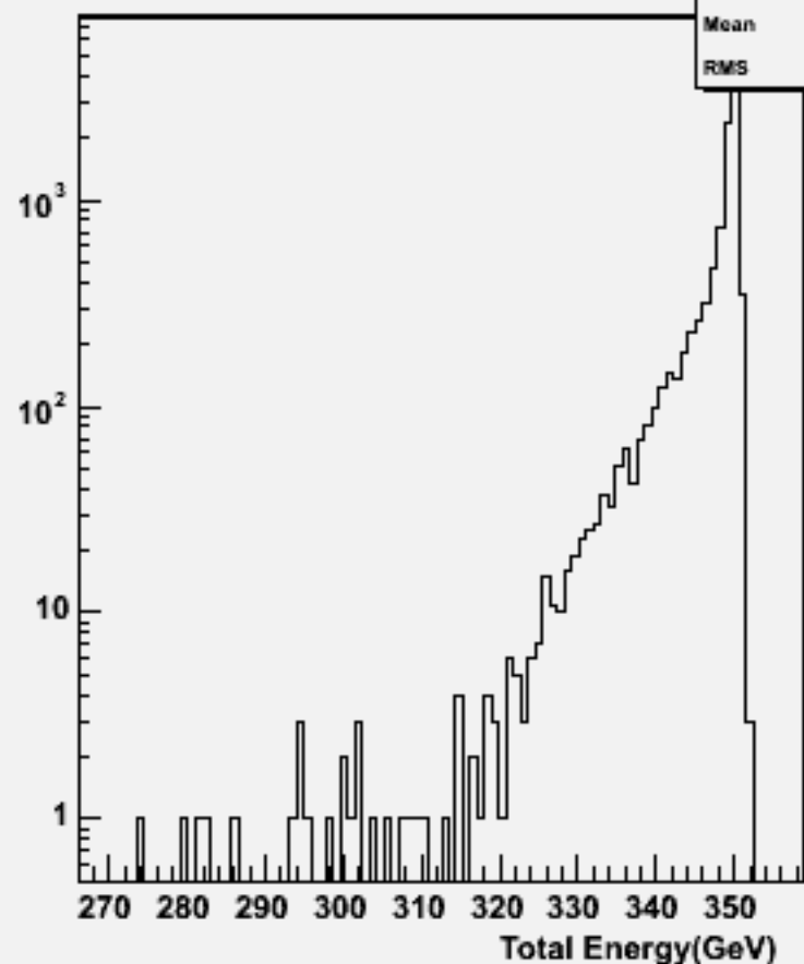
Pt Sum: w101952 n1n1uue3e3_o
