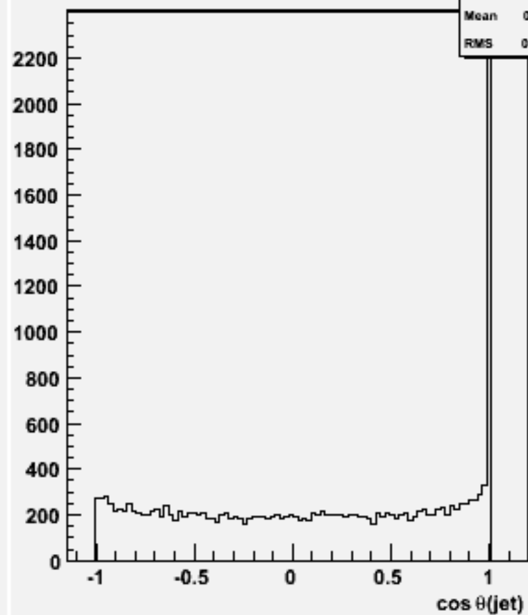
cos \theta for 2-jets :w101952 n1n1uue3e3_o
