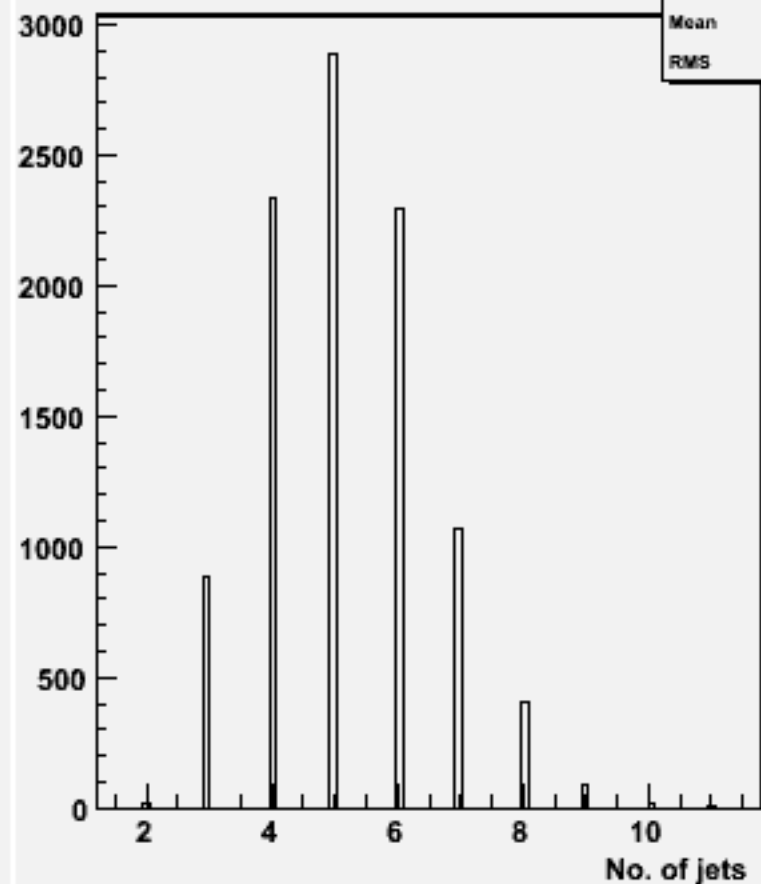
No. jets (ycut=0.001) : w101952 n1n1uue3e3_o
