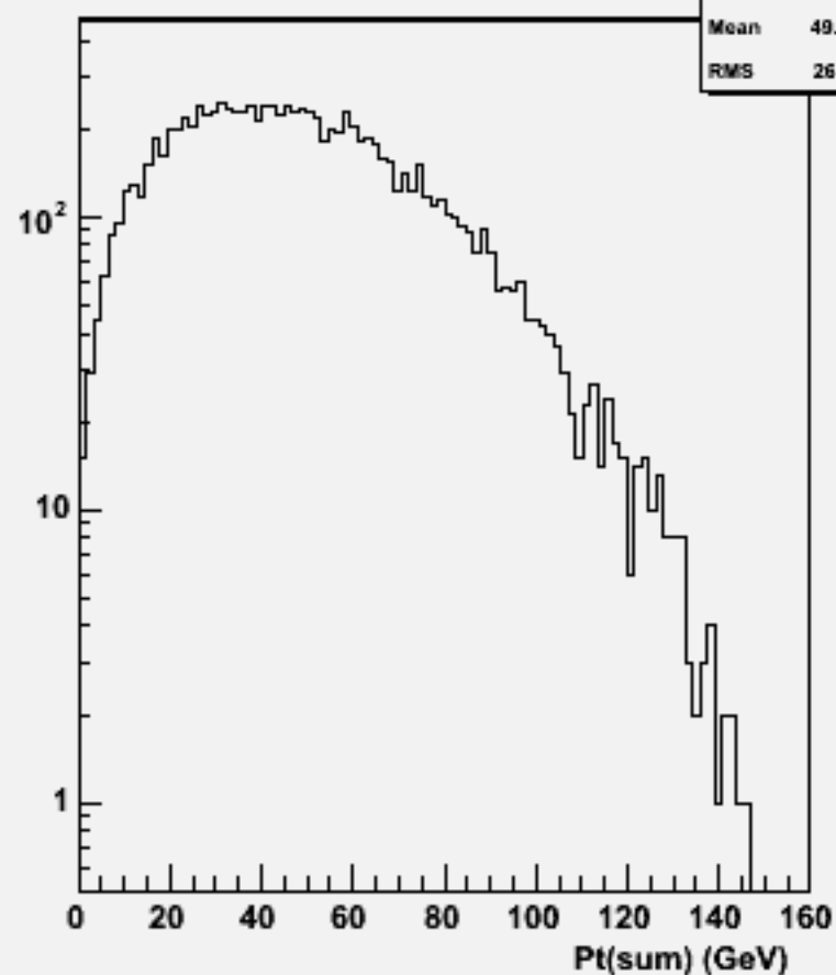
Pt Sum: w101952 n1n1uue3e3_o
