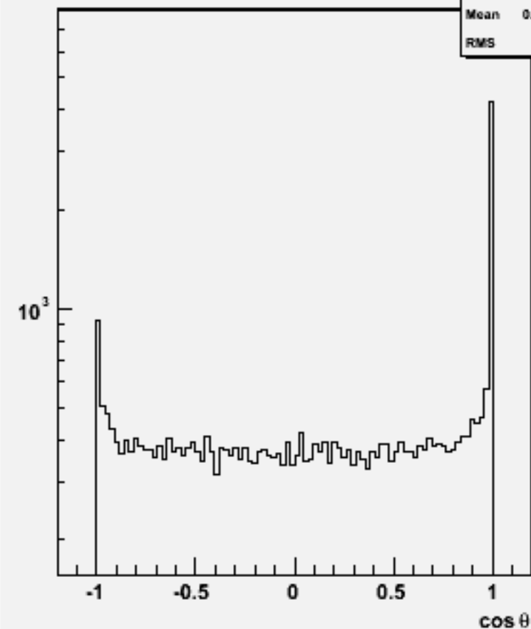
Jet cos \theta (All jets)w101952 n1n1uue3e3_o
