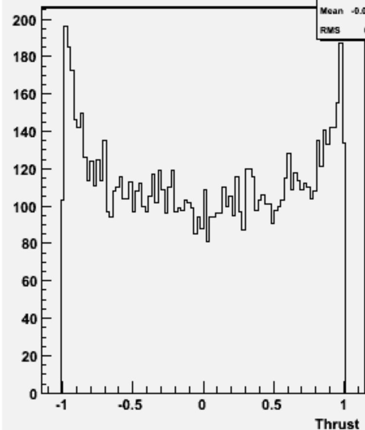
cos \Theta (thrust) w101952 n1n1uue3e3_o
