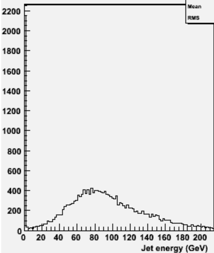
energy for 2-jets :w101952 n1n1uue3e3_o
