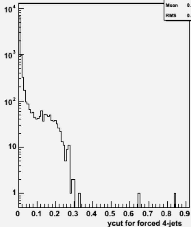
Ycut for 4-jets :w101952 n1n1uue3e3_o
