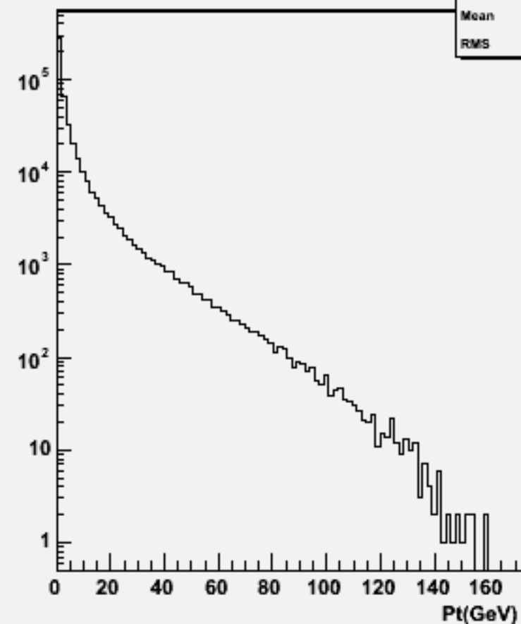
Start point Z : w101952 n1n1uue3e3_o
