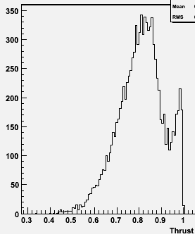
Thrust w101952 n1n1uue3e3_o
