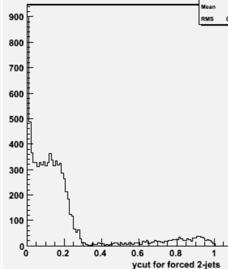
Ycut for 2-jets :w101952 n1n1uue3e3_o
