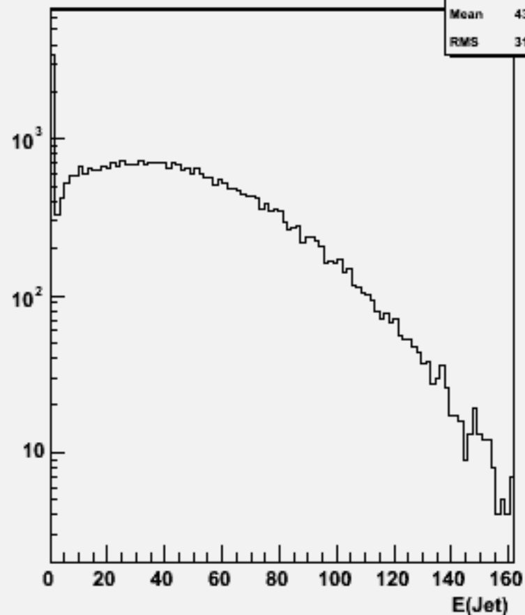
Jet energies(All jets)w101952 n1n1uue3e3_o
