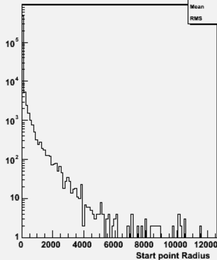
Start point R : w101952 n1n1uue3e3_o
