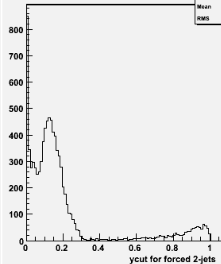
Ycut for 2-jets :w101948 n1n1uue2e2_o
