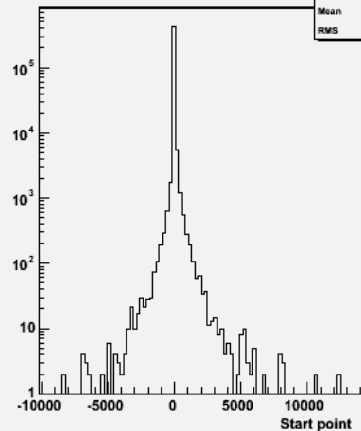
Start point Z : w101948 n1n1uue2e2_o
