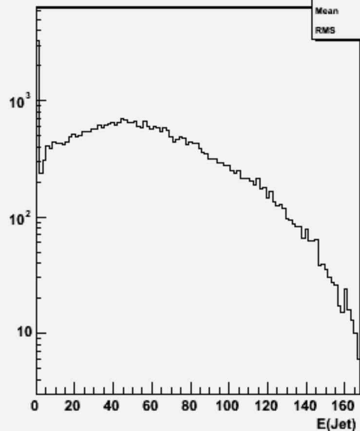
Jet energies(All jets)w101948 n1n1uue2e2_o
