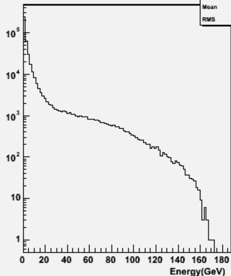
Start point R : w101948 n1n1uue2e2_o
