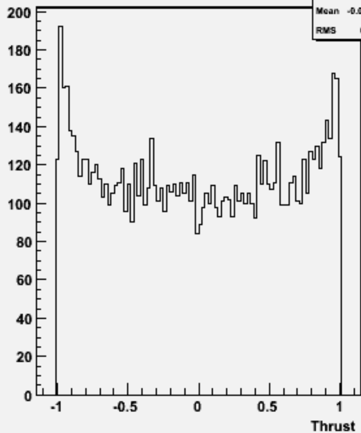
cos \Theta (thrust) w101948 n1n1uue2e2_o
