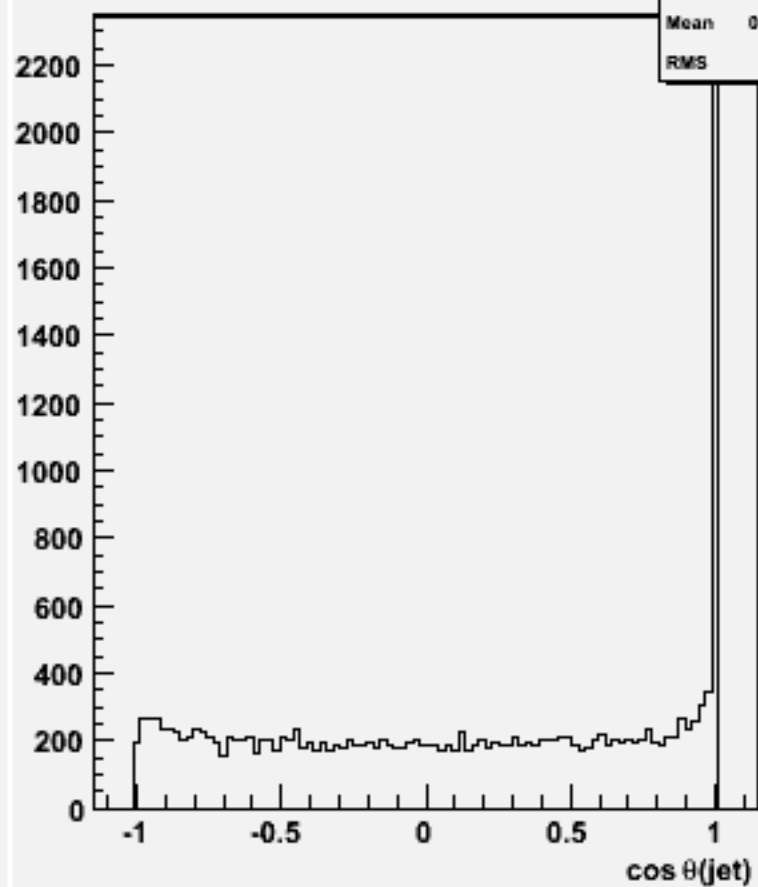
cos \theta for 2-jets :w101948 n1n1uue2e2_o
