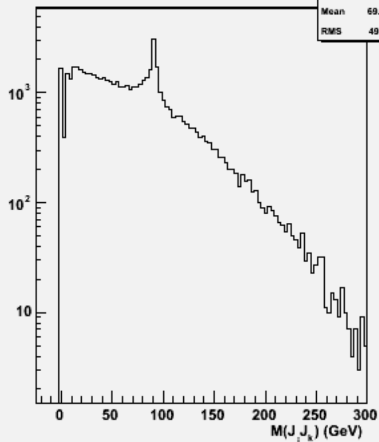
2jets mass(All comb)w101948 n1n1uue2e2_o
