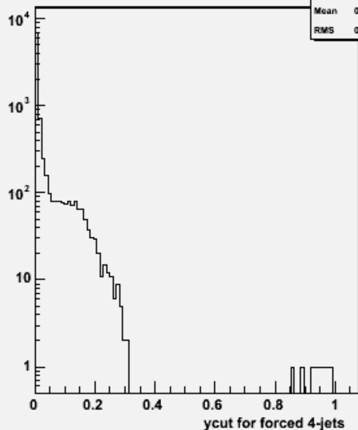
Ycut for 4-jets :w101948 n1n1uue2e2_o
