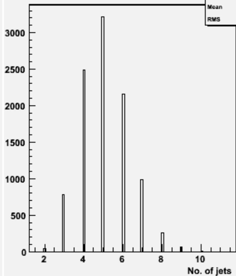
No. jets (ycut=0.001) : w101948 n1n1uue2e2_o
