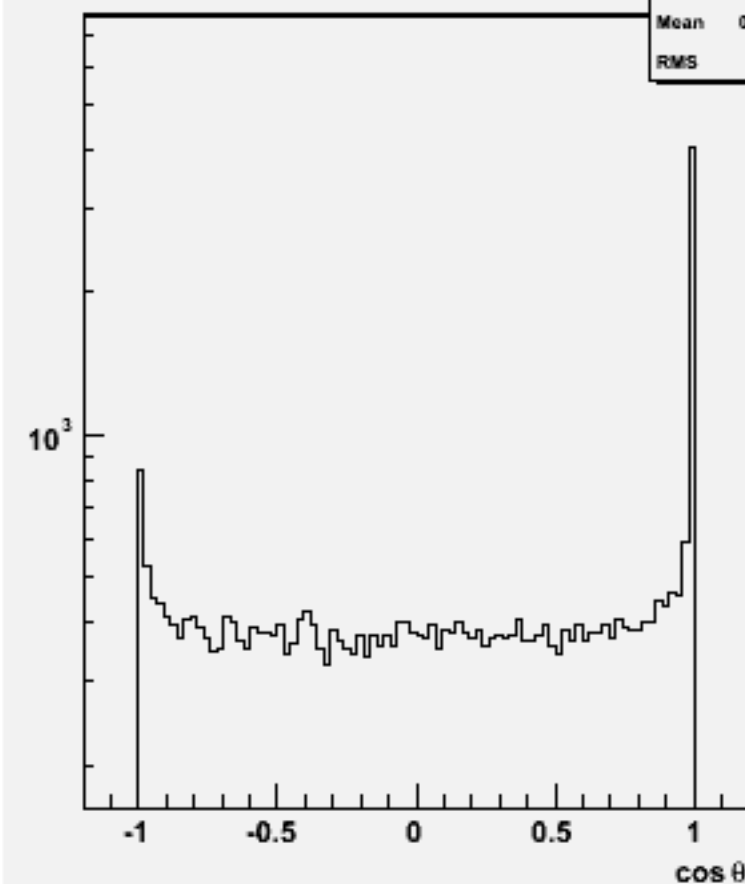
Jet cos \theta (All jets)w101948 n1n1uue2e2_o
