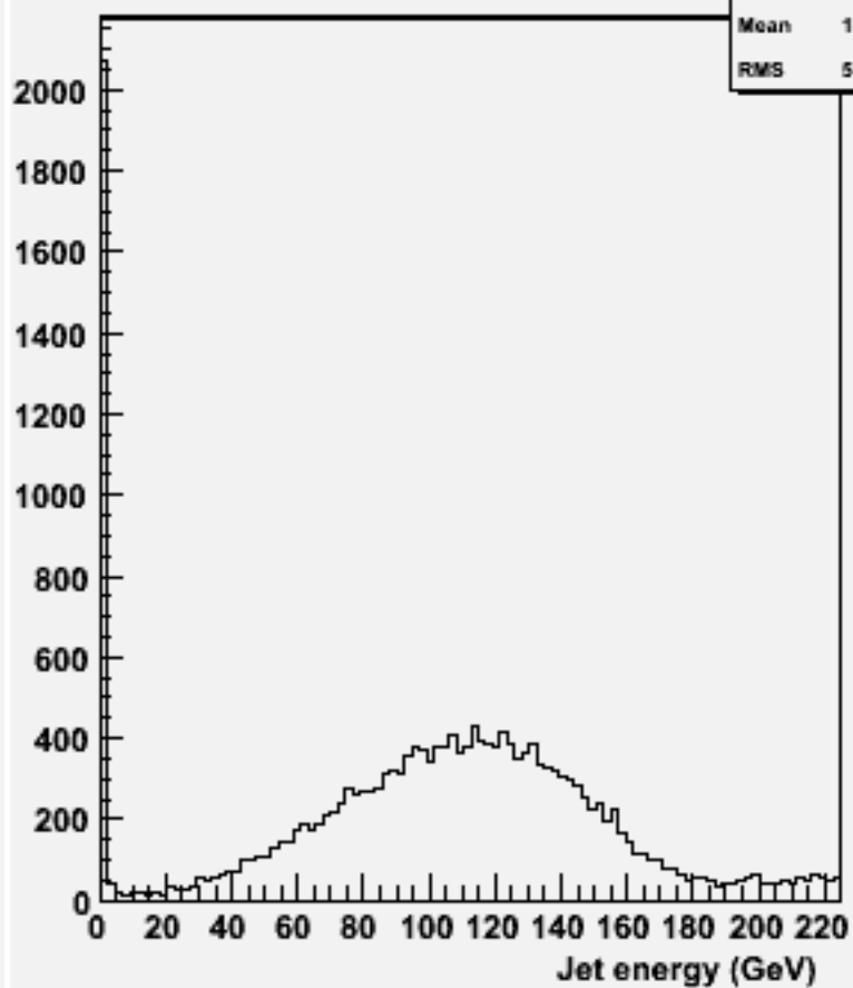
energy for 2-jets :w101948 n1n1uue2e2_o
