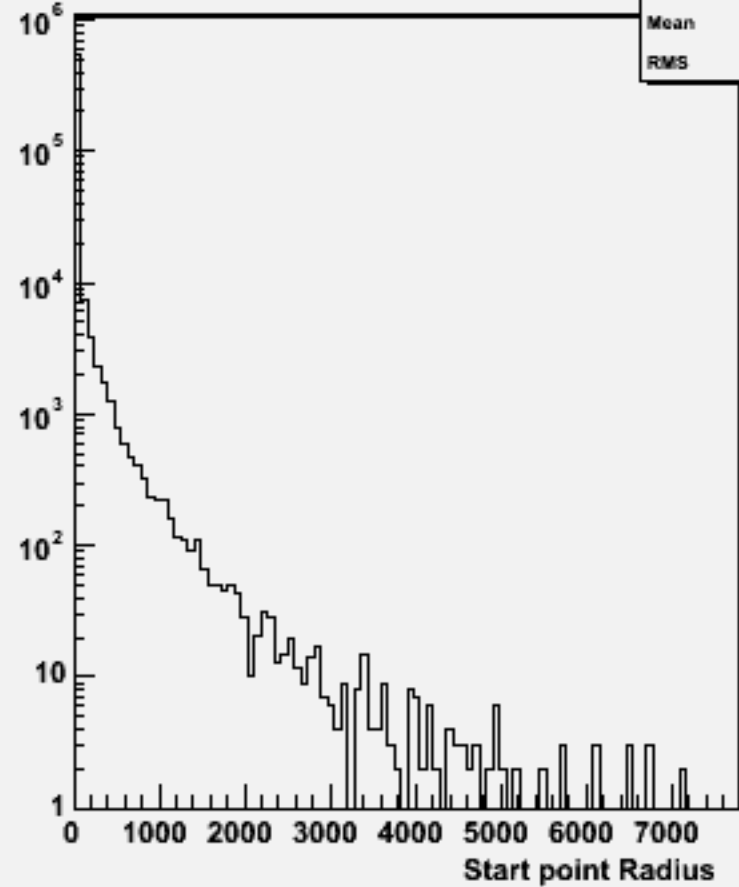
Start point R : w101945 n1n1n3n3bb_o
