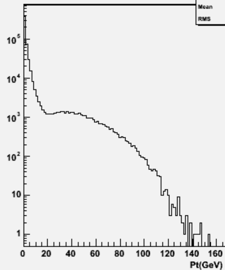
Particle Pt : w101945 n1n1n3n3bb_o
