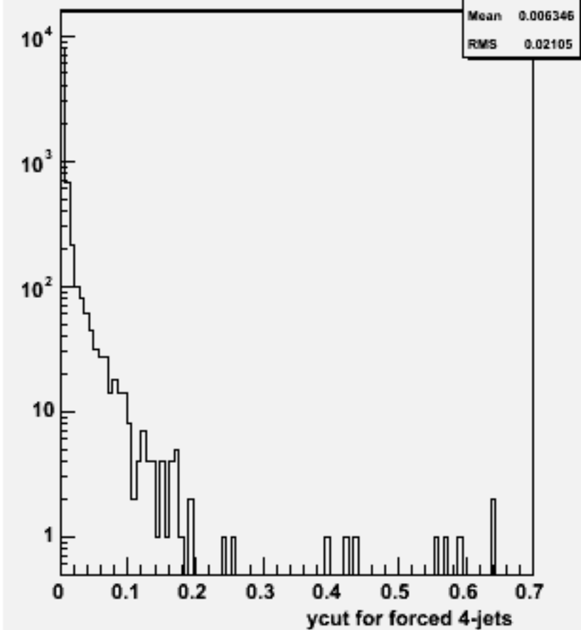
Ycut for 4-jets :w101945 n1n1n3n3bb_o
