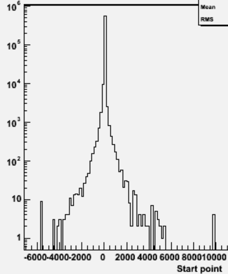
Start point Z : w101945 n1n1n3n3bb_o
