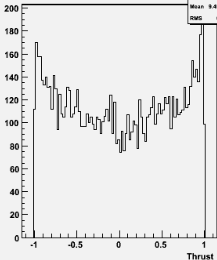
cos \Theta (thrust) w101945 n1n1n3n3bb_o
