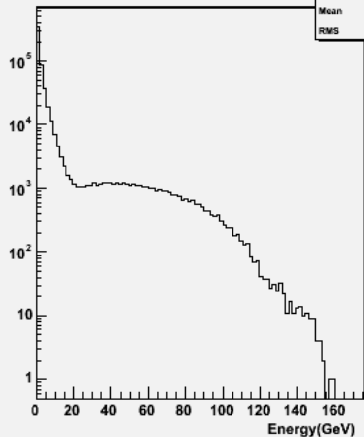
Particle Energy : w101945 n1n1n3n3bb_o
