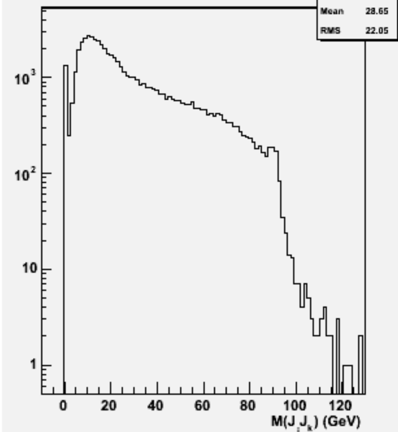
2jets mass(All comb)w101945 n1n1n3n3bb_o
