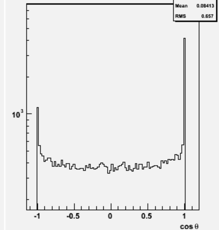
Jet cos \theta (All jets)w101945 n1n1n3n3bb_o
