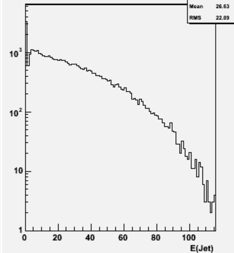
Jet energies(All jets)w101945 n1n1n3n3bb_o
