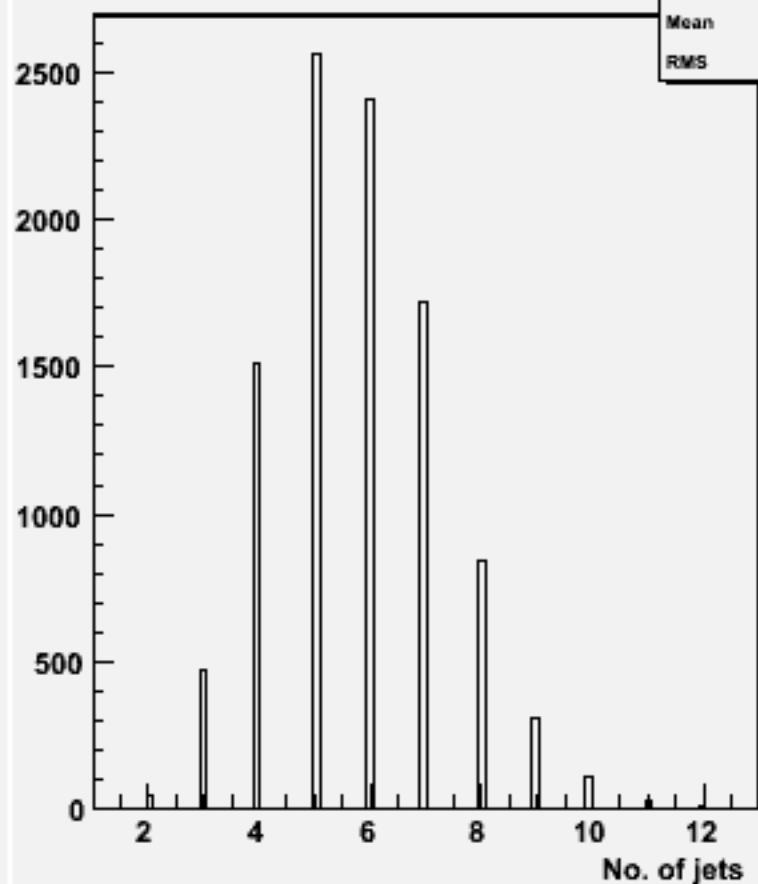
No. jets (ycut=0.001) : w101945 n1n1n3n3bb_o
