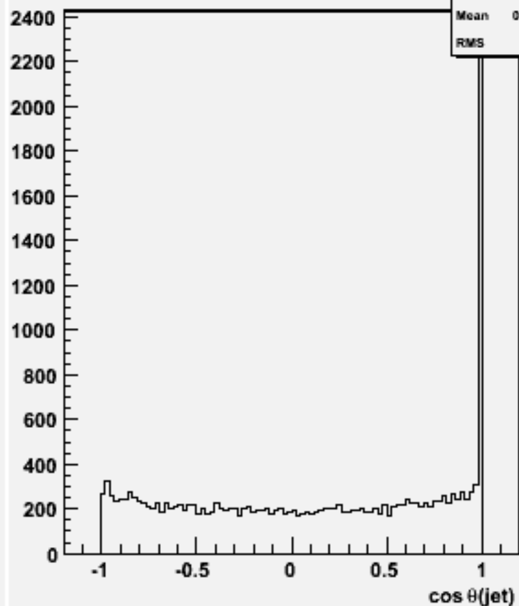
cos \theta for 2-jets :w101945 n1n1n3n3bb_o
