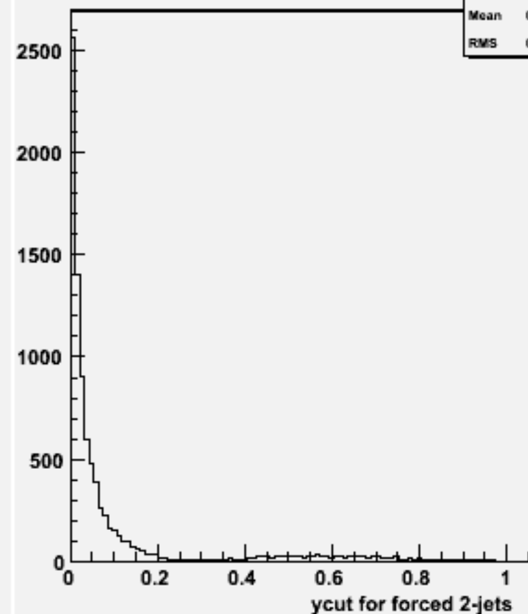
Ycut for 2-jets :w101945 n1n1n3n3bb_o
