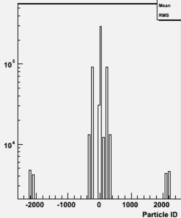
Particle ID : w101945 n1n1n3n3bb_o
