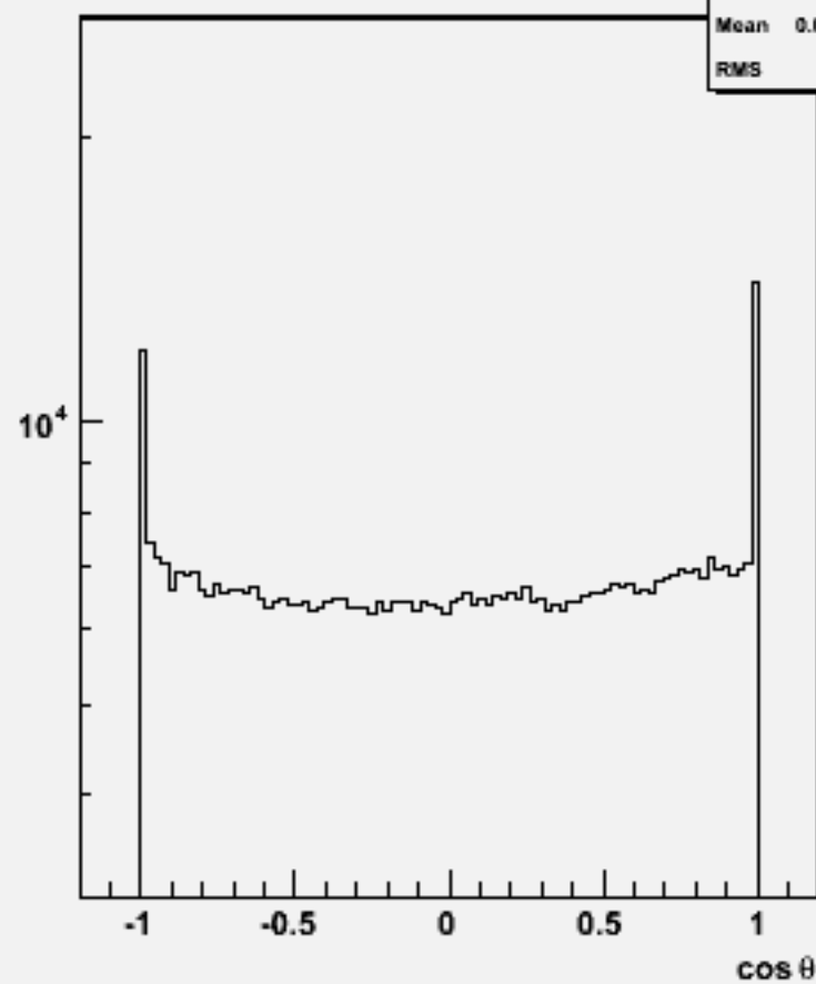
Particle cosθ : w101945 n1n1n3n3bb_o
