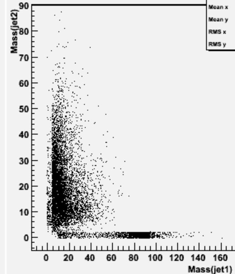
Jet mass for forced 2-jets : w101945 n1n1n3n3bb_o
