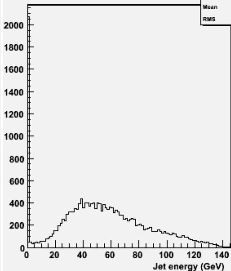
energy for 2-jets :w101945 n1n1n3n3bb_o
