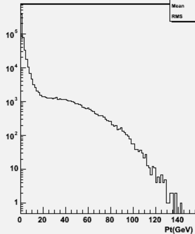
Particle Pt : w101944 n1n1n3n3bb_o
