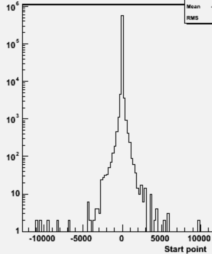
Start point Z : w101944 n1n1n3n3bb_o
