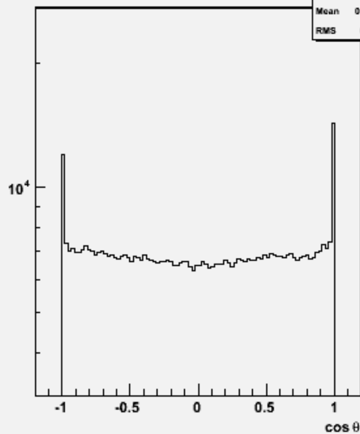
Particle cosθ : w101944 n1n1n3n3bb_o
