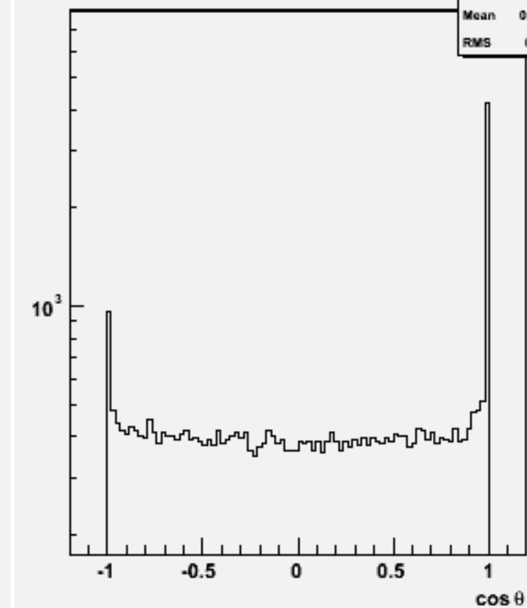
Jet cos \theta (All jets)w101944 n1n1n3n3bb_o
