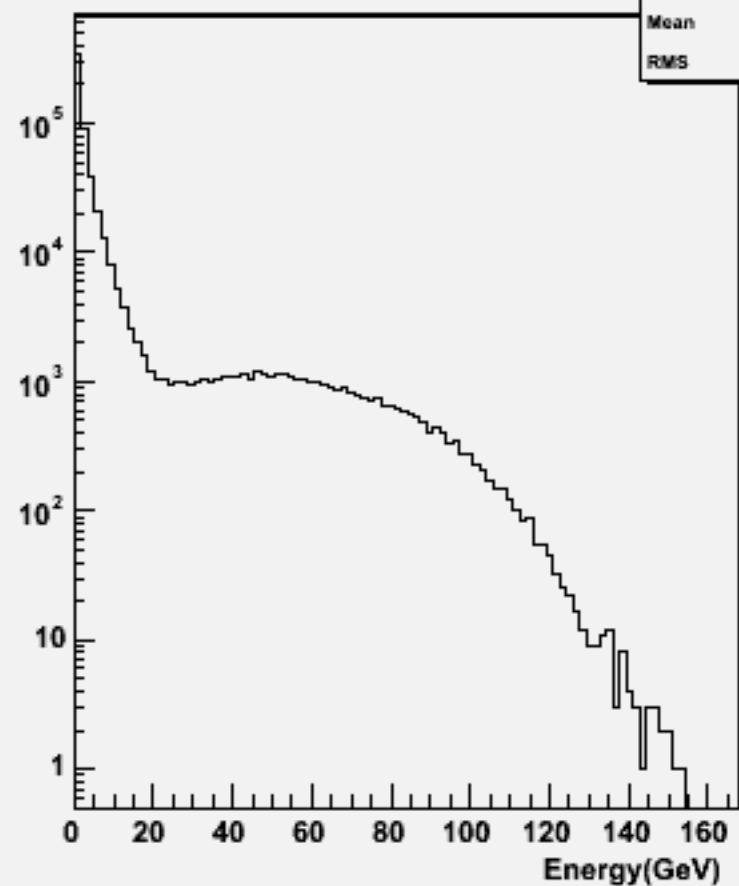
Particle Energy : w101944 n1n1n3n3bb_o
