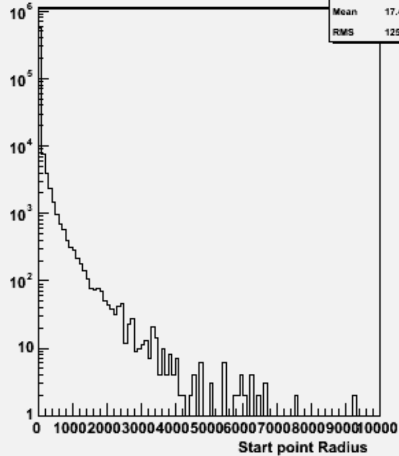
Start point R : w101944 n1n1n3n3bb_o
