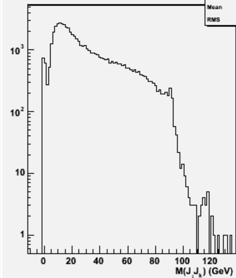
2jets mass(All comb)w101944 n1n1n3n3bb_o
