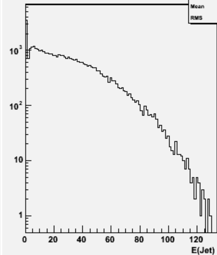
Jet energies(All jets)w101944 n1n1n3n3bb_o
