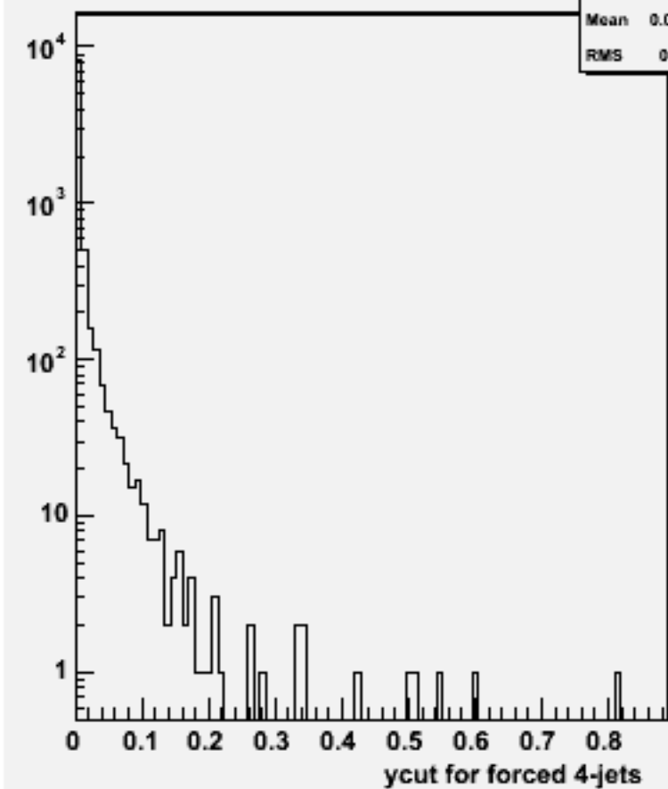
Ycut for 4-jets :w101944 n1n1n3n3bb_o
