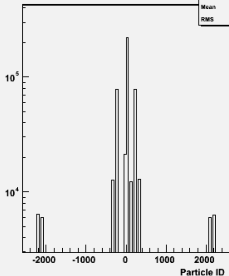
Particle ID : w101940 n1n1n3n3ss_o
