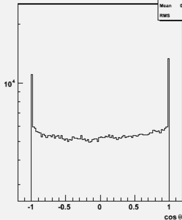
Particle cosθ : w101940 n1n1n3n3ss_o
