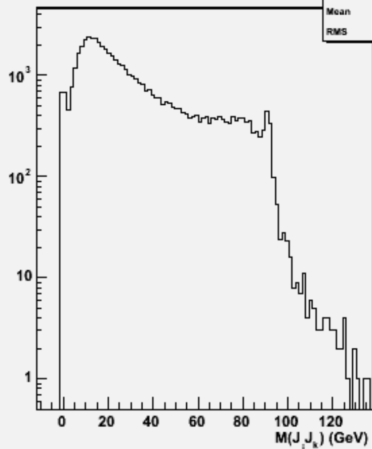
2jets mass(All comb)w101940 n1n1n3n3ss_o
