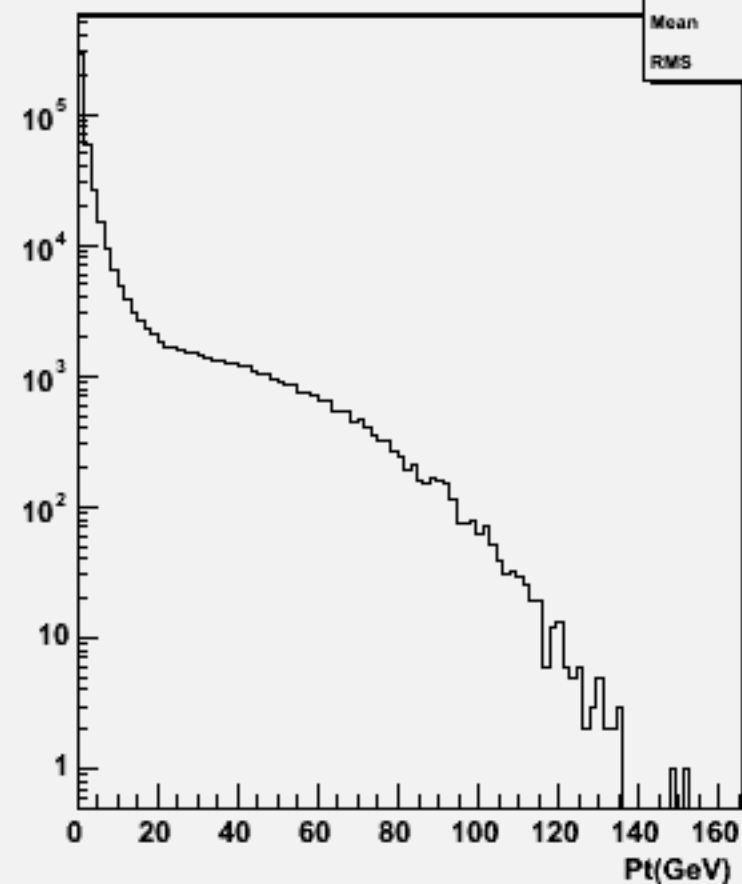
Particle Pt : w101940 n1n1n3n3ss_o
