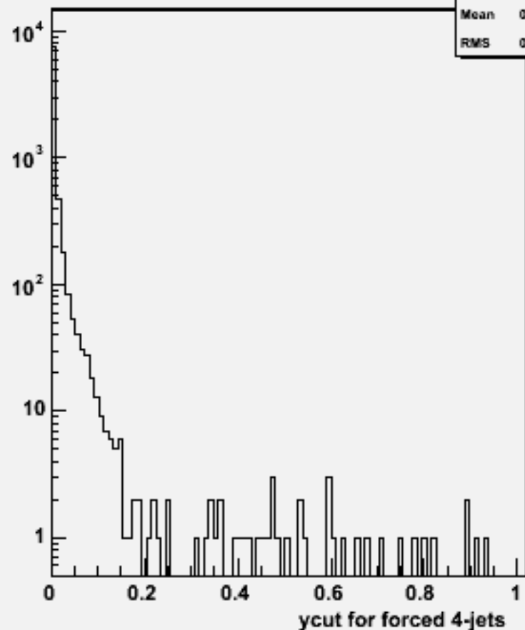
Ycut for 4-jets :w101940 n1n1n3n3ss_o
