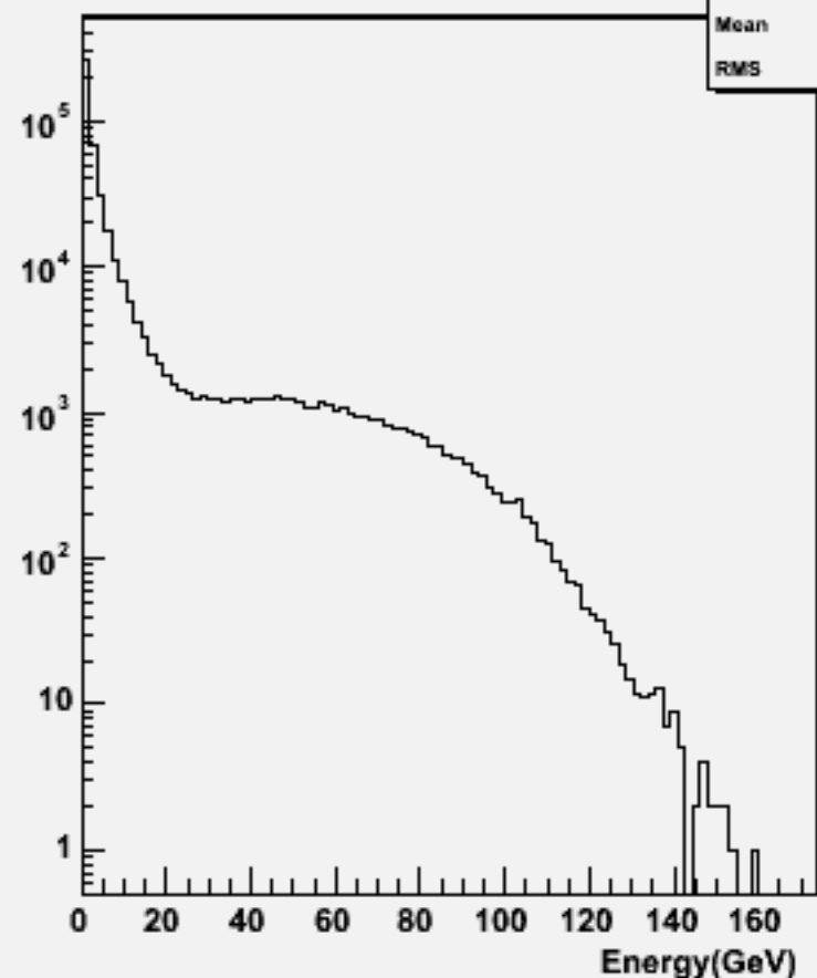
Particle Energy : w101940 n1n1n3n3ss_o
