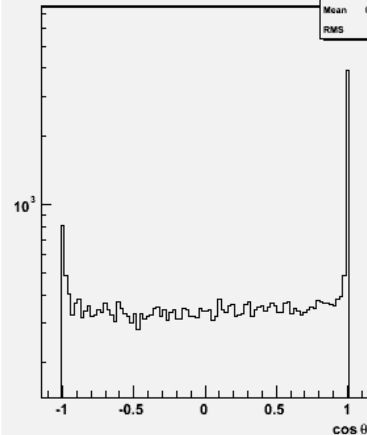
Jet cos \theta (All jets)w101940 n1n1n3n3ss_o
