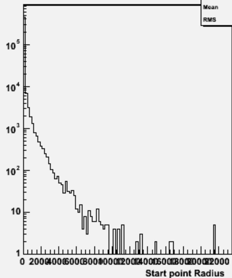
Start point R : w101940 n1n1n3n3ss_o
