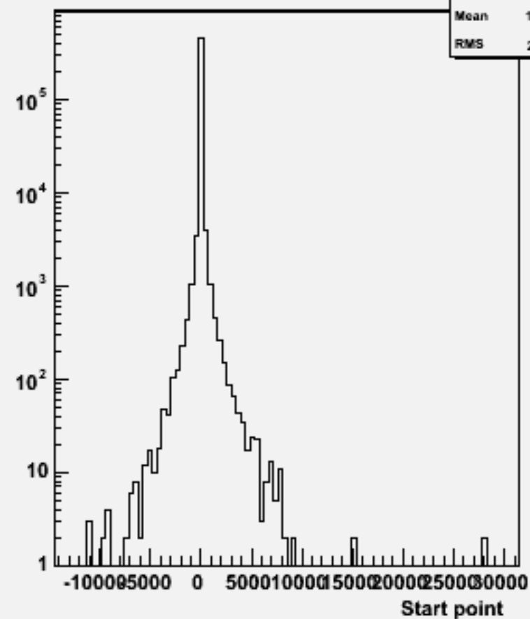
Start point Z : w101940 n1n1n3n3ss_o
