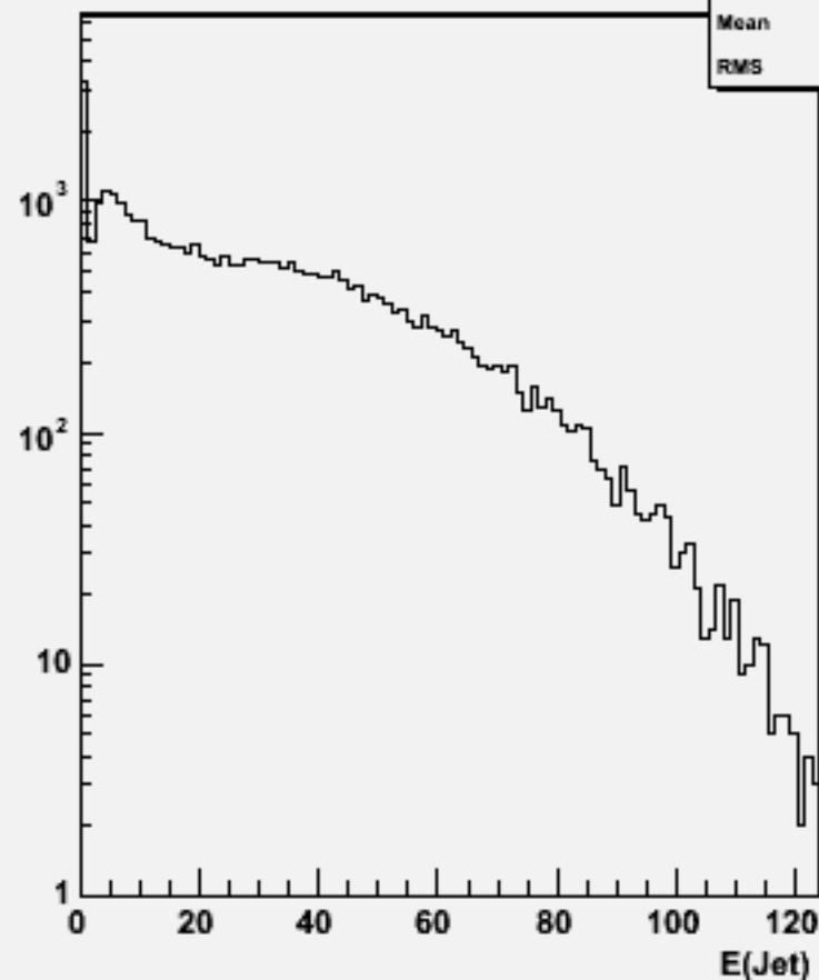
Jet energies(All jets)w101940 n1n1n3n3ss_o
