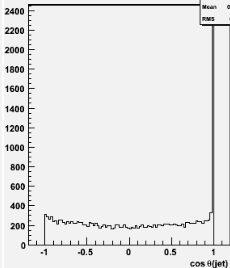
cos \theta for 2-jets :w101937 n1n1n3n3dd_o
