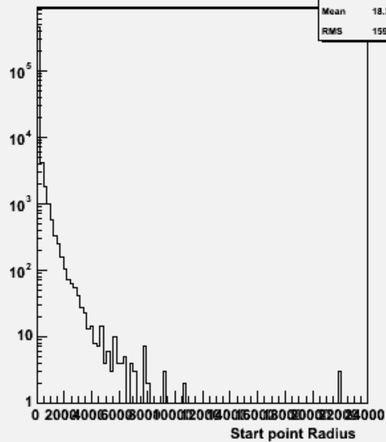
Start point R : w101937 n1n1n3n3dd_o
