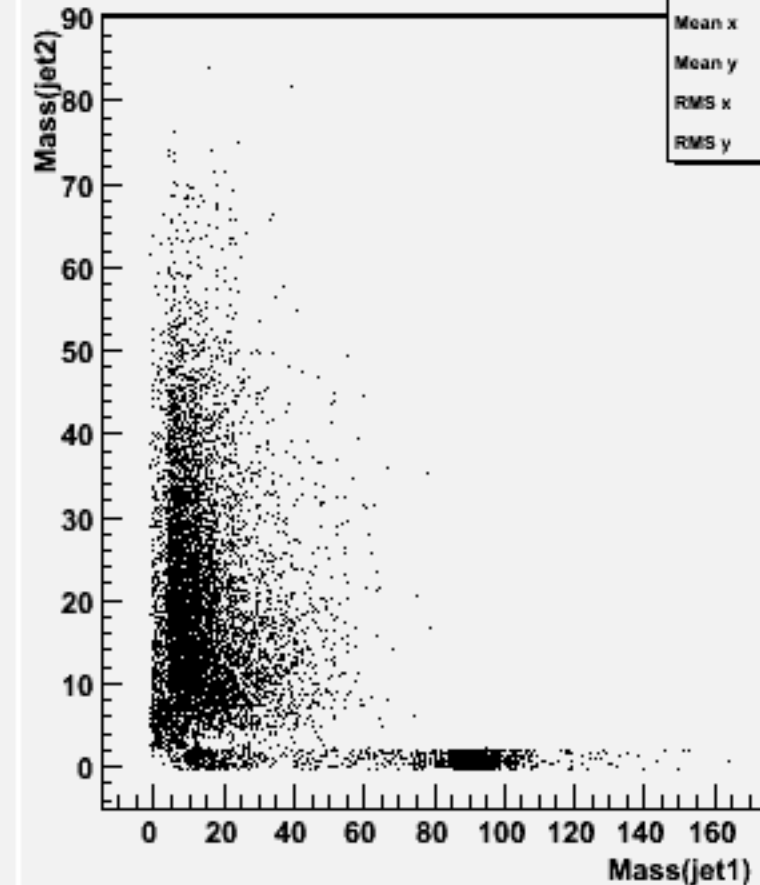
Jet mass for forced 2-jets : w101937 n1n1n3n3dd_o
