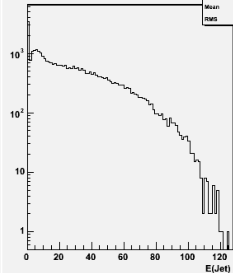
Jet energies(All jets)w101937 n1n1n3n3dd_o
