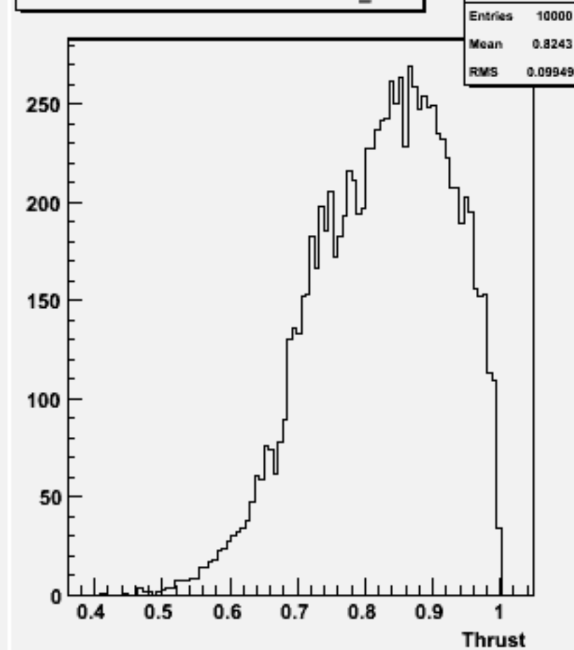
Thrust w101937 n1n1n3n3dd_o
