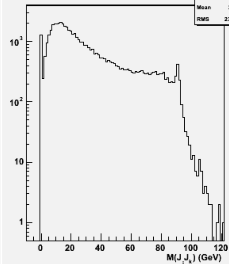
2jets mass(All comb)w101937 n1n1n3n3dd_o
