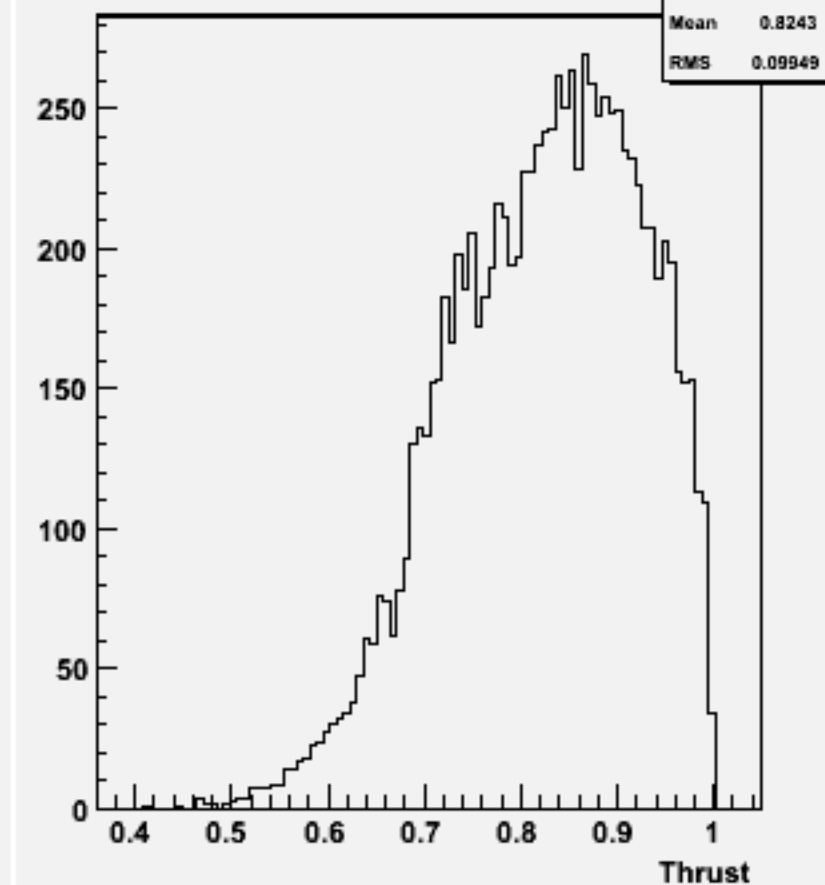
Thrust w101937 n1n1n3n3dd_o
