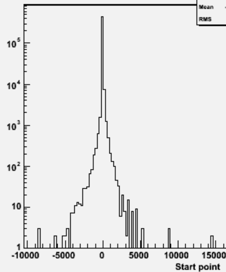
Start point Z : w101937 n1n1n3n3dd_o
