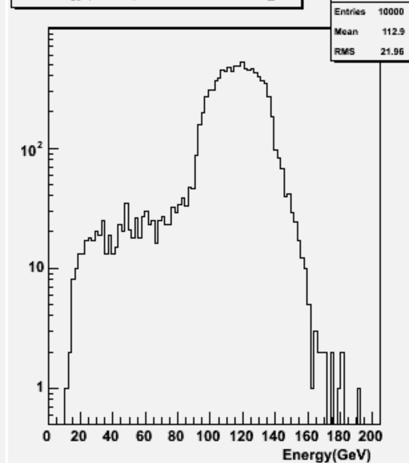
Total Energy (w/o \nu ): w101937 n1n1n3n3dd_o
