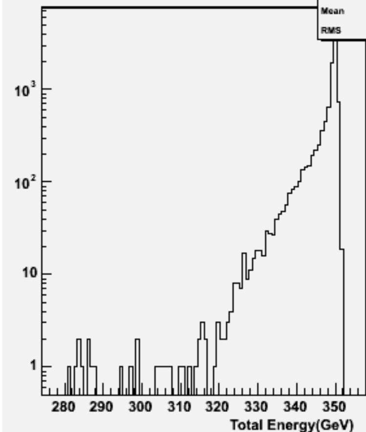
Pt Sum: w101937 n1n1n3n3dd_o
