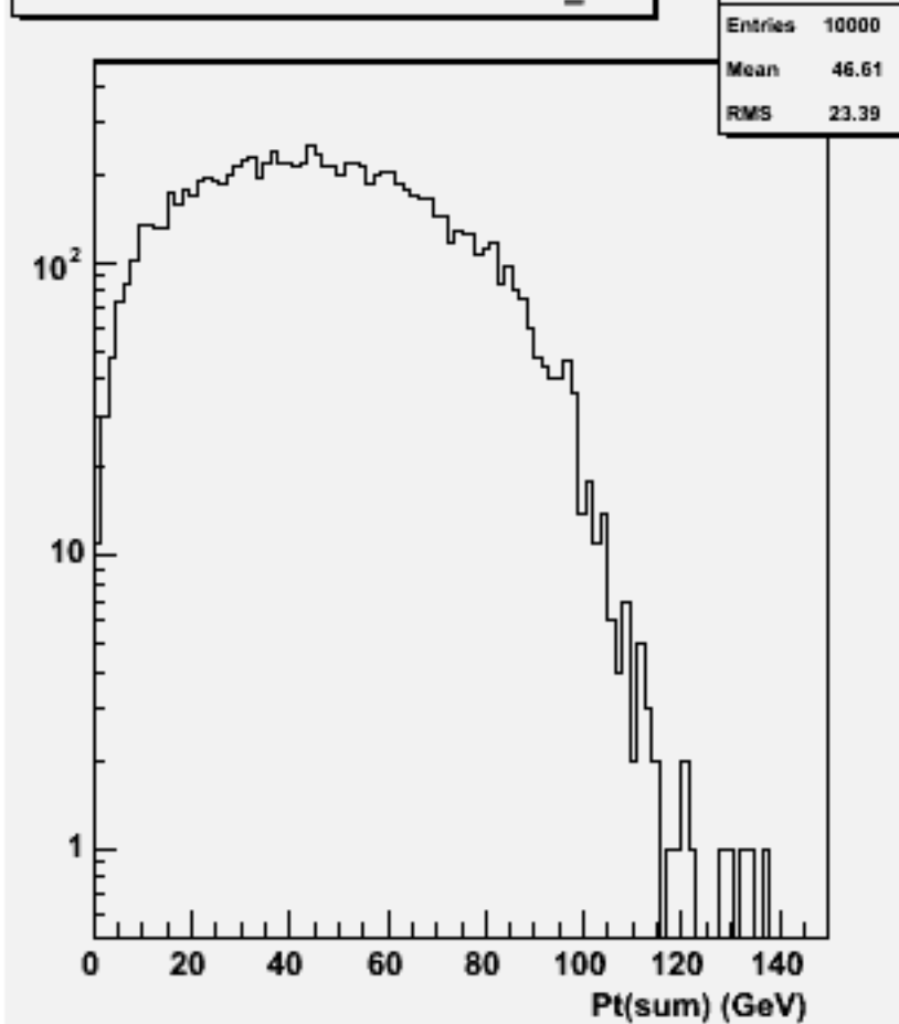
Pt Sum: w101937 n1n1n3n3dd_o
