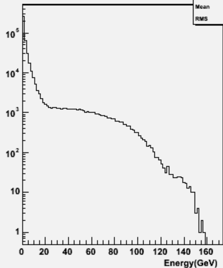
Particle Energy : w101937 n1n1n3n3dd_o
