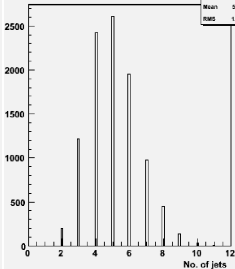
No. jets (ycut=0.001) : w101937 n1n1n3n3dd_o
