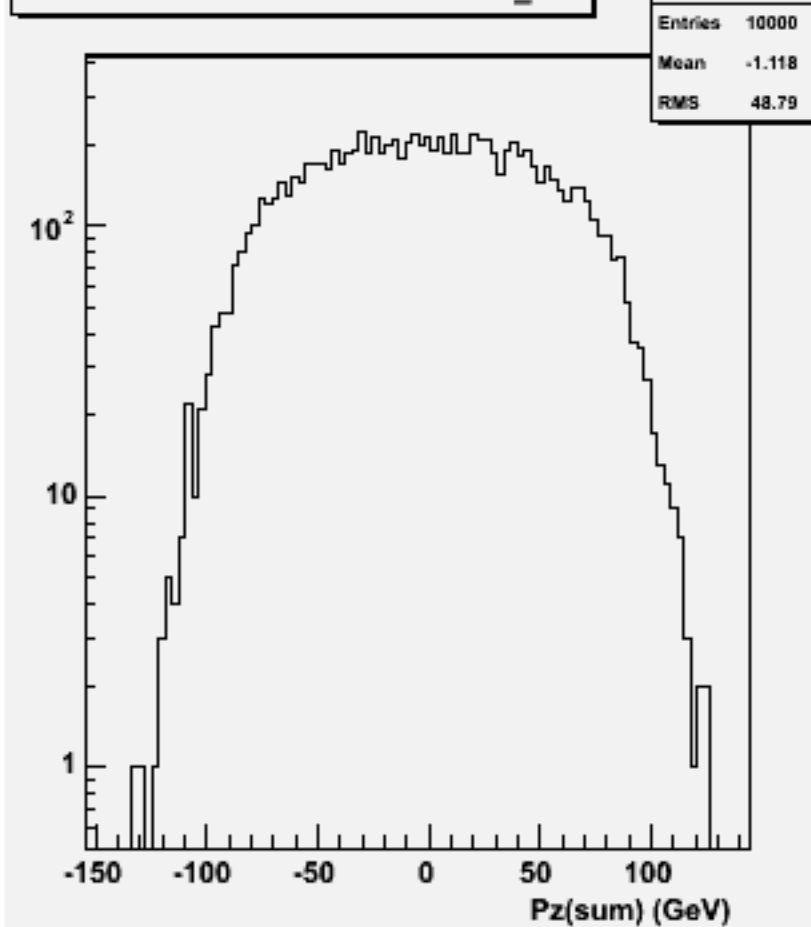
Pz Sum: w101937 n1n1n3n3dd_o
