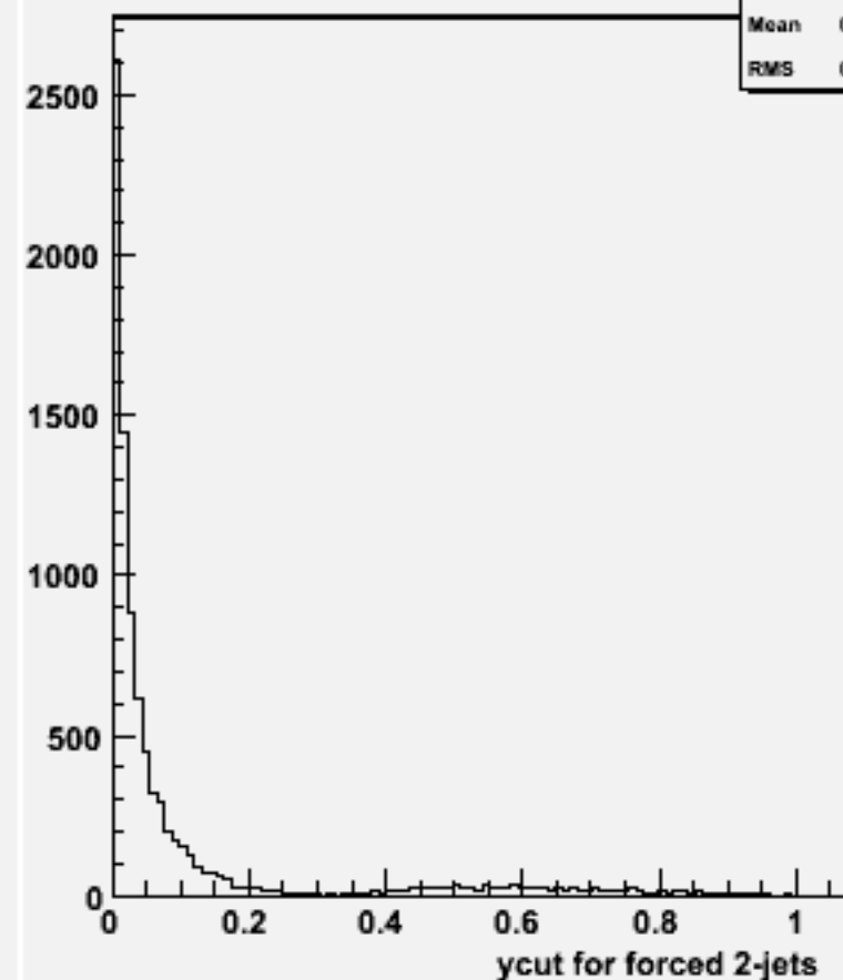
Ycut for 2-jets :w101937 n1n1n3n3dd_o
