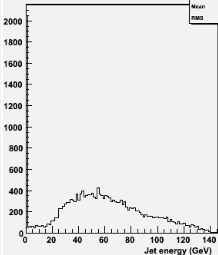
energy for 2-jets :w101937 n1n1n3n3dd_o
