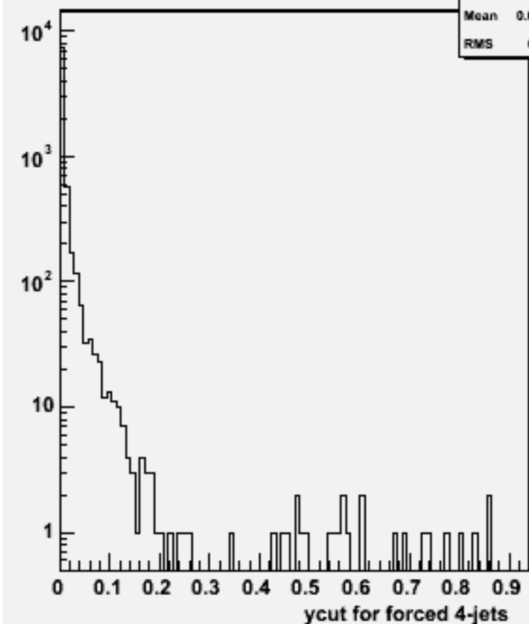
Ycut for 4-jets :w101937 n1n1n3n3dd_o
