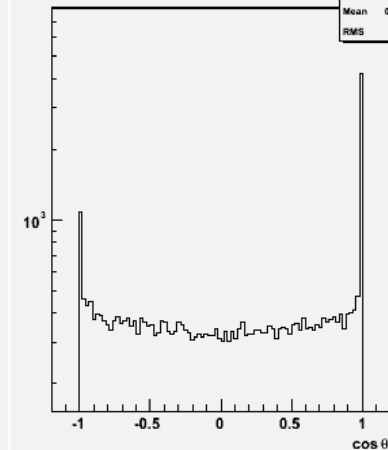
Jet cos \theta (All jets)w101937 n1n1n3n3dd_o
