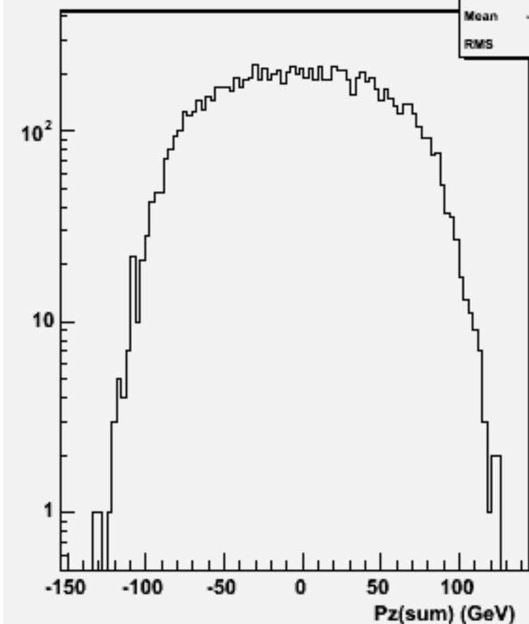
Pz Sum: w101937 n1n1n3n3dd_o
