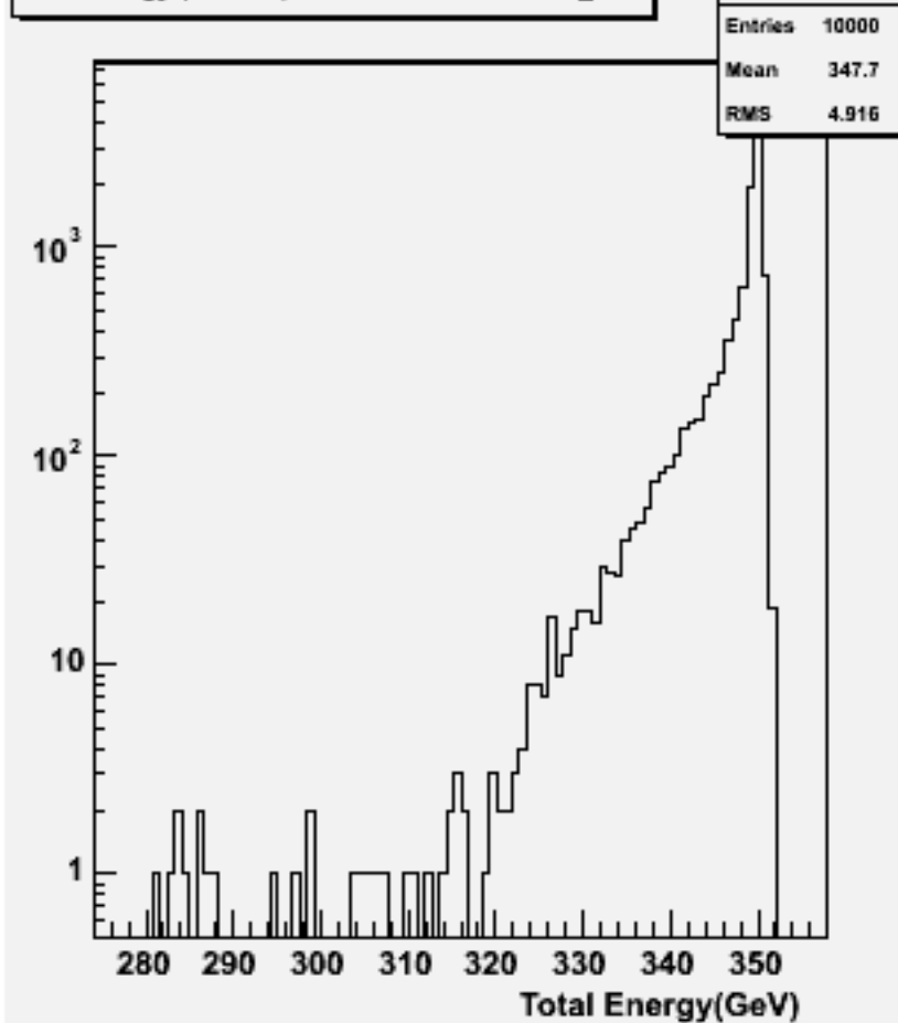
Total Energy (inc. \nu ): w101937 n1n1n3n3dd_o
