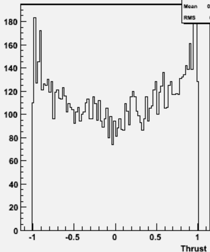
cos \Theta (thrust) w101937 n1n1n3n3dd_o
