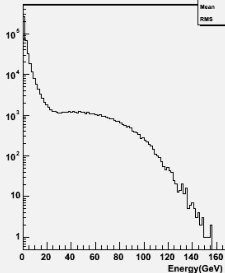
Particle Energy : w101936 n1n1n3n3dd_o
