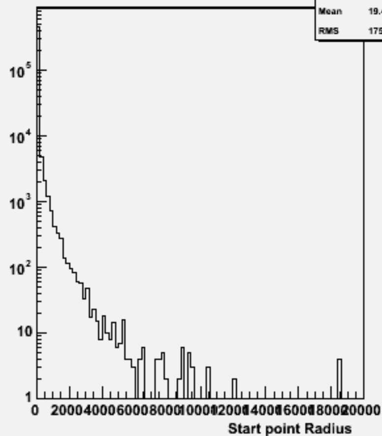
Start point R : w101936 n1n1n3n3dd_o
