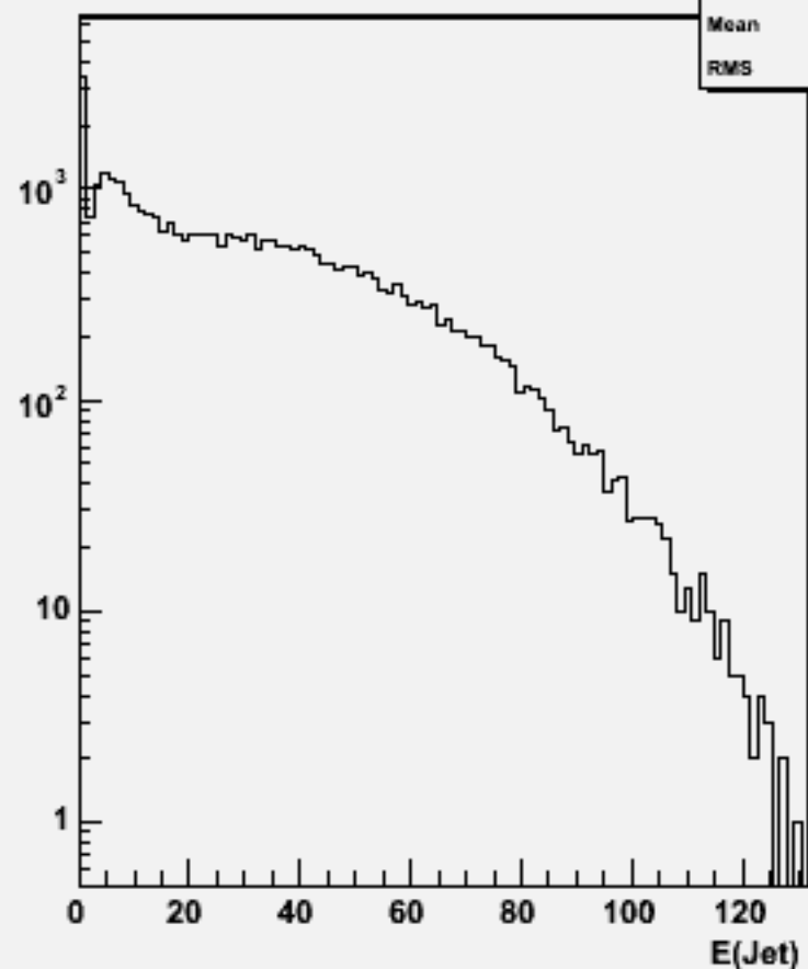
Jet energies(All jets)w101936 n1n1n3n3dd_o
