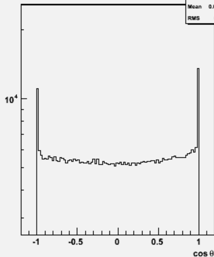
Particle cosθ : w101936 n1n1n3n3dd_o
