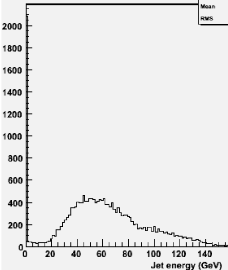
energy for 2-jets :w101936 n1n1n3n3dd_o
