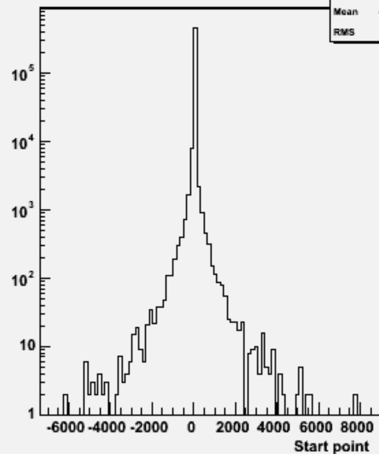
Start point Z : w101936 n1n1n3n3dd_o
