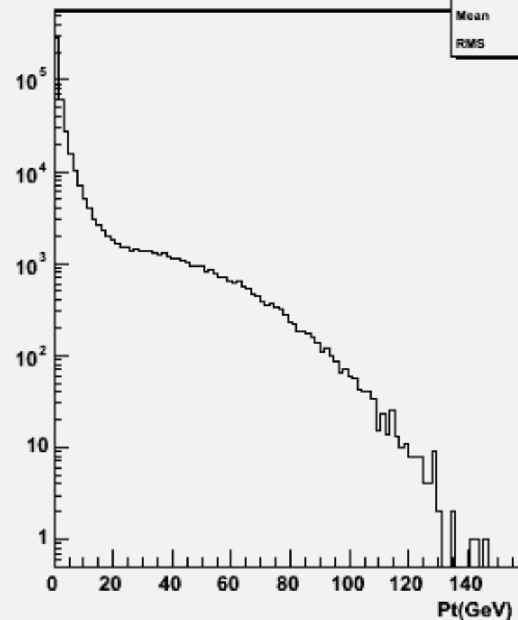
Particle Pt : w101936 n1n1n3n3dd_o
