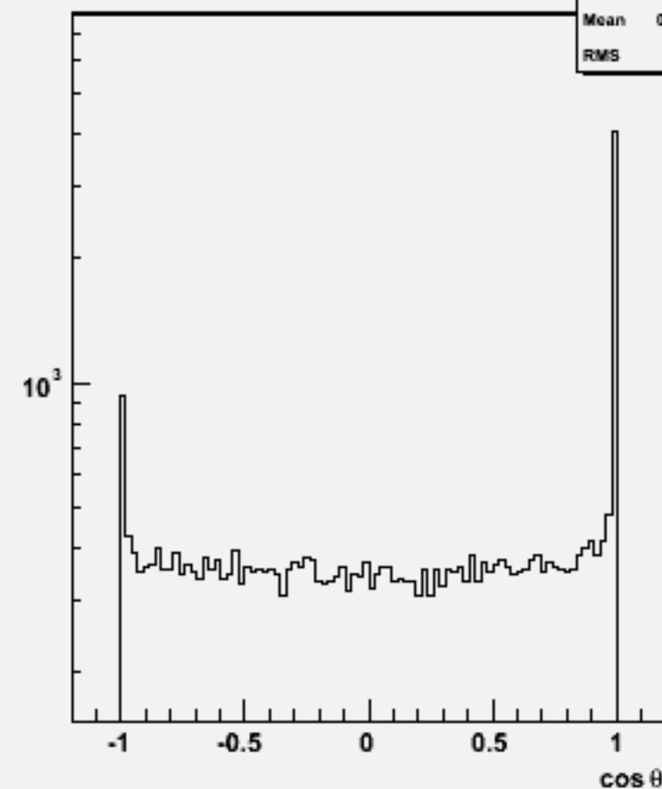
Jet cos \theta (All jets)w101936 n1n1n3n3dd_o
