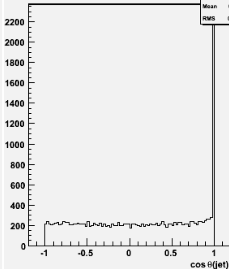
cos \theta for 2-jets :w101936 n1n1n3n3dd_o
