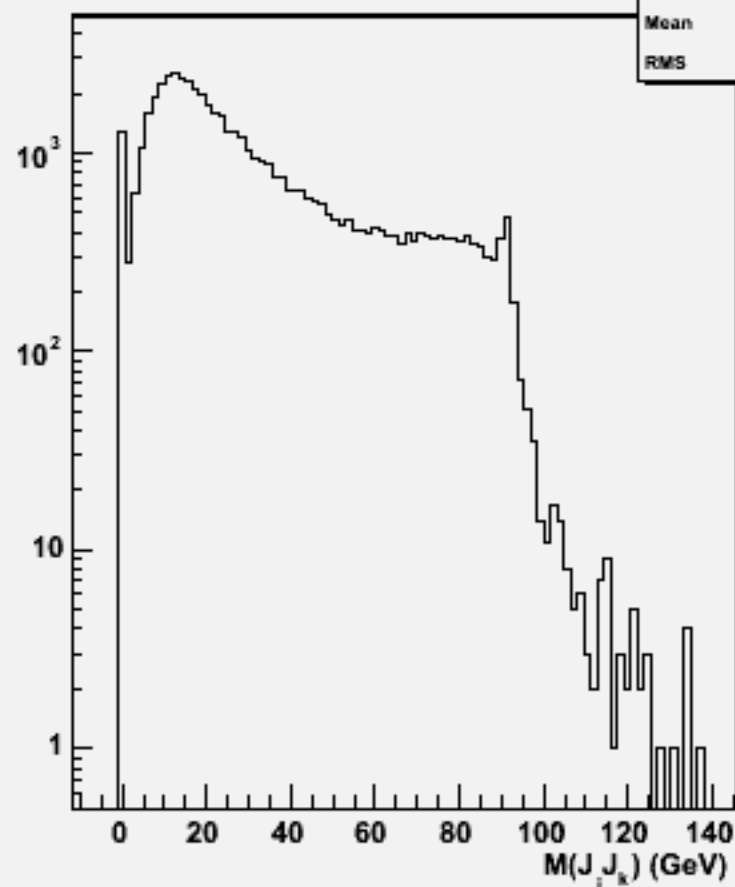
2jets mass(All comb)w101936 n1n1n3n3dd_o
