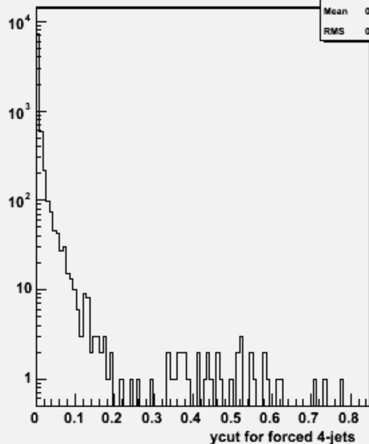
Ycut for 4-jets :w101936 n1n1n3n3dd_o
