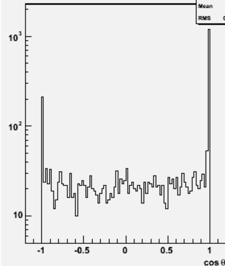
Jet cos \theta (All jets)w101932 n1n1n3n3e2e2_o
