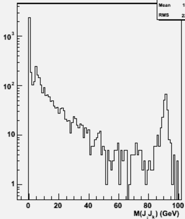
2jets mass(All comb)w101932 n1n1n3n3e2e2_o
