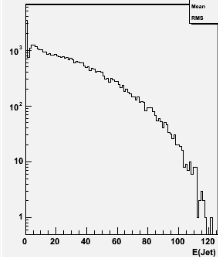
Jet energies(All jets)w101929 n1n1n2n2bb_o
