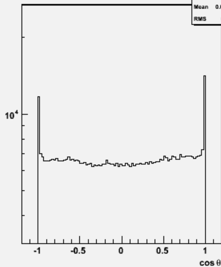
Particle cos \theta : w101929 n1n1n2n2bb_o
