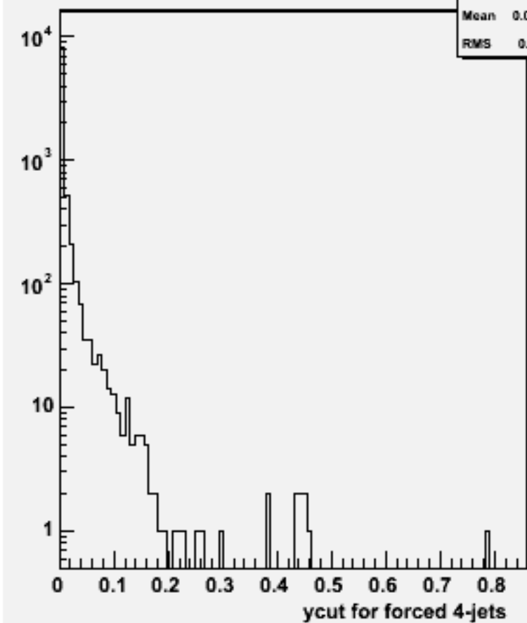
Ycut for 4-jets :w101929 n1n1n2n2bb_o
