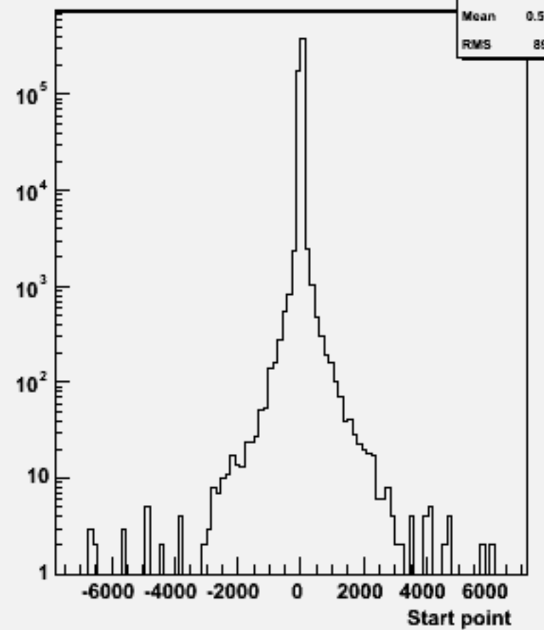
Start point Z : w101929 n1n1n2n2bb_o
