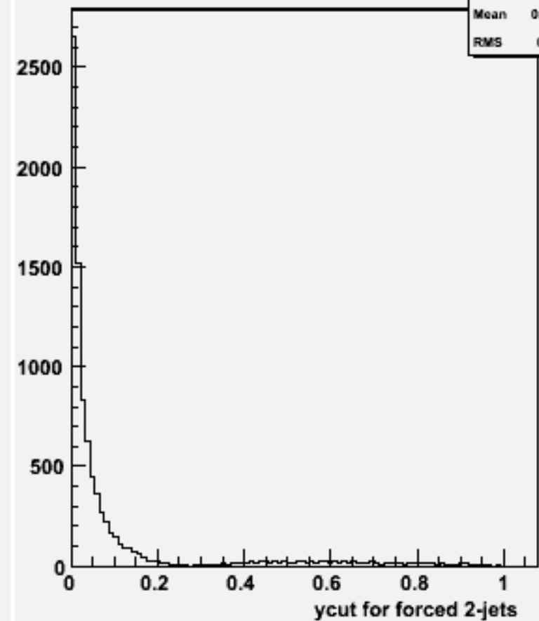
Ycut for 2-jets :w101929 n1n1n2n2bb_o
