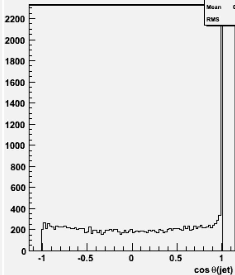
cos \theta for 2-jets :w101929 n1n1n2n2bb_o
