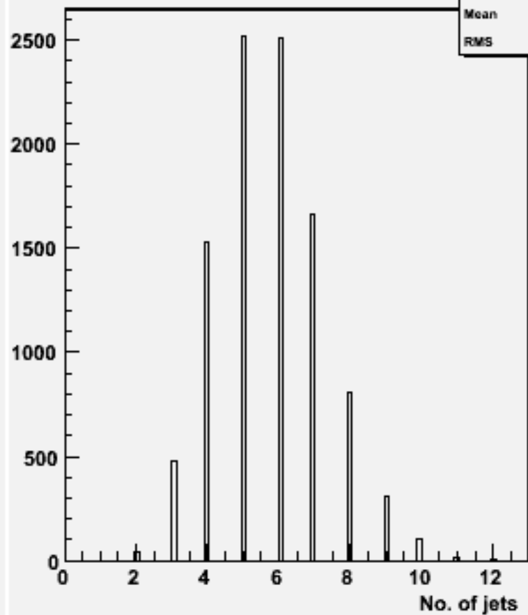
No. jets (ycut=0.001) : w101929 n1n1n2n2bb_o
