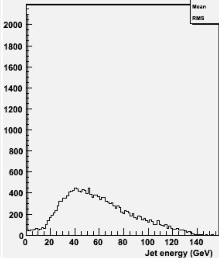
energy for 2-jets :w101929 n1n1n2n2bb_o
