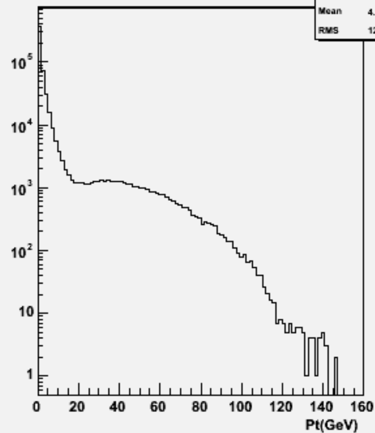
Particle Pt : w101929 n1n1n2n2bb_o
