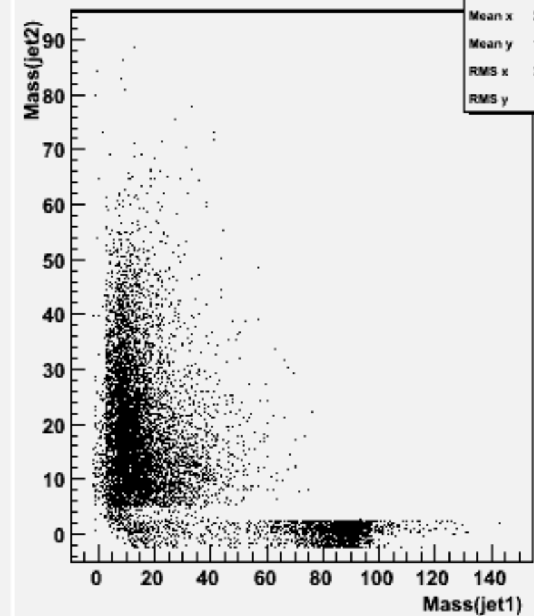
Jet mass for forced 2-jets : w101929 n1n1n2n2bb_o
