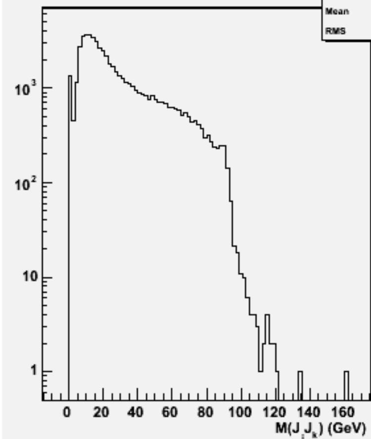
2jets mass(All comb)w101929 n1n1n2n2bb_o
