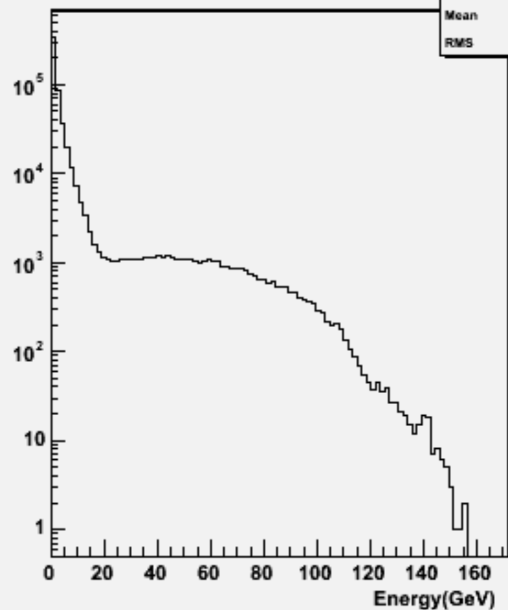
Particle Energy : w101929 n1n1n2n2bb_o
