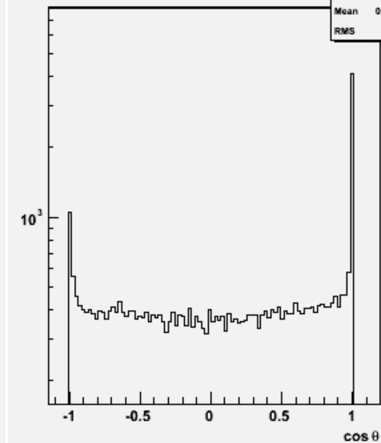
Jet cos \theta (All jets)w101929 n1n1n2n2bb_o
