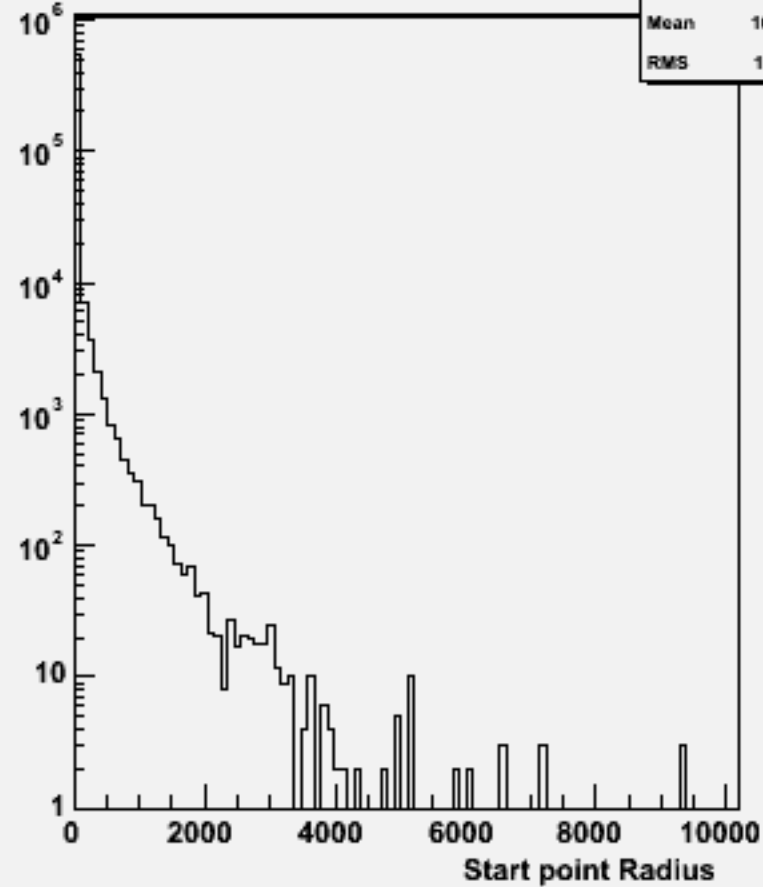
Start point R : w101929 n1n1n2n2bb_o
