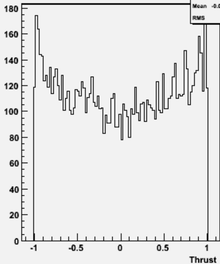
cos \Theta (thrust) w101929 n1n1n2n2bb_o
