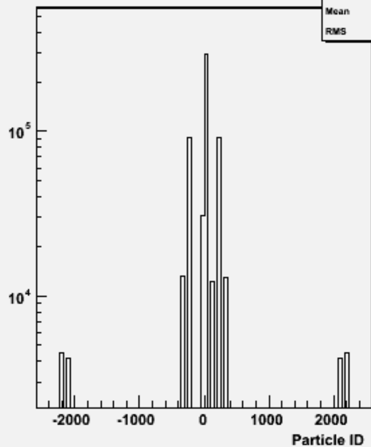
Particle ID : w101929 n1n1n2n2bb_o
